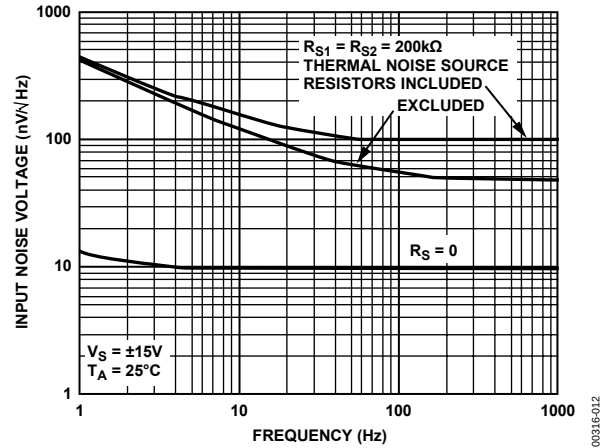
Figure 12. Total Input Noise Voltage vs. Frequency
