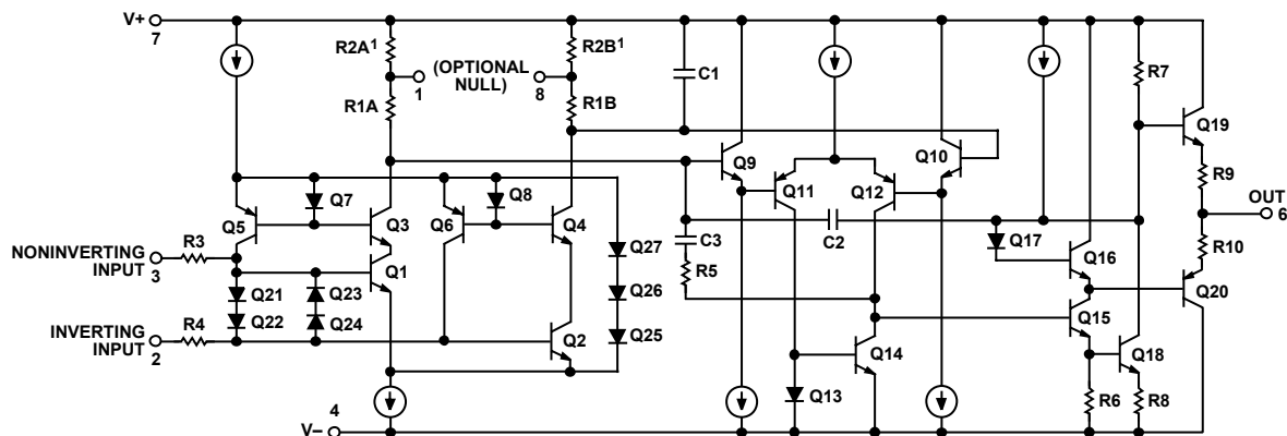
Figure 2. Simplified Schematic
