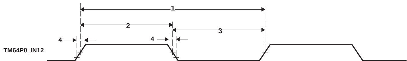
Figure 6-57. Timer Timing
