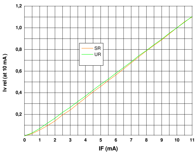
I_F - I_{v, \text{rel}} characteristic
