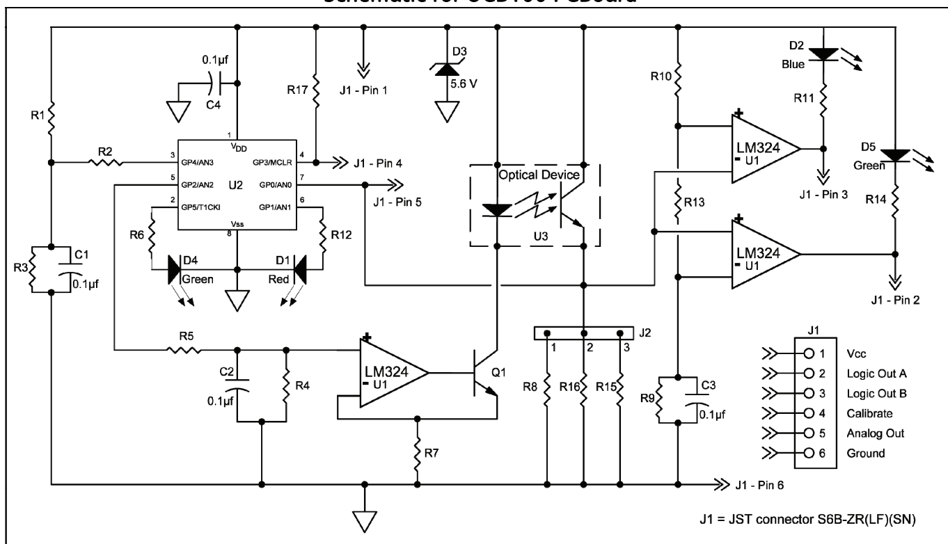
Schematic for OCB100 PCBoard
