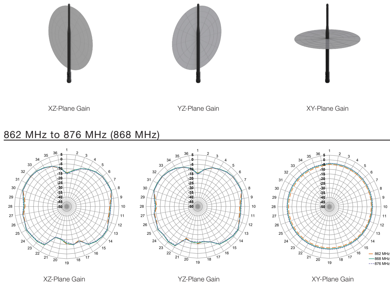
Figure 8. ANT-868-OC-LG Radiation Patterns
