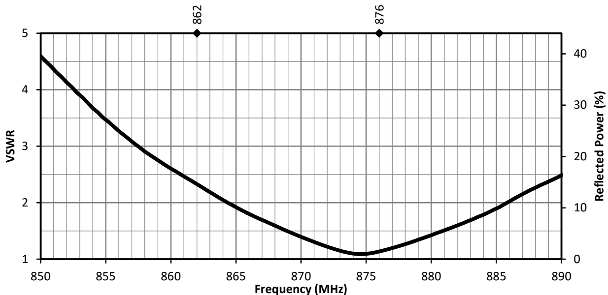
Figure 3. ANT-868-OC-LG VSWR
