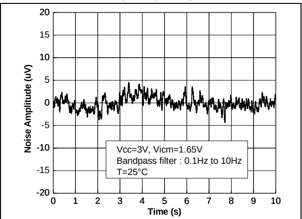
Figure 35. Noise amplitude on 0.1 to 10 Hz frequency range
