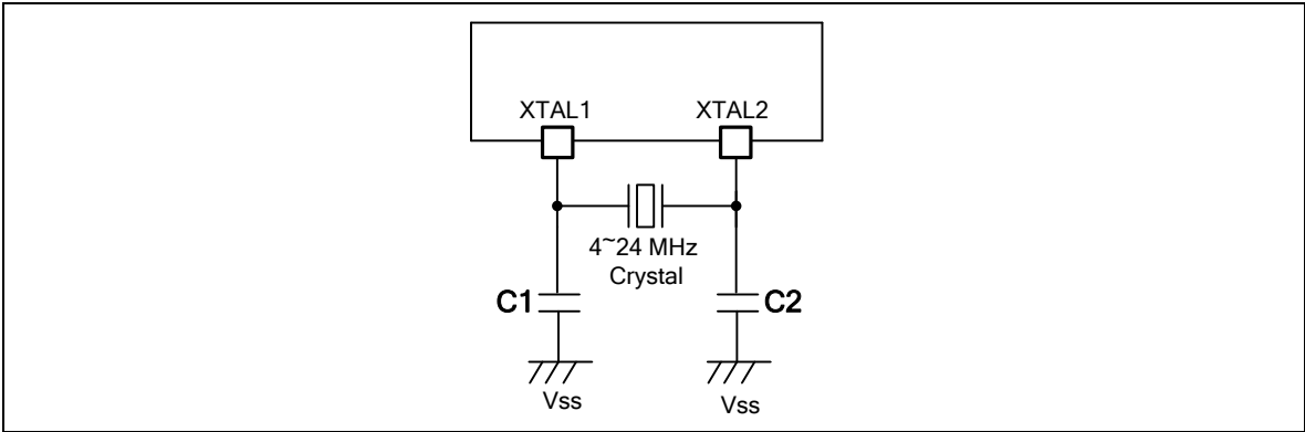
Figure 8-1Mini5xDE Typical Crystal Application Circuit
