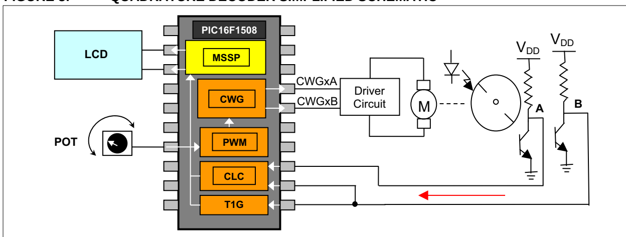
FIGURE 3: QUADRATURE DECODER SIMPLIFIED SCHEMATIC
