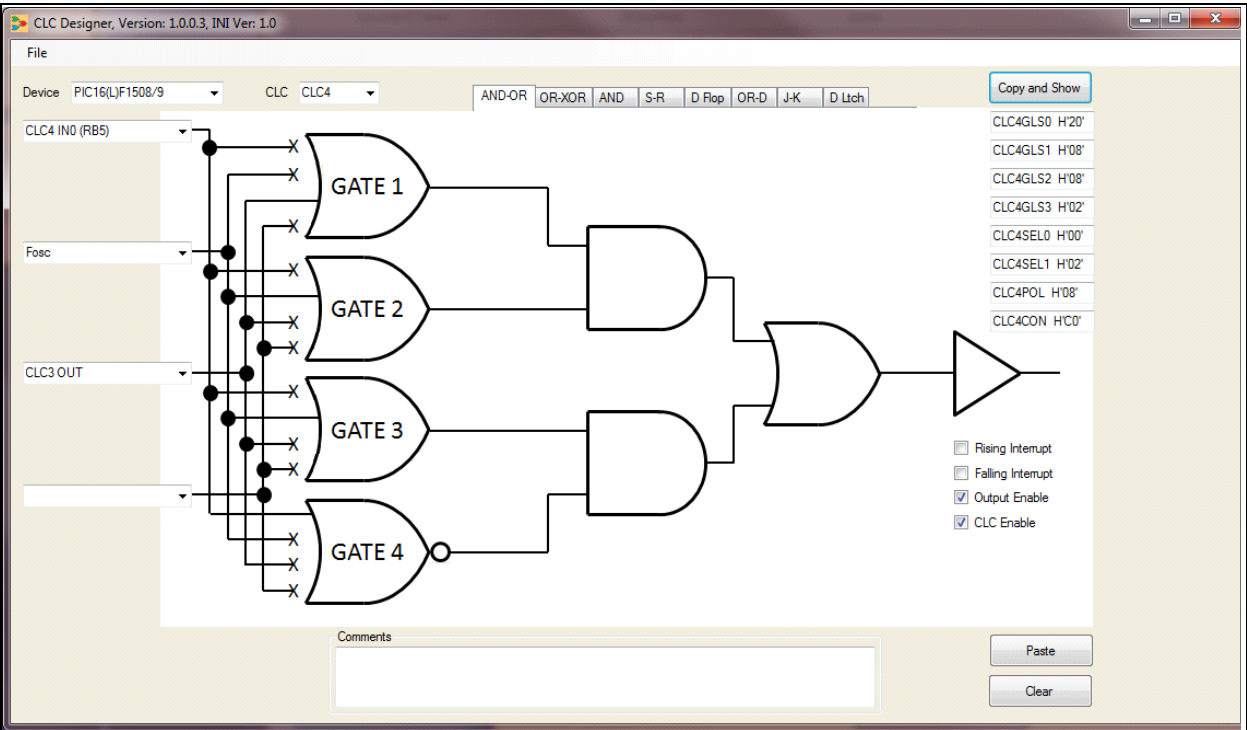
FIGURE 8: CLC4 SETUP
