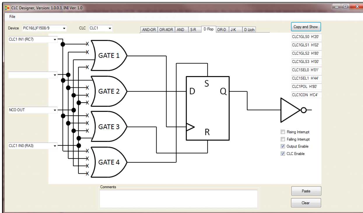
FIGURE 5: CLC1 SETUP
