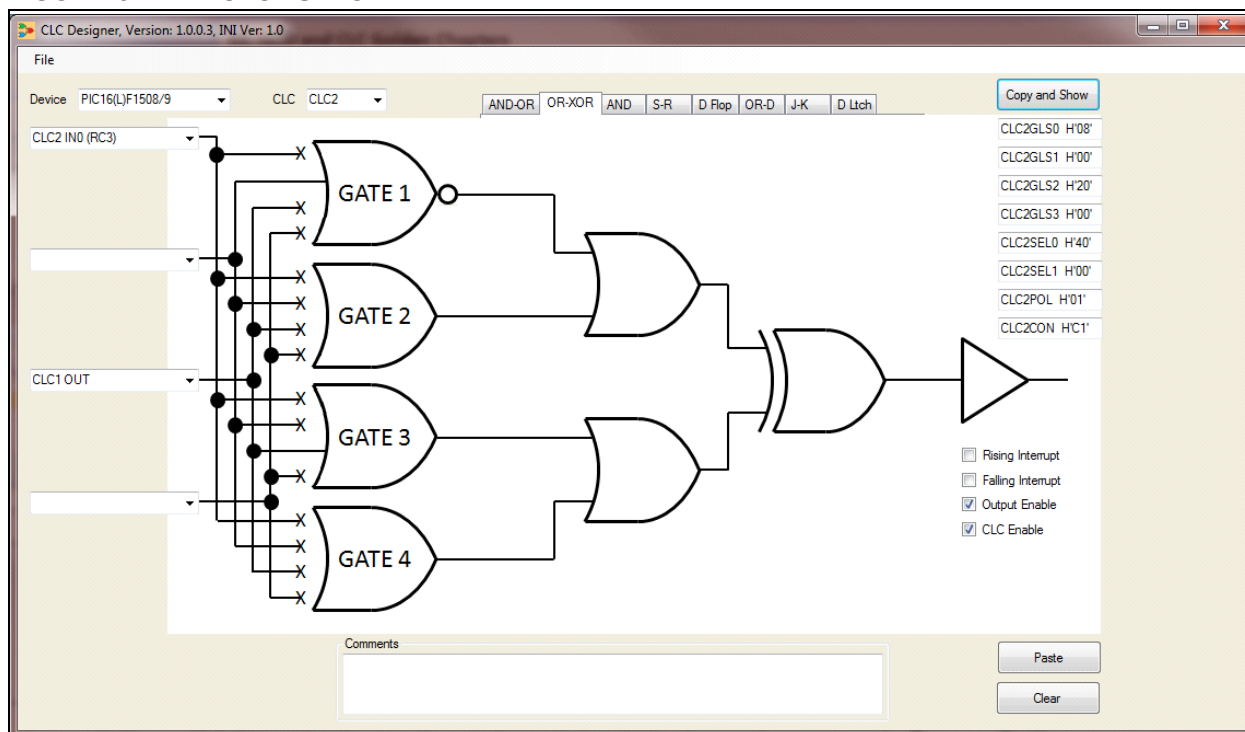
FIGURE 6: CLC2 SETUP
