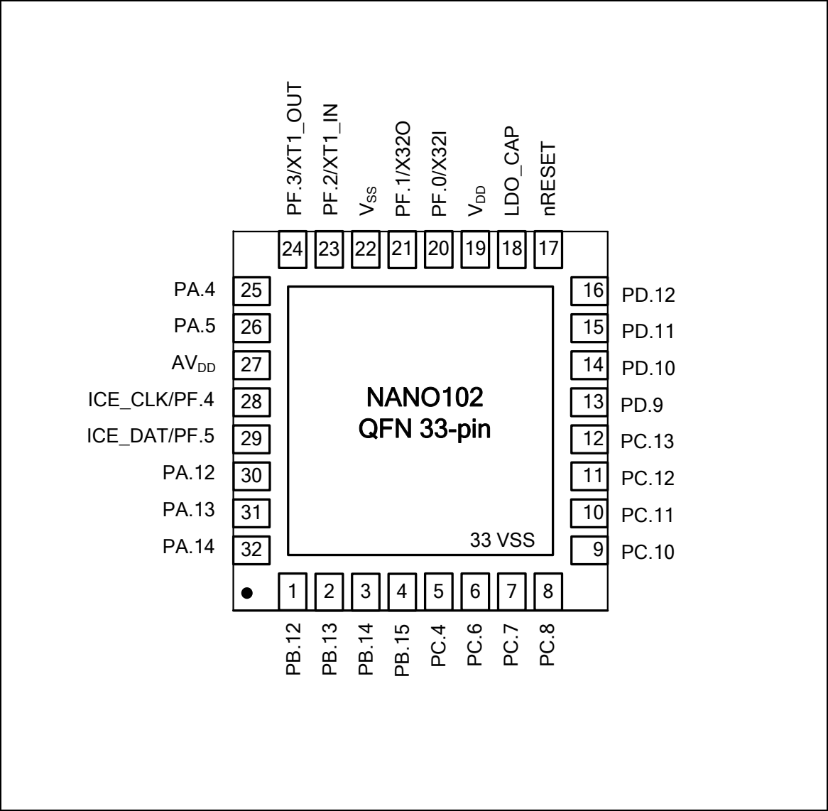
Figure 4-4 NuMicro® Nano102 QFN 32-pin Diagram
