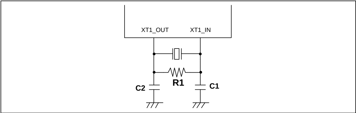
Figure 9-1 Typical Crystal Application Circuit
