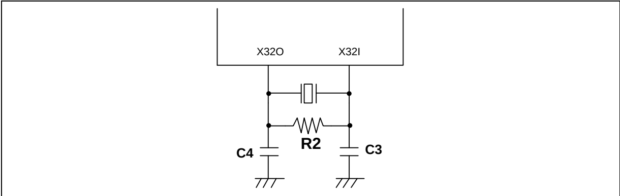
Figure 9-2 Typical Crystal Application Circuit
