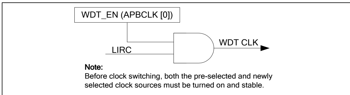
Figure 6-47 Watchdog Timer Clock Control Diagram
