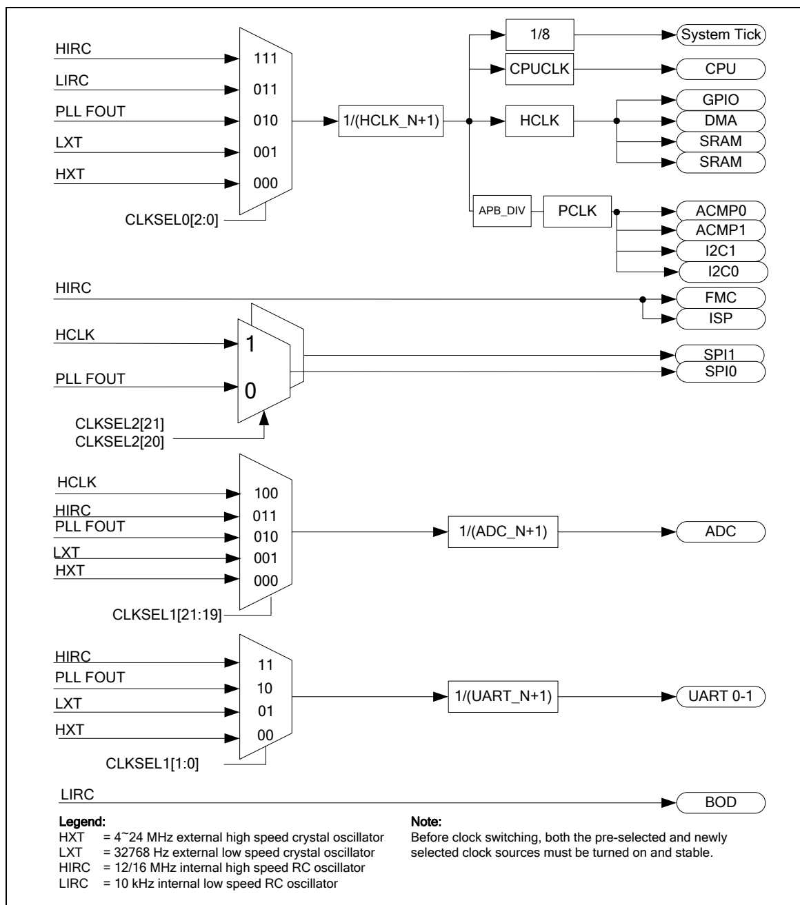
Figure 6-7 Clock Controller Block Diagram (2/3)
