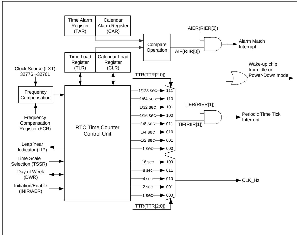
Figure 6-51 RTC Core Block Diagram
