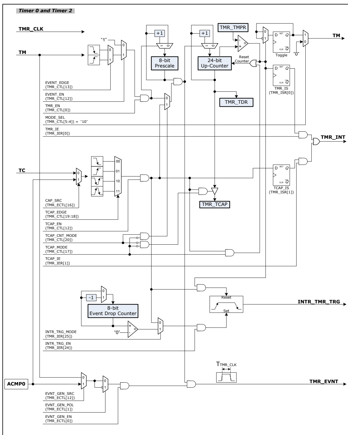
Figure 6-28 Timer 0 and Timer 2 Controller Block Diagram
