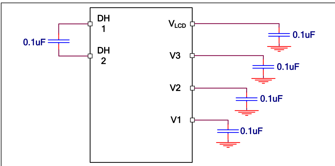
Figure 6-114 1/3 Bias (Charge Pump)
