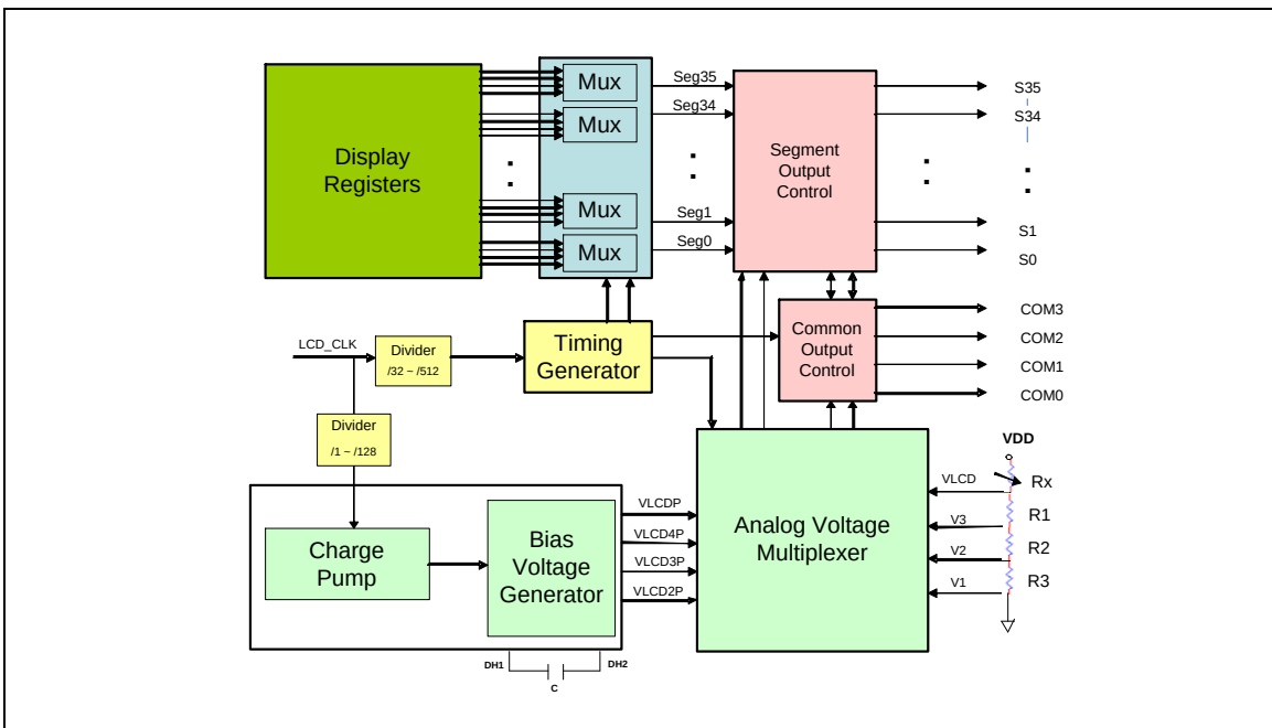
Figure 6-104 LCD Driver Block Diagram
