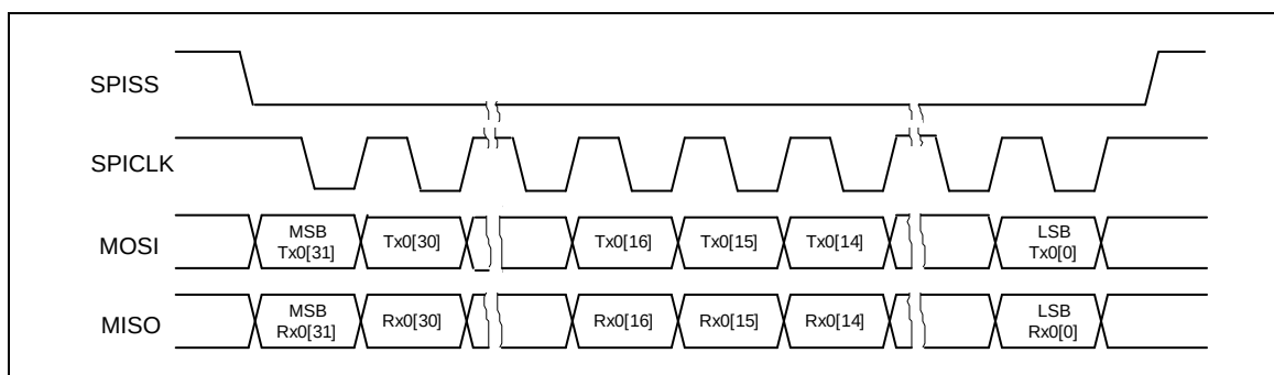
Figure 6-92 SPI 32-bit in One Transaction
