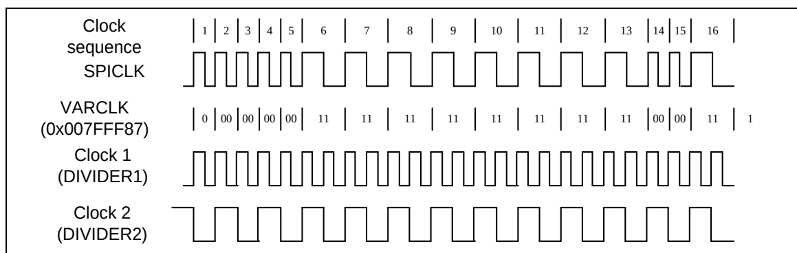
Figure 6-91 SPI Variable Clock Frequency
