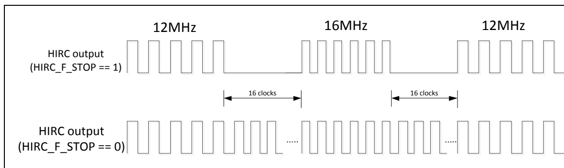
Figure 6-14 HIRC Frequency Change
