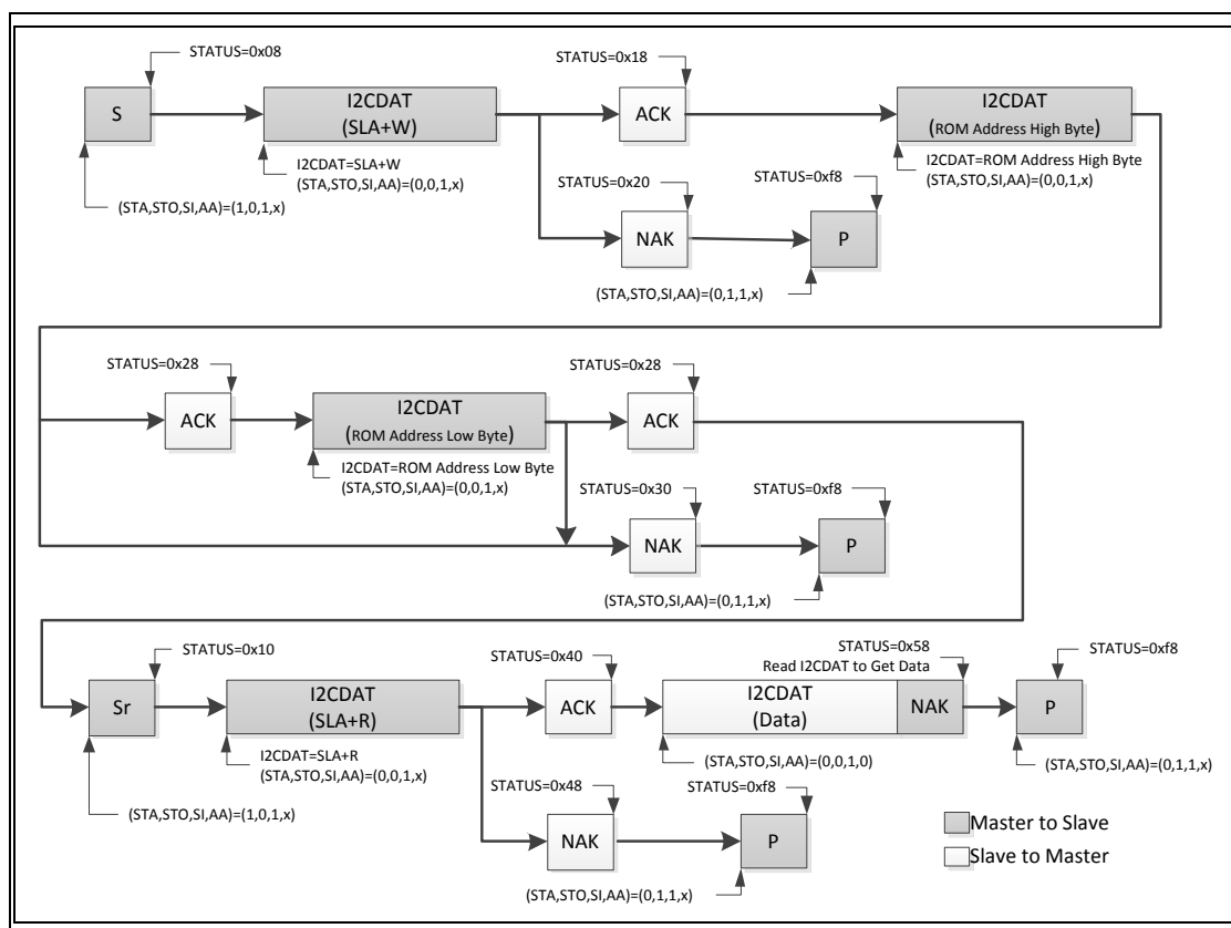
Figure 6-87 Protocol of EEPROM Random Read
