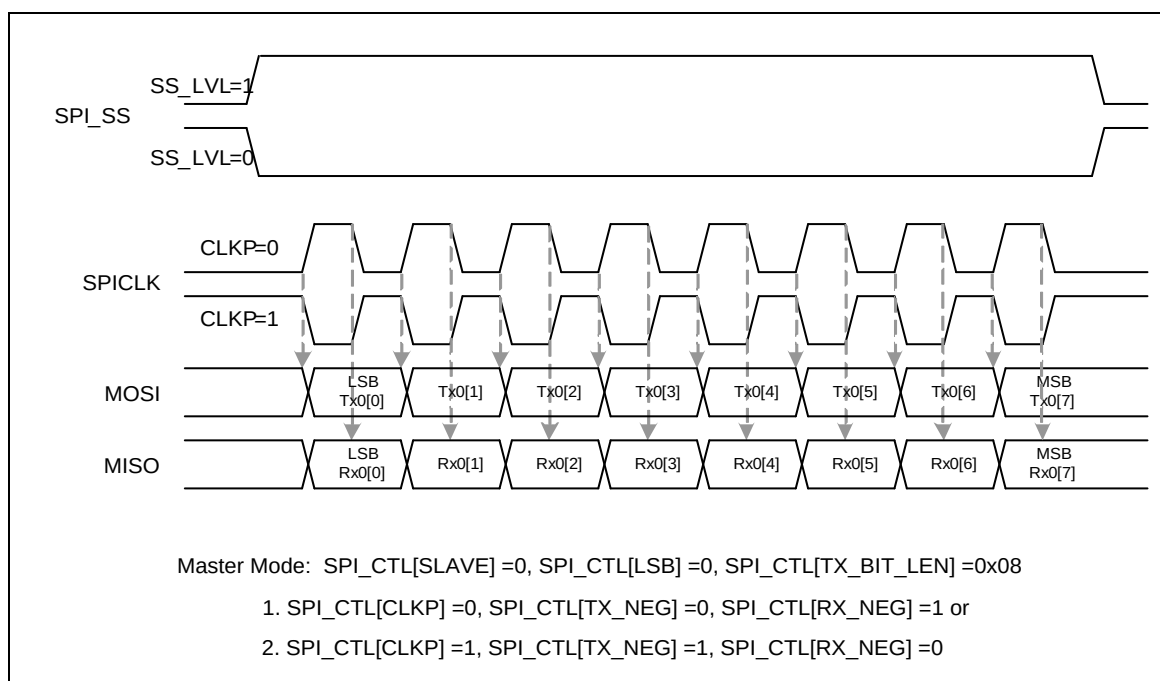
Figure 6-100 SPI Timing in Master Mode (Alternate Phase of SPICLK & LSB = 1)
