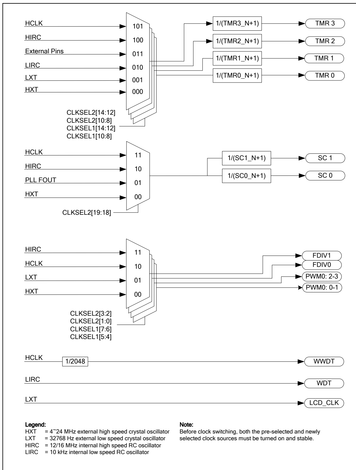
Figure 6-8 Clock Controller Block Diagram (3/3)
