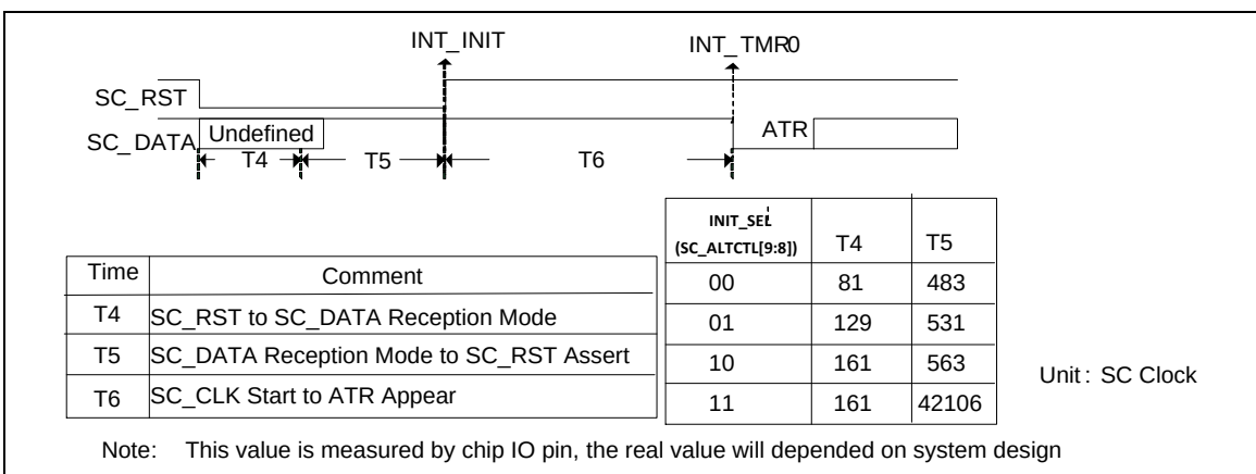
Figure 6-70 SC Warm Reset Sequence
