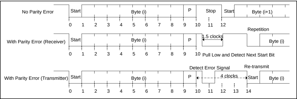
Figure 6-73 SC Error Signal
