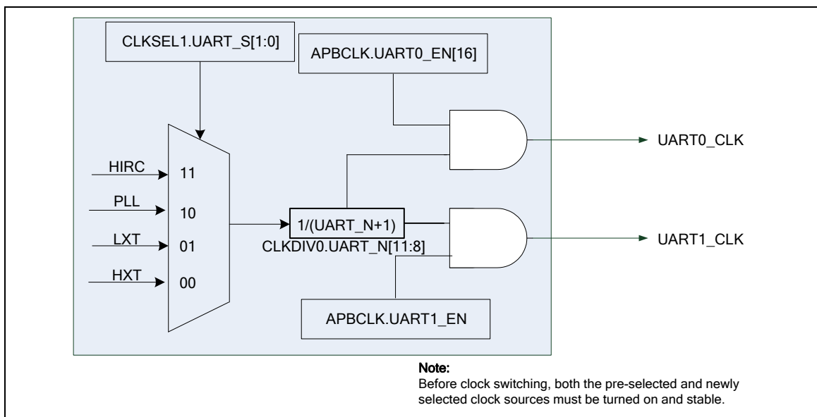
Figure 6-52 UART Clock Control Diagram
