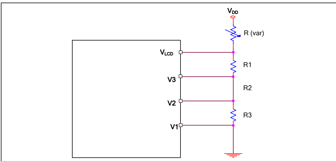
Figure 6-110 1/2 Bias (External Resistor Ladder)
