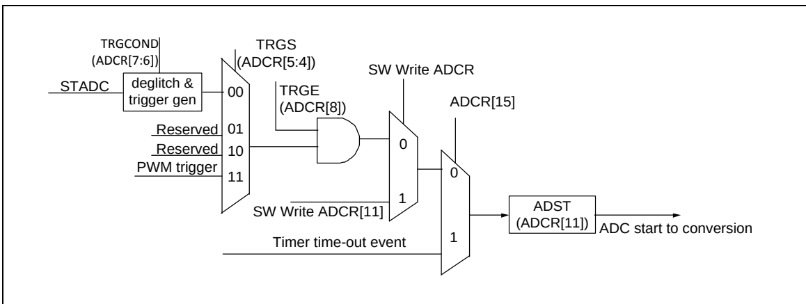
Figure 6-124 ADC Start Conversion Conditions
