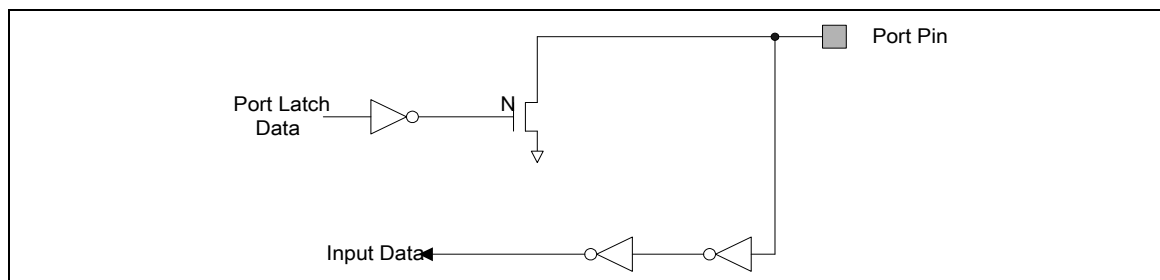
Figure 6-24 Open-Drain Output
