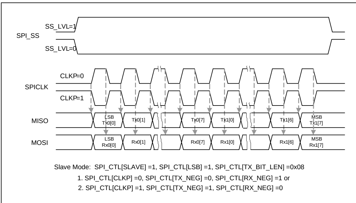
Figure 6-103 SPI Timing in Slave Mode (Alternate Phase of SPICLK)
