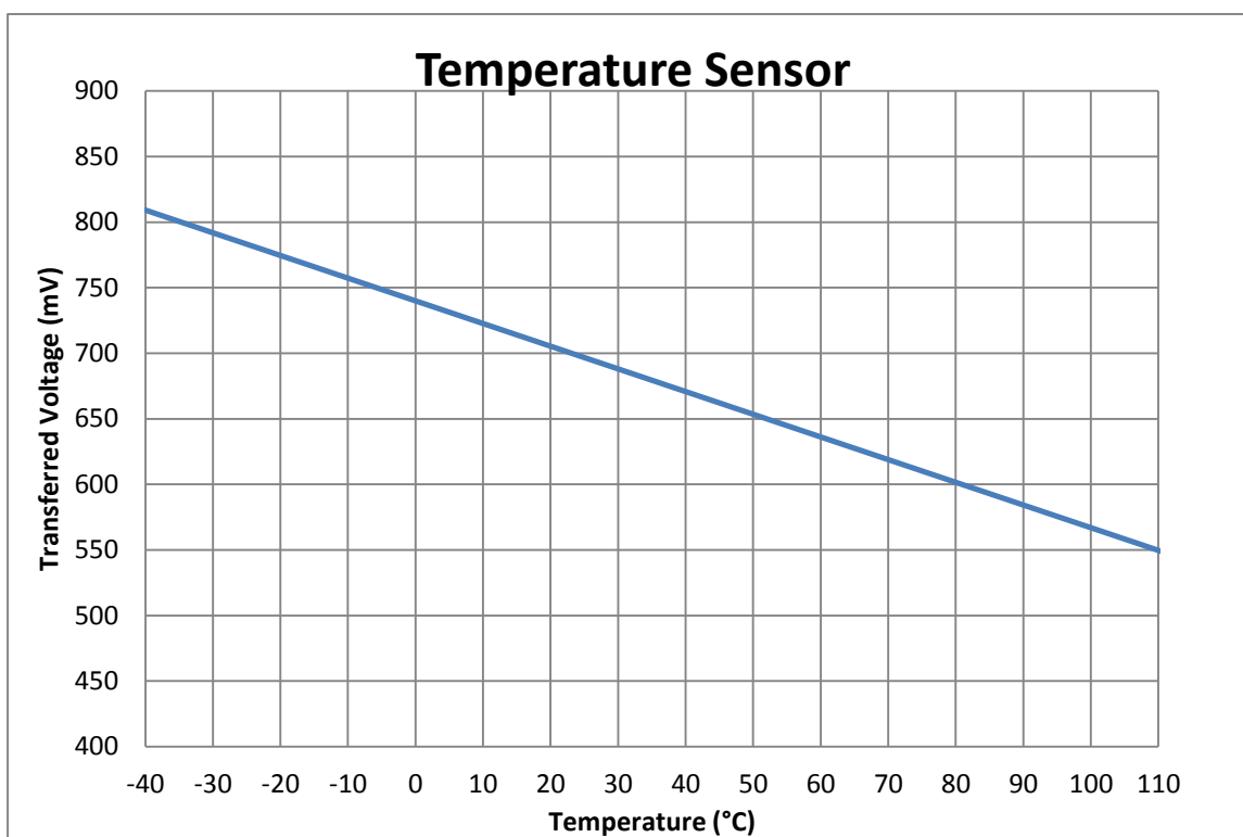
Figure 6-129 Temperature Sensor Transfer Function
