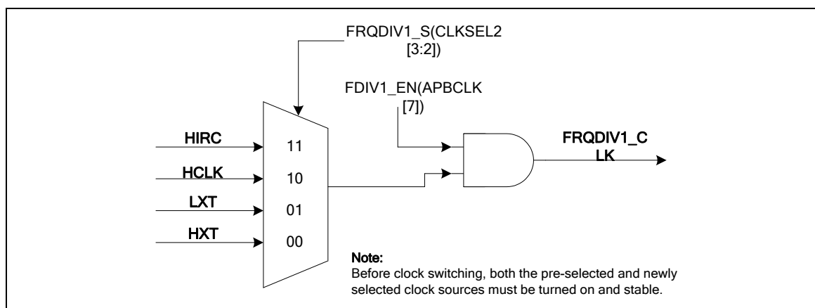
Figure 6-10 Clock Source of Frequency Divider1
