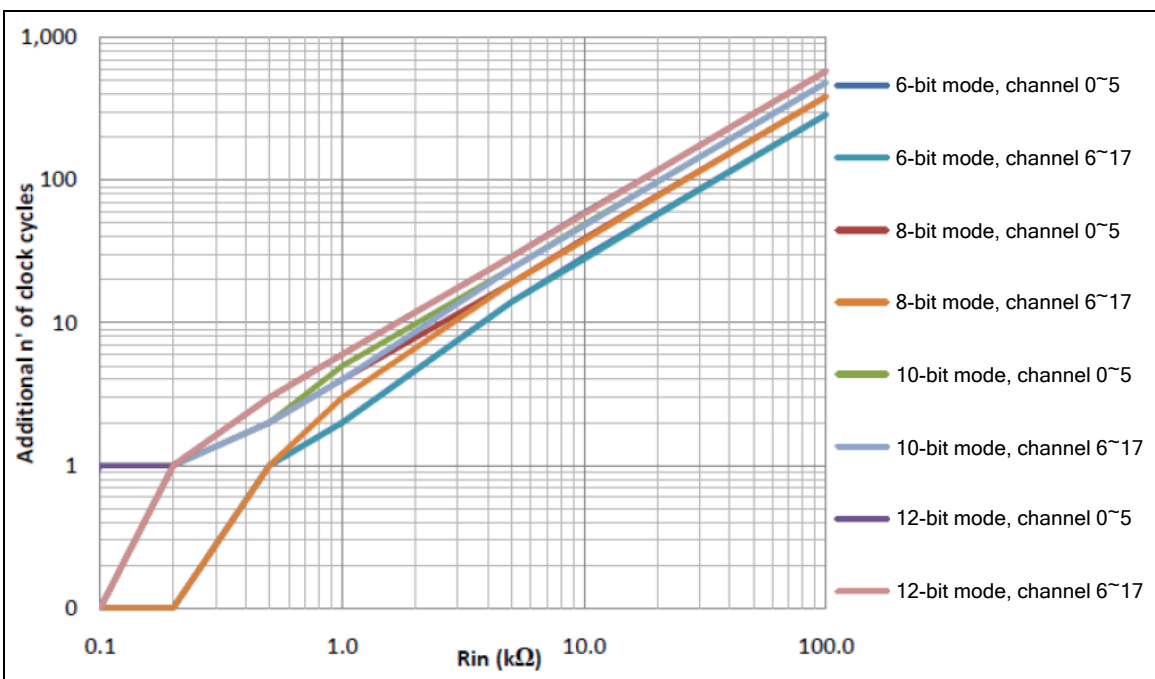
Figure 6-128 Additional Sample and Hold Clock Cycles ( n ) as a Function of the Signal Source Output Resistance R_{in} ( k\Omega )
