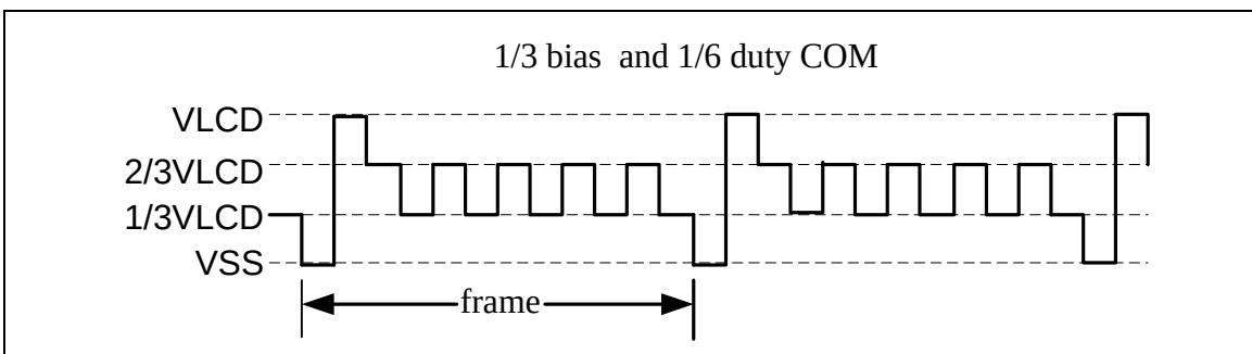
Figure 6-106 COM Signal Waveform
