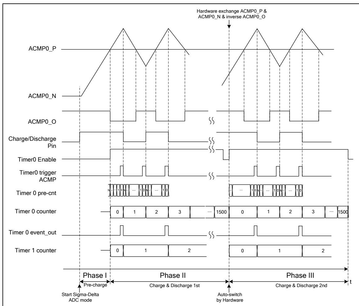
Figure 6-137 ACMP Sigma-Delta ADC Mode Timing
