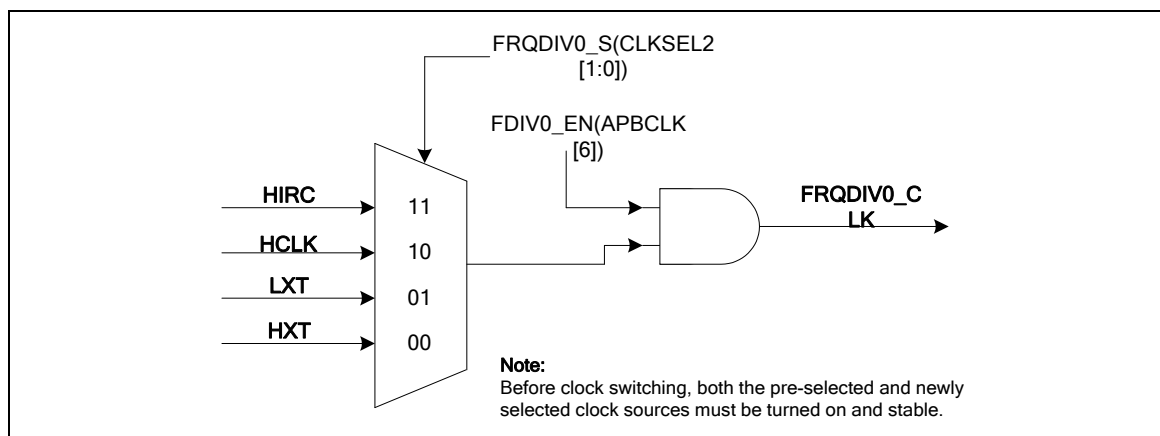
Figure 6-9 Clock Source of Frequency Divider0
