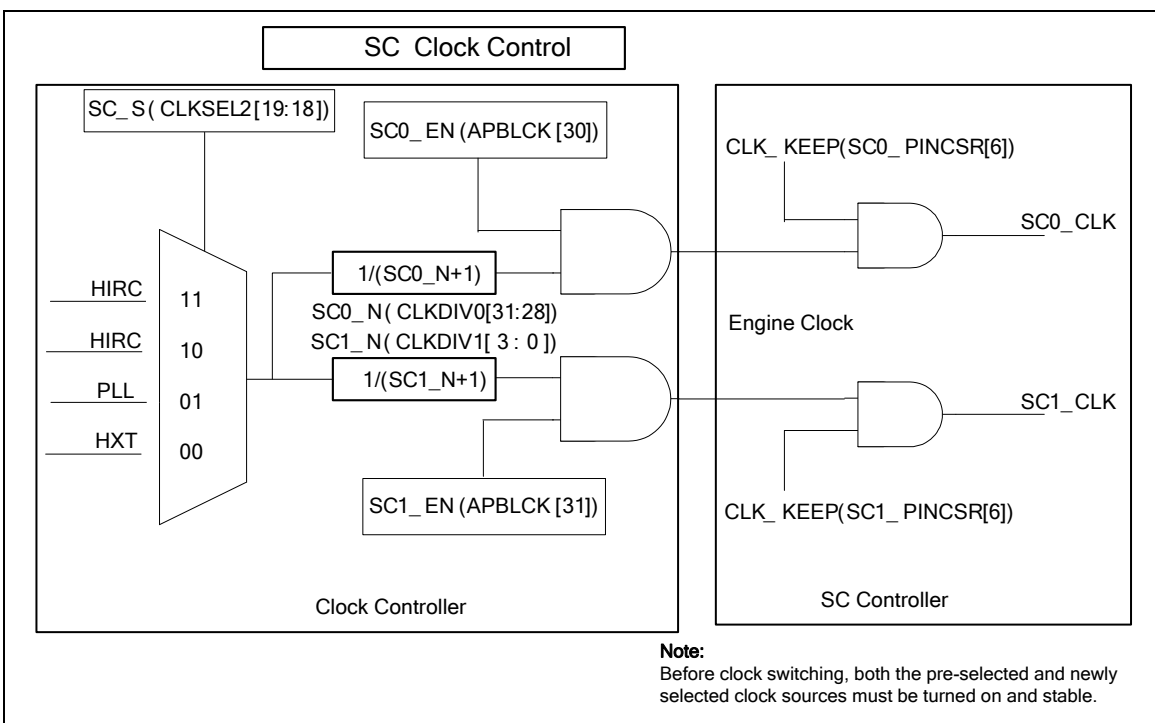
Figure 6-66 SC Clock Control Diagram (4-bit Prescale Counter in Clock Controller)
