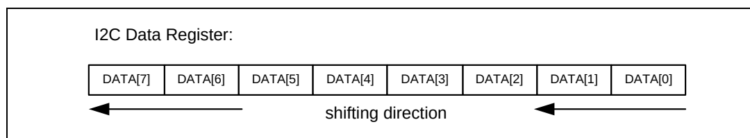
Figure 6-80 I 2 C Data Shifting Direction
