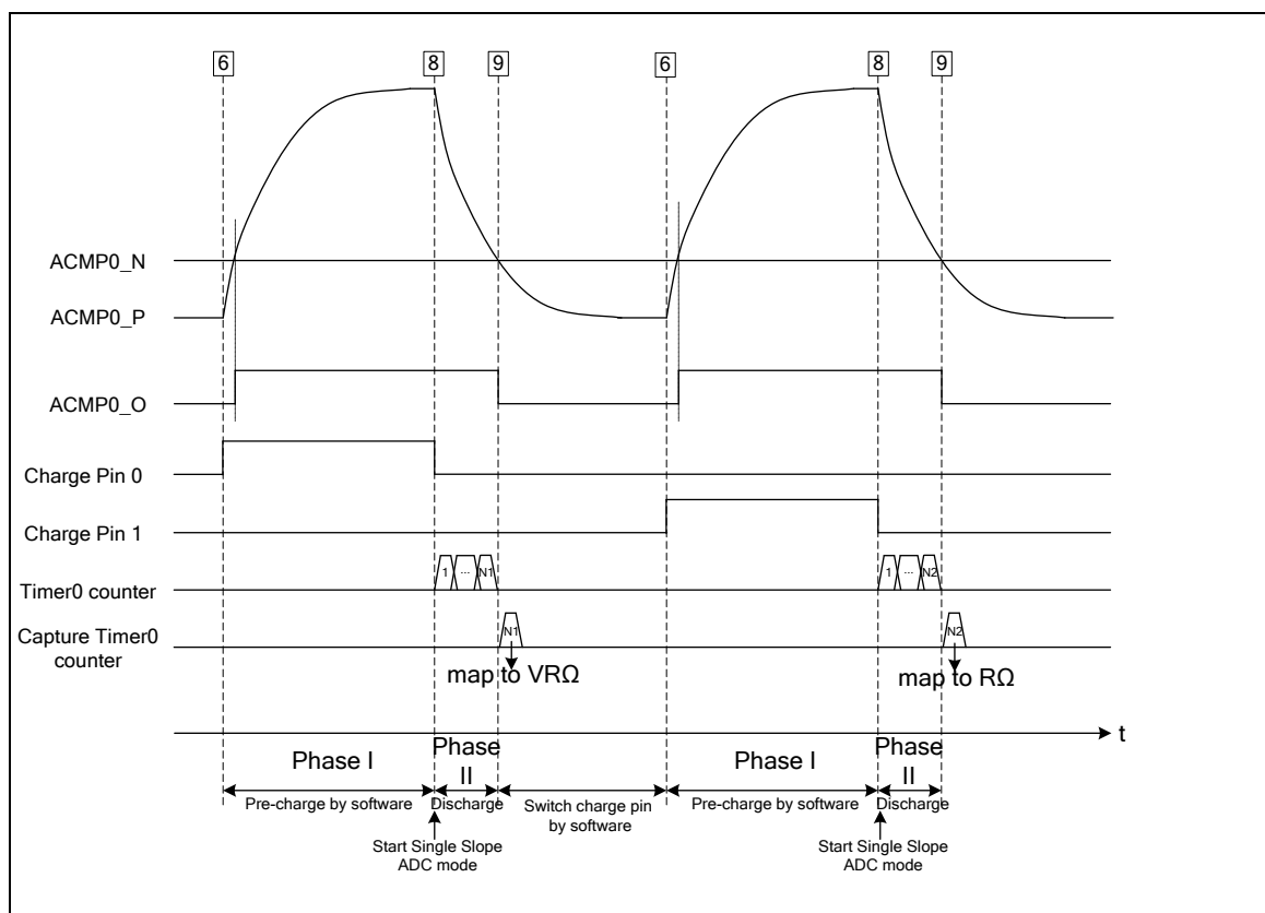
Figure 6-135 ACMP0 Single Slope ADC Mode Timing
