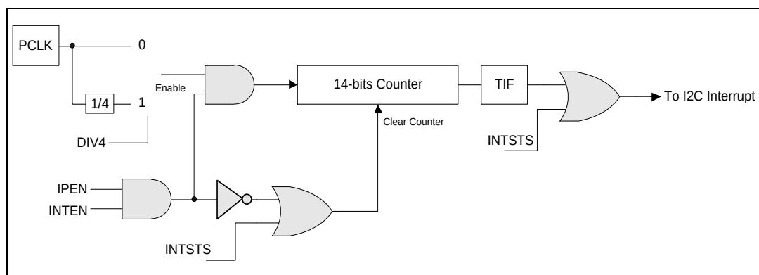
Figure 6-79 I 2 C Time-out Block Diagram
