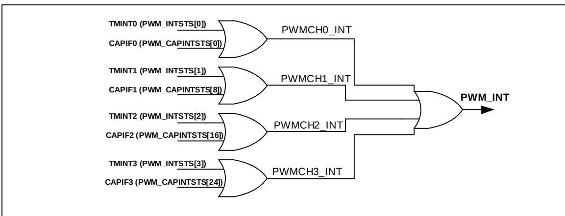
Figure 6-44 PWM-Timer Interrupt
