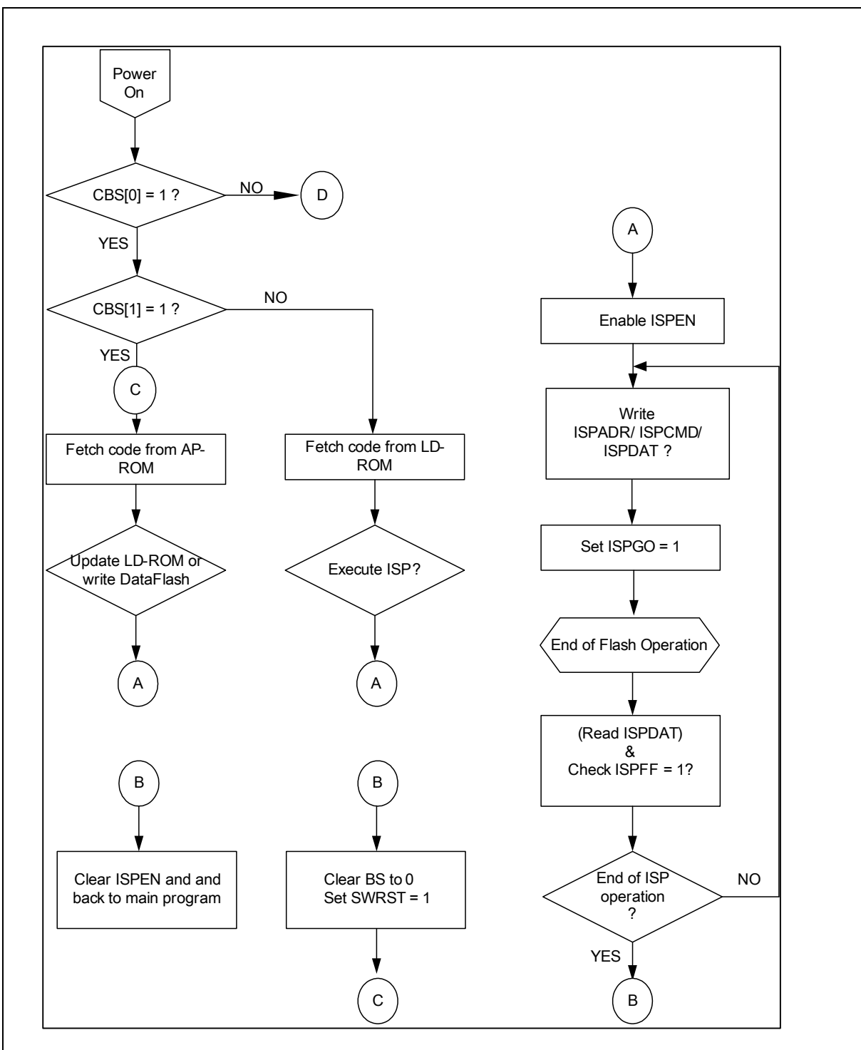
Figure 6-21 ISP Operation Flow
