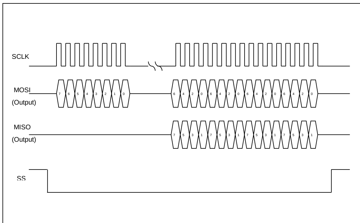
Figure 6-97 SPI DUAL-I/O output Sequence
