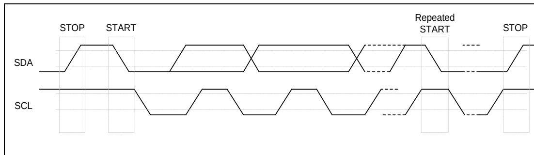
Figure 6-74 I 2 C Bus Timing
