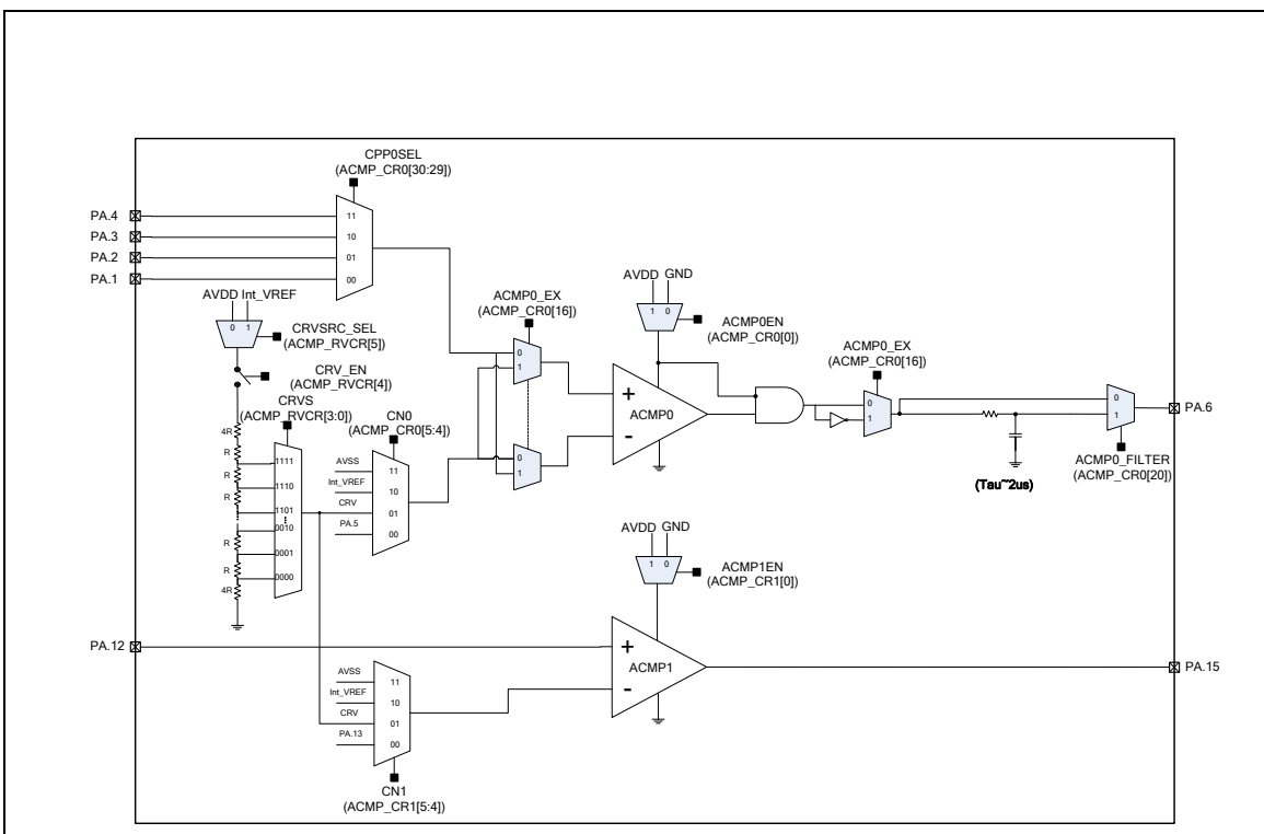
Figure 6-133 Normal Comparator Mode Block Diagram
