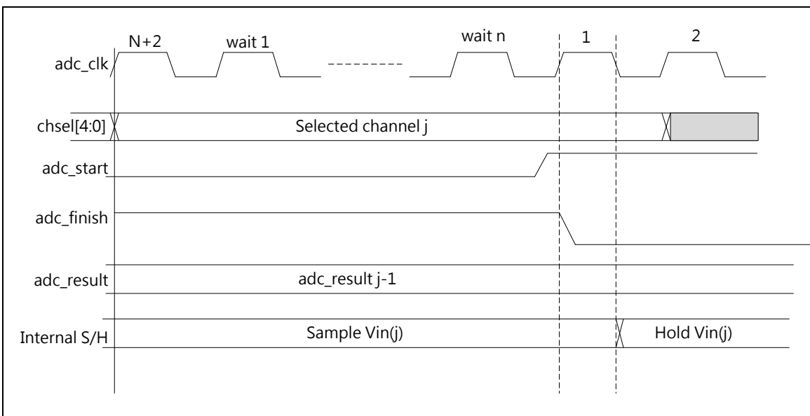
Figure 6-126 Increased Sampling Time Waveform
