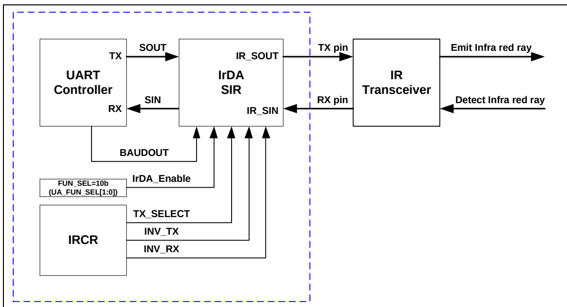
Figure 6-61 IrDA Block Diagram
