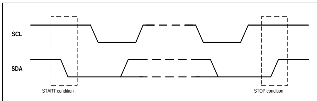
Figure 6-76 I 2 C START and STOP Conditions
