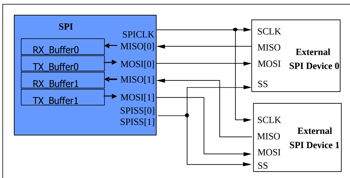
Figure 6-95 SPI 2-bit Transfer Mode
