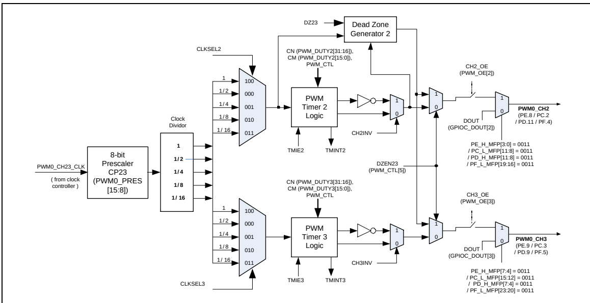
Figure 6-36 PWM Generator for Channel 2, 3
