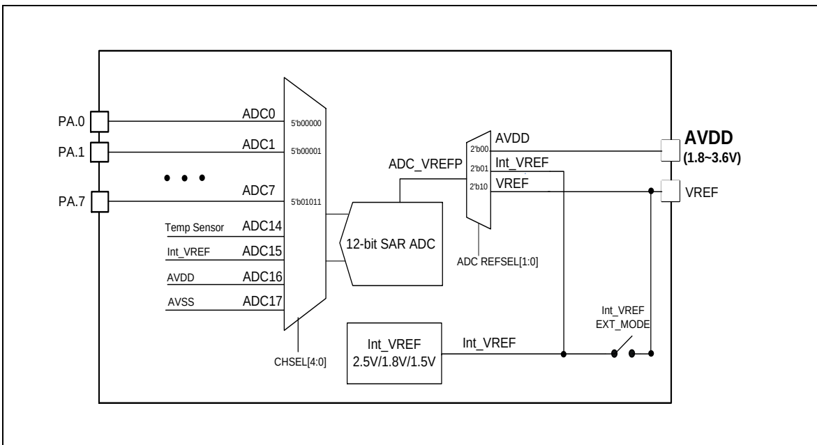
Figure 6-116 ADC Block Diagram
