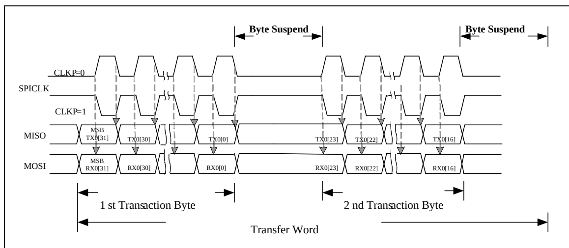
Figure 6-94 SPI Byte Suspend Mode
