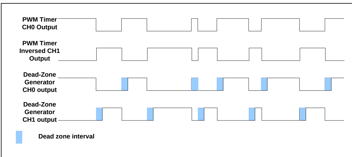
Figure 6-42 Paired PWM Output with Dead Zone Generation Operation
