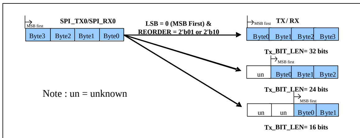
Figure 6-93 SPI Byte Reorder
