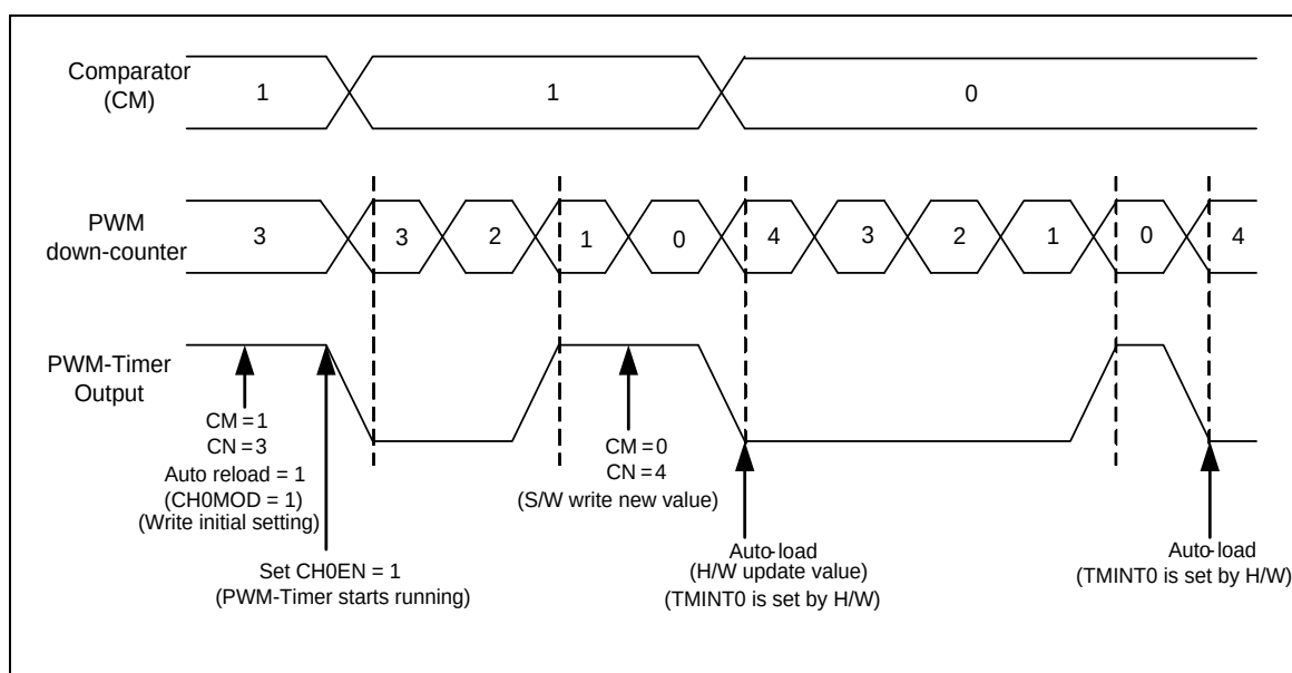
Figure 6-38 PWM-Timer Operation in Edge-aligned Mode
