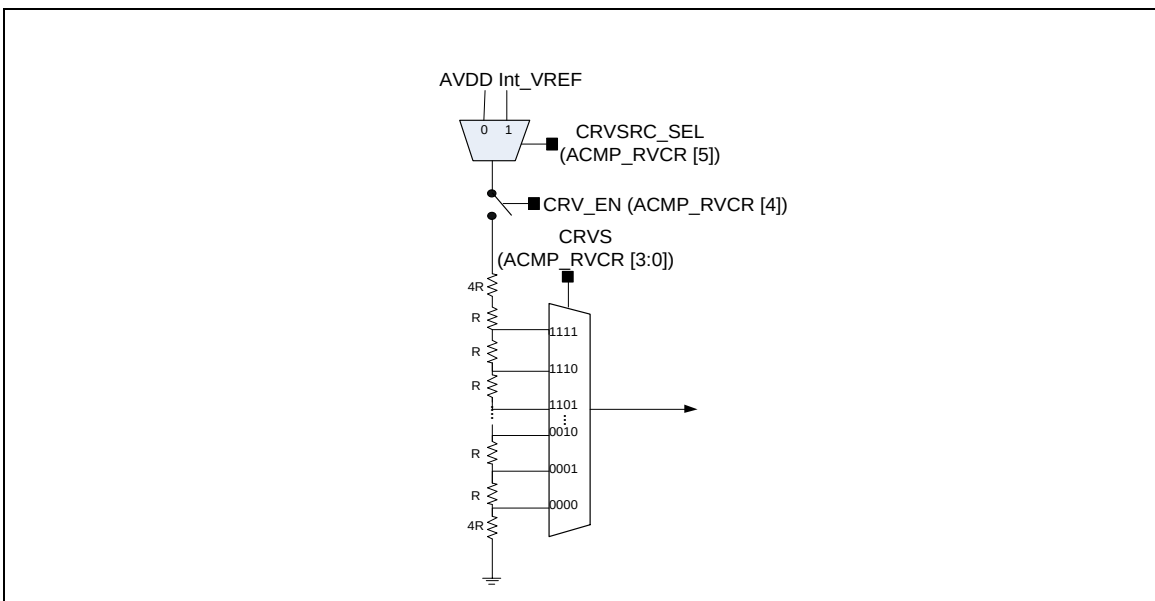
Figure 6-132 Comparator Reference Voltage Block Diagram
