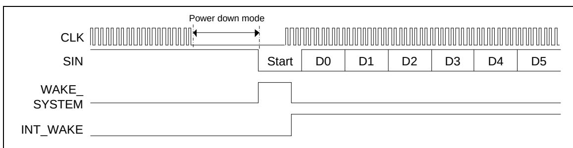
Figure 6-58 UART DATA Wake-Up
