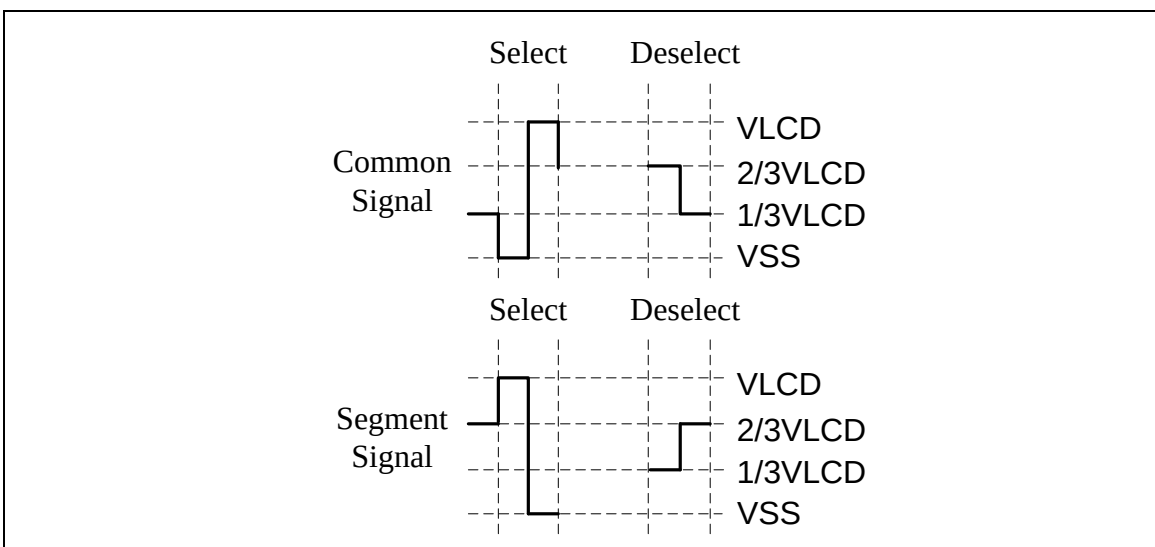
Figure 6-107 SEG Signal Waveform
