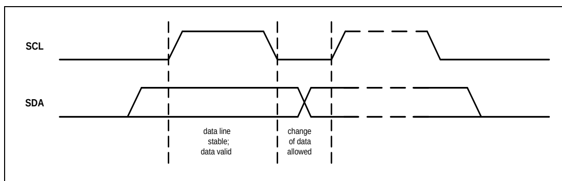
Figure 6-77 Bit Transfer on I 2 C Bus
