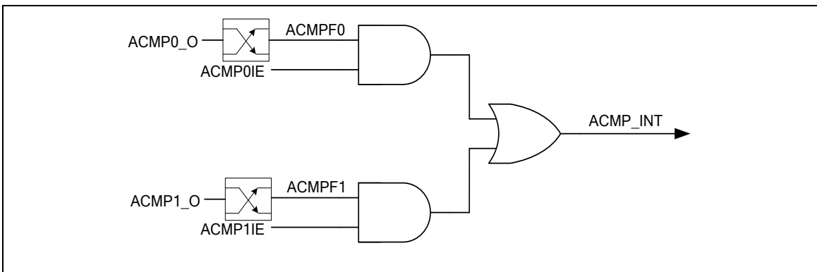
Figure 6-138 Analog Comparator Interrupt Sources
