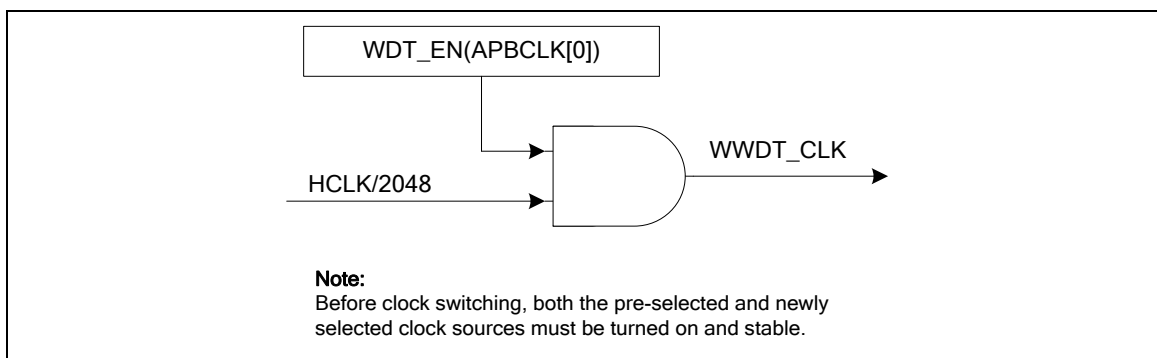
Figure 6-49 Window Watchdog Controller Block Diagram
