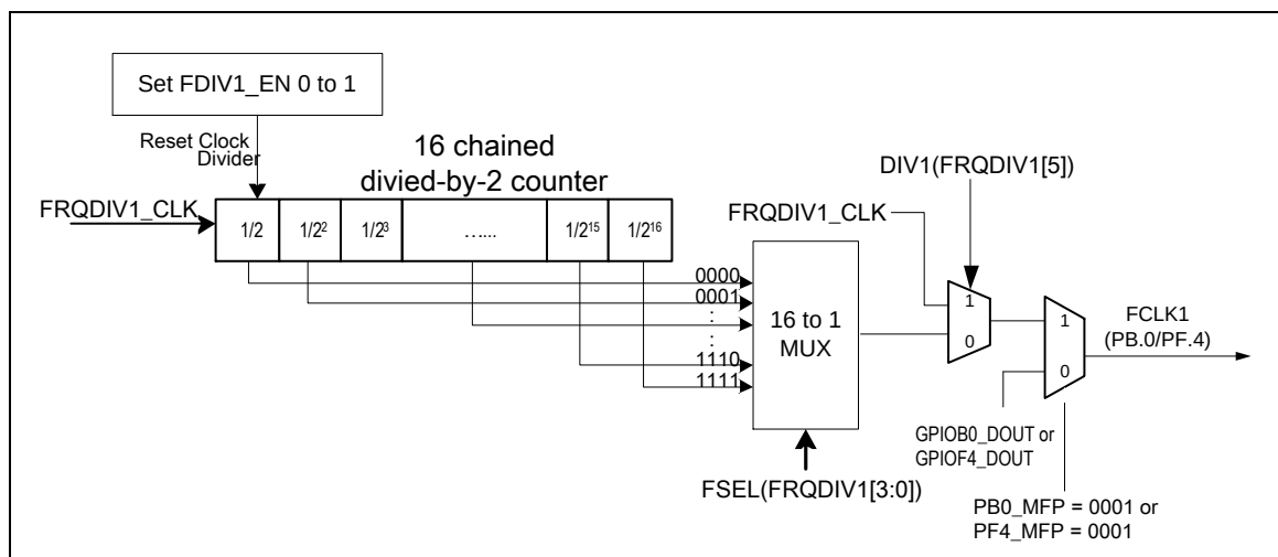
Figure 6-12 Frequency Divider1 Block Diagram
