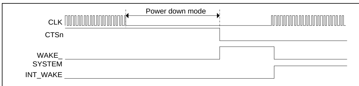
Figure 6-57 UART CTSn Wake-Up Case 2
