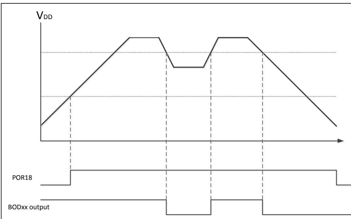
Figure 6-4 Power Supervisors
