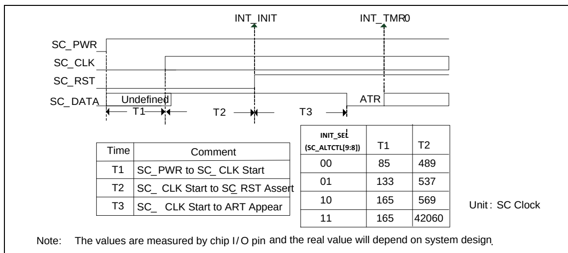
Figure 6-69 SC Activation Sequence
