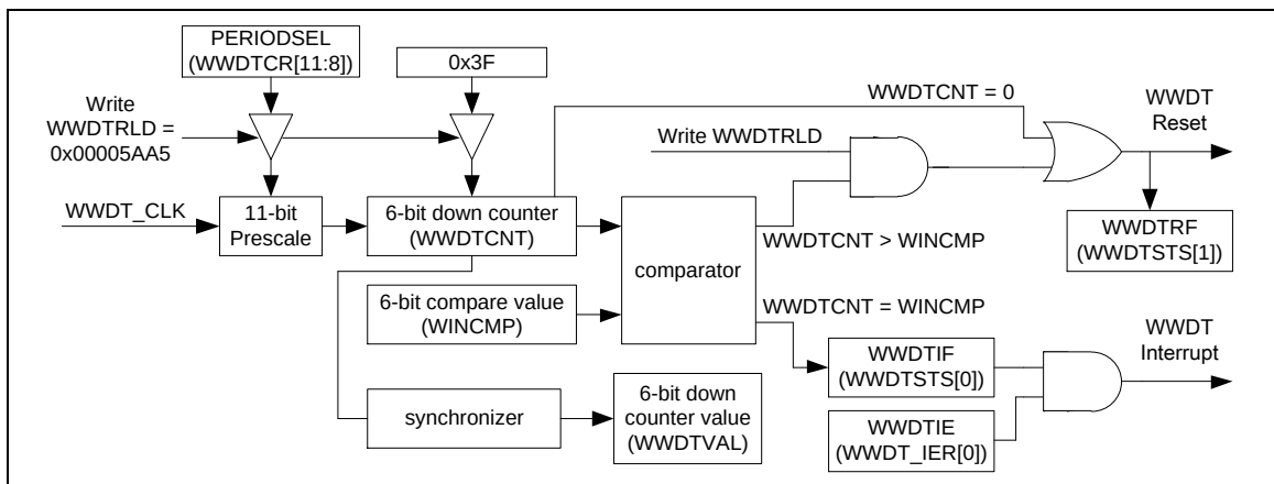
Figure 6-50 Watchdog Controller Block Diagram
