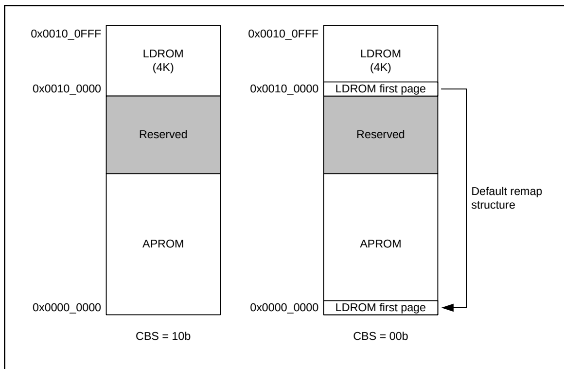
Figure 6-18 Executable Range of Code with IAP Function Enabled
