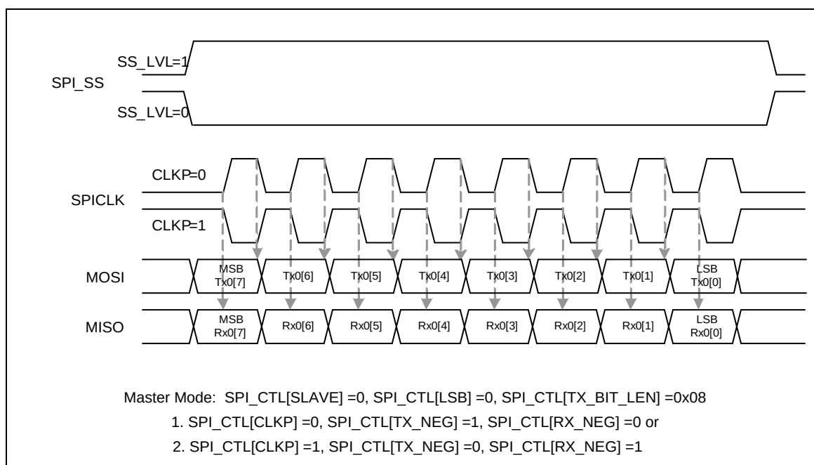
Figure 6-99 SPI Timing in Master Mode
