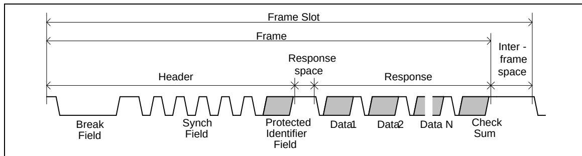
Figure 6-64 Structure of LIN Frame
