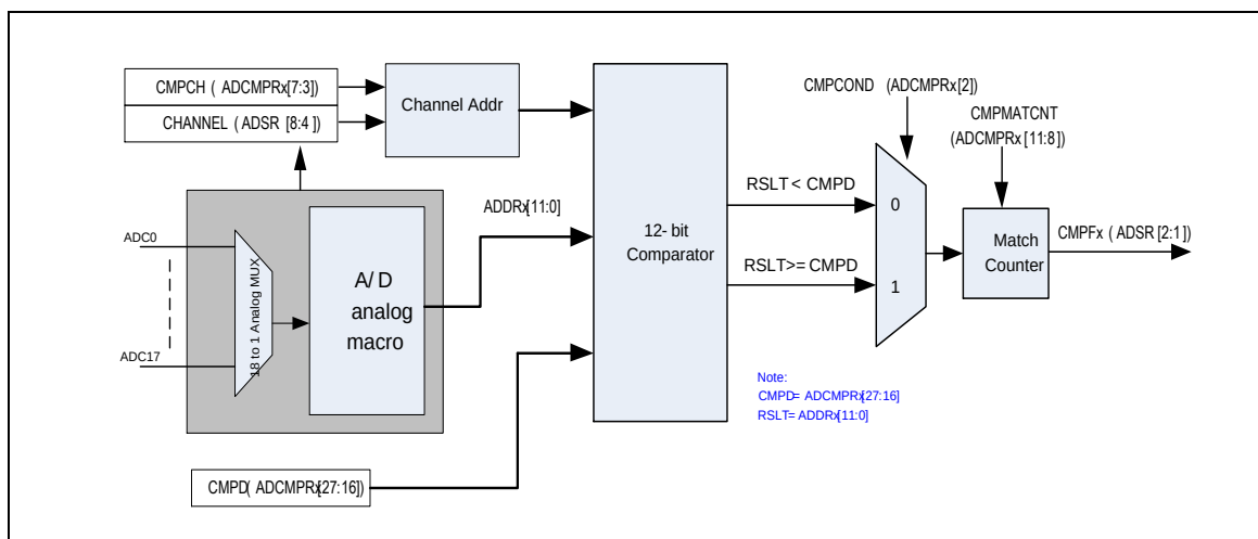
Figure 6-122 ADC Conversion Result Monitor Logic Diagram
