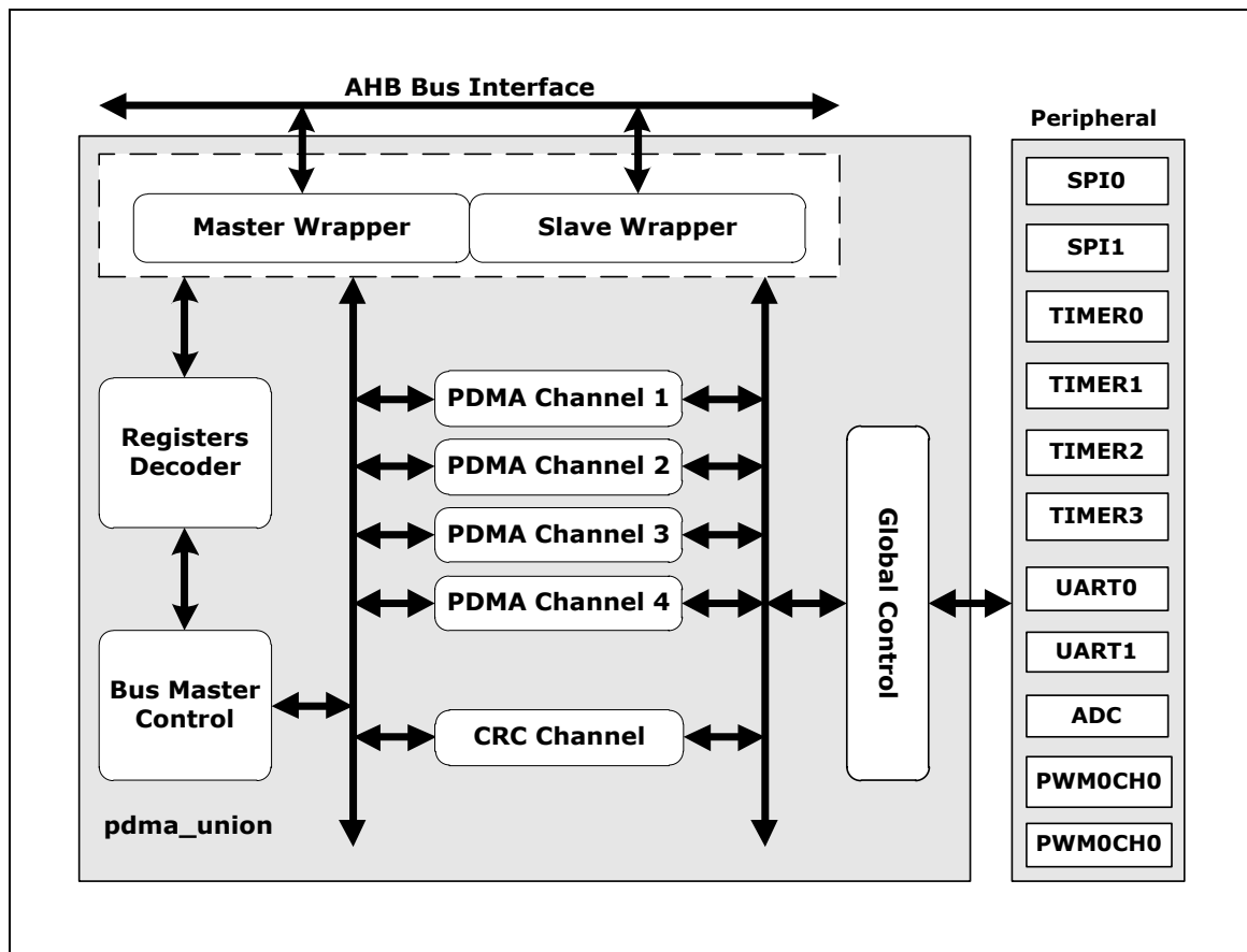
Figure 6-25 DMA Controller Block Diagram
