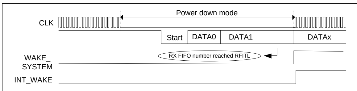
Figure 6-59 UART Receive DATA FIFO Reach RFITL Wake-Up
