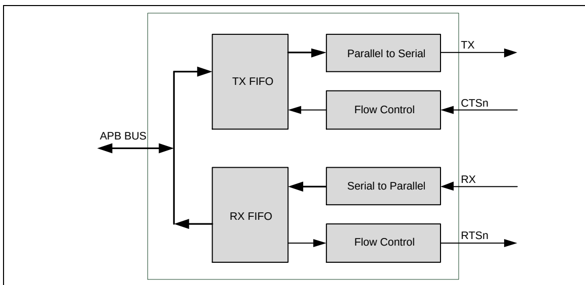
Figure 6-55 UART Auto-Flow Control Block Diagram
