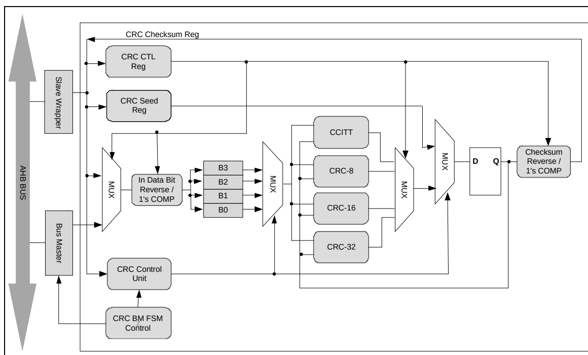
Figure 6-27 CRC Generator Block Diagram
