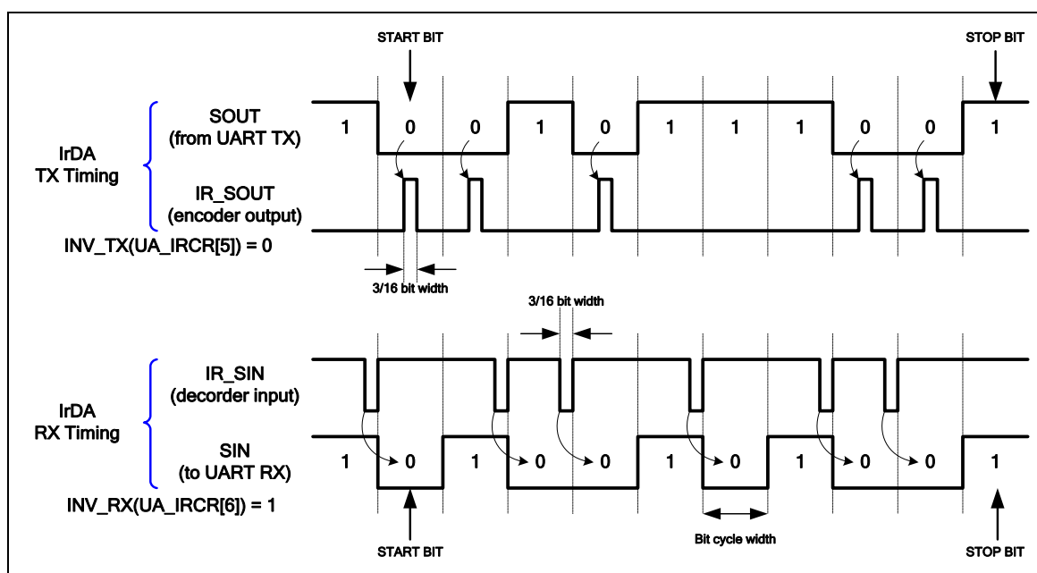
Figure 6-62 IrDA TX/RX Timing Diagram
