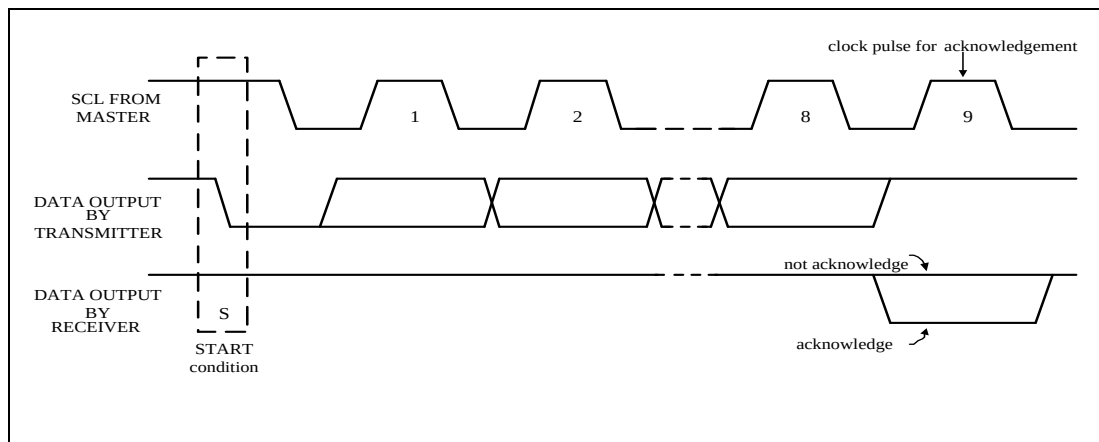
Figure 6-78 Acknowledge on I 2 C Bus
