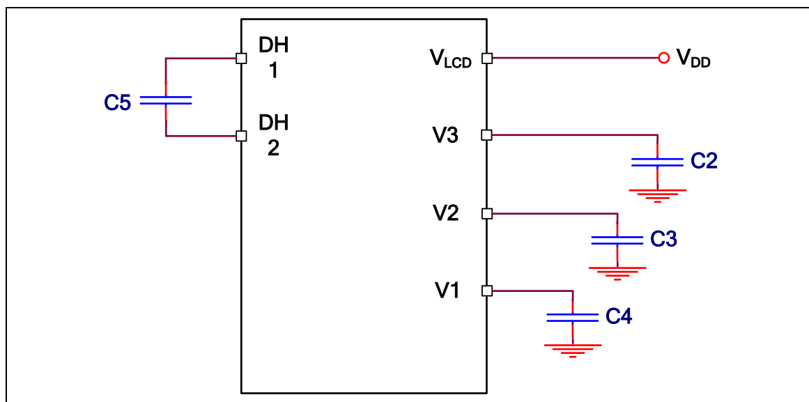
Figure 6-65 1/2 Bias (External Capacitor Ladder)
