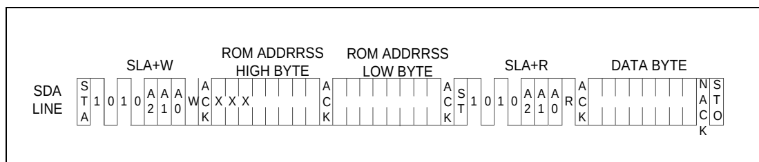
Figure 6-86 EEPROM Random Read
