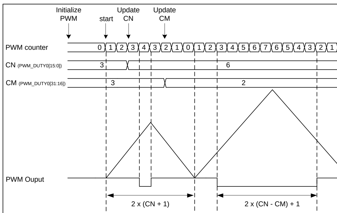
Figure 6-39 PWM-Timer Operation in Center-aligned Mode
