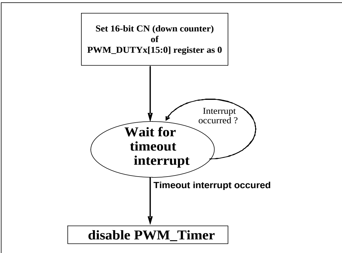
Figure 6-45 PWM-Timer Stop Method 1
