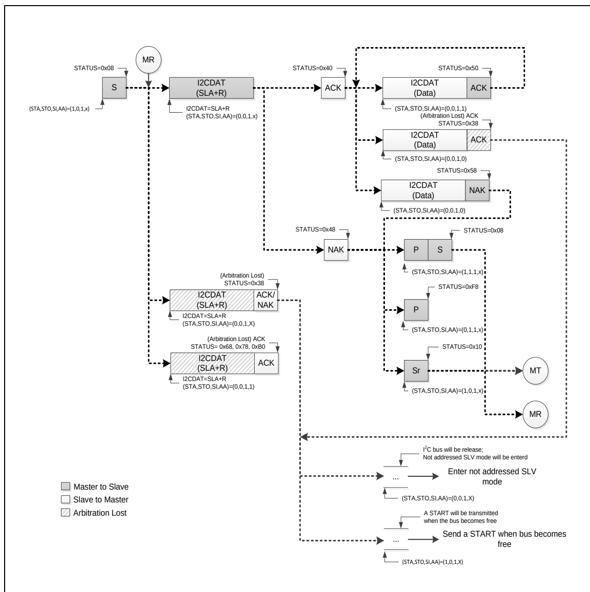
Figure 6-83 Master Receiver Mode Control Flow
