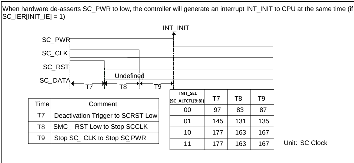
Figure 6-71 SC Deactivation Sequence
