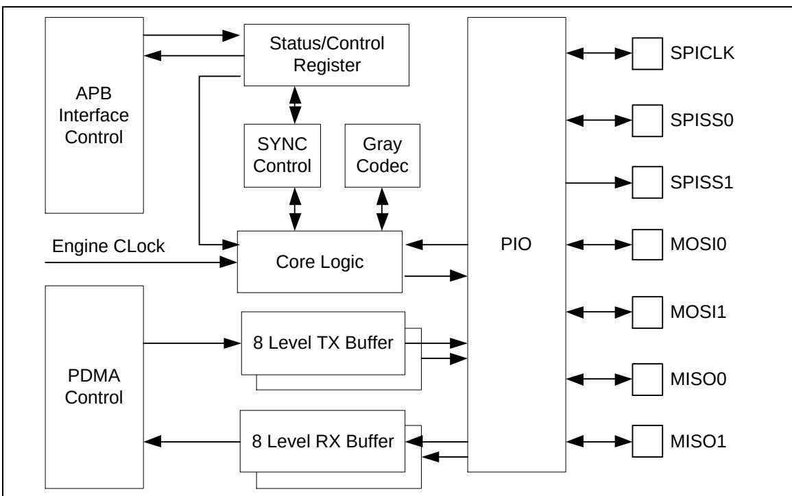
Figure 6-88 SPI Block Diagram
