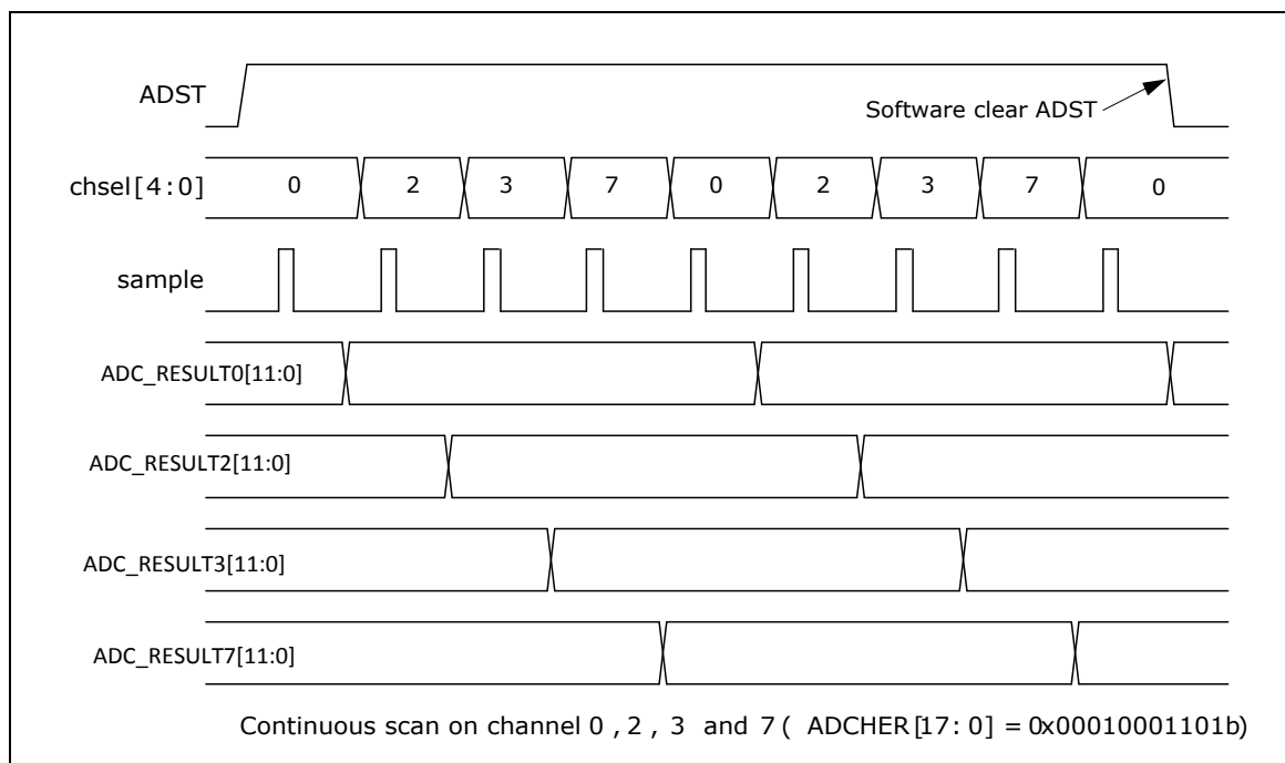
Figure 6-121 ADC Continuous Scan on Enabled Channels Timing Diagram
