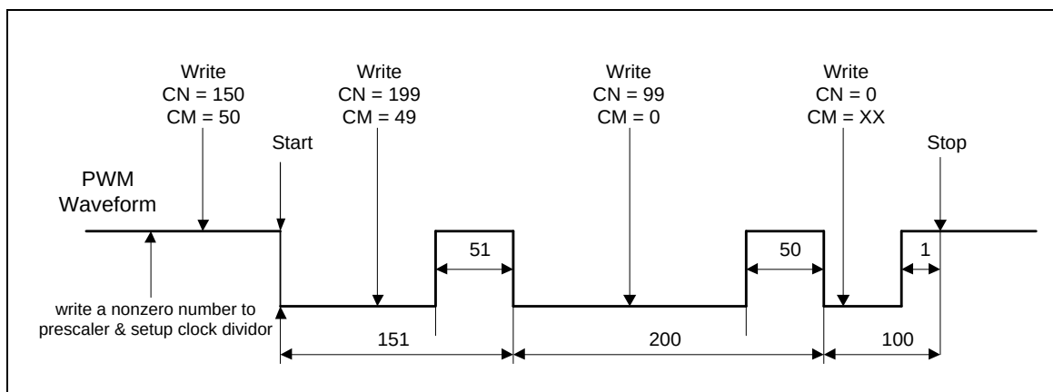
Figure 6-40 PWM Double Buffer Illustration
