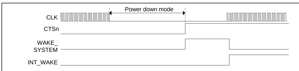
Figure 6-56 UART CTSn Wake-Up Case 1
