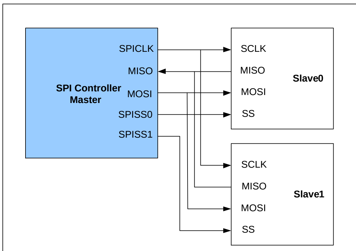
Figure 6-89 SPI Master Mode Application Block Diagram
