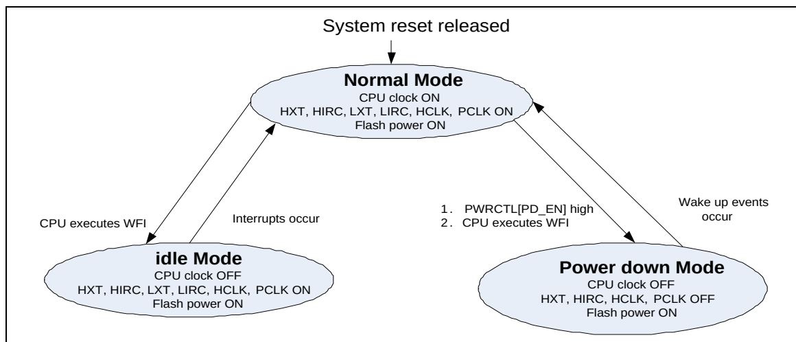
Figure 6-2 Power Modes
