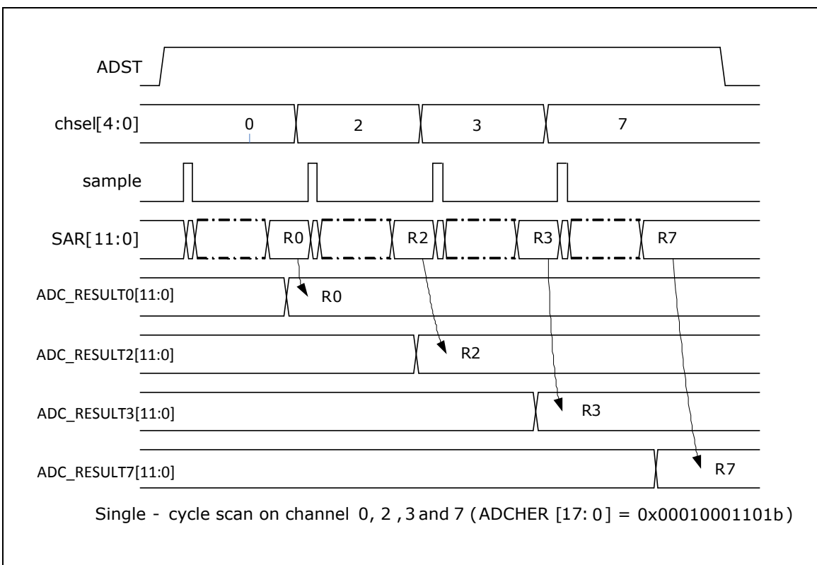
Figure 6-120 ADC Single-cycle Scan on Enabled Channels Timing Diagram
