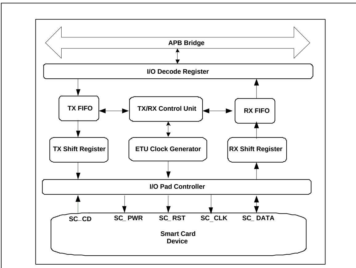
Figure 6-67 SC Controller Block Diagram
