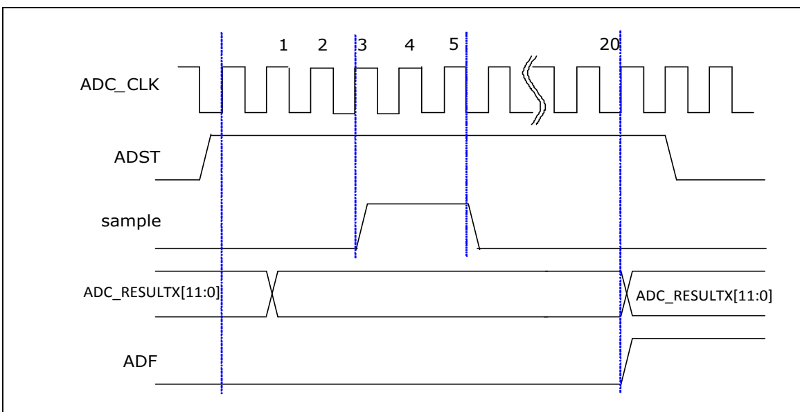
Figure 6-119 ADC Single Mode Conversion Timing Diagram
