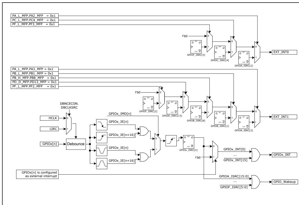
Figure 6-22 GPIO Block Diagram
