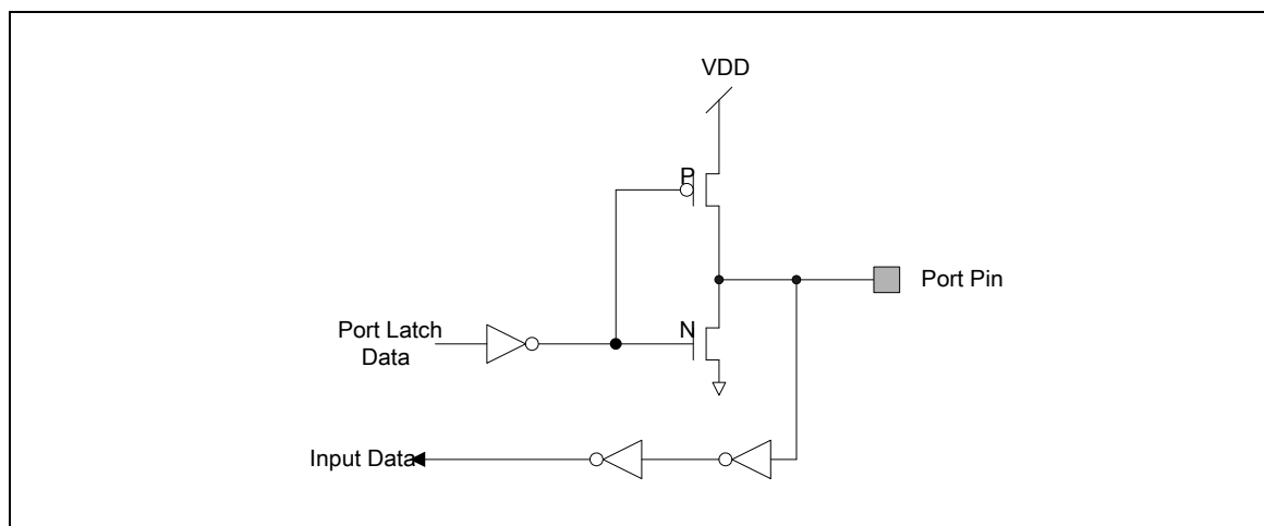
Figure 6-23 Push-Pull Output
