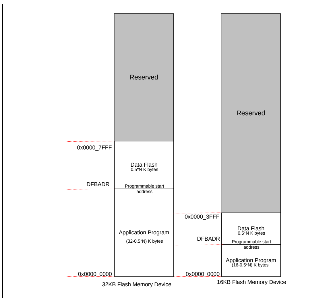
Figure 6-19 16/32KB Flash Memory Structure
