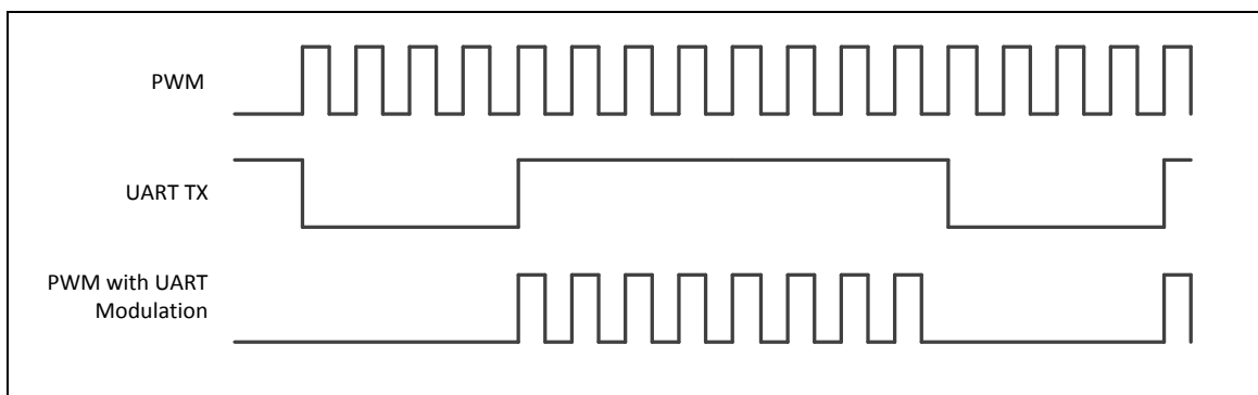
Figure 6-65 UART with PWM Modulation Waveform
