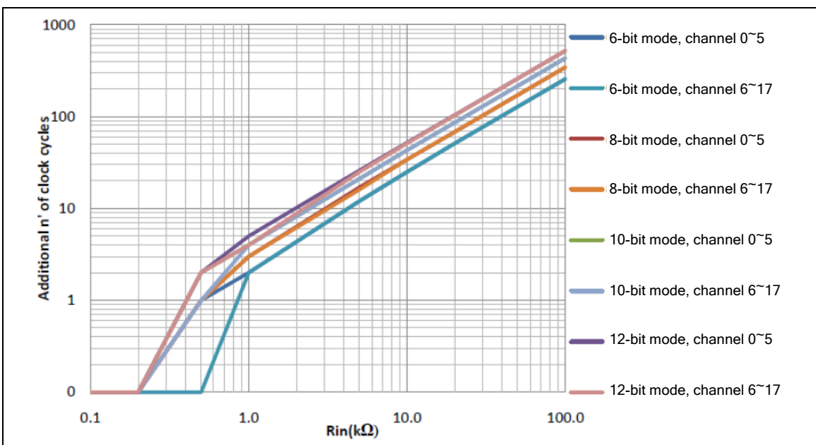
Figure 6-127 Additional Sample and Hold Clock Cycles ( n ) as a Function of the Signal Source Output Resistance R_{in} ( k\Omega )
