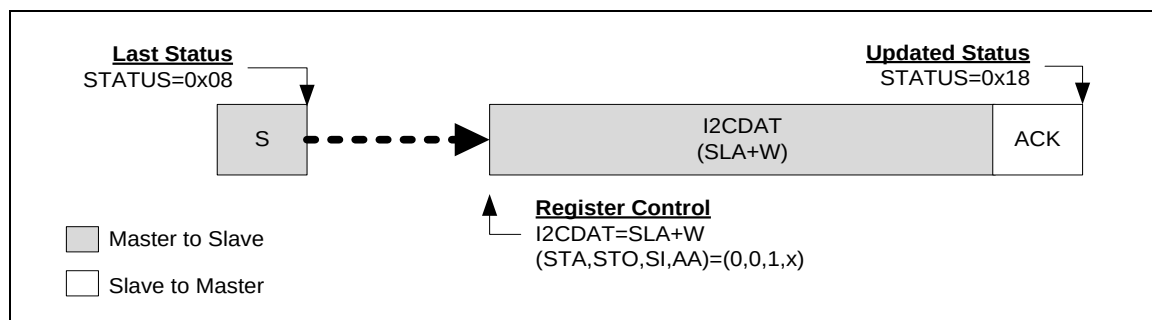
Figure 6-81 Control I2C Bus according to Current I 2 C Status
