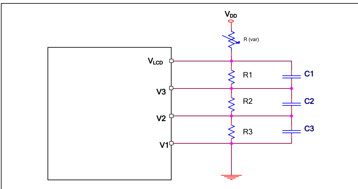
Figure 6-111 1/3 Bias (Resistor Ladder with Capacitor)
