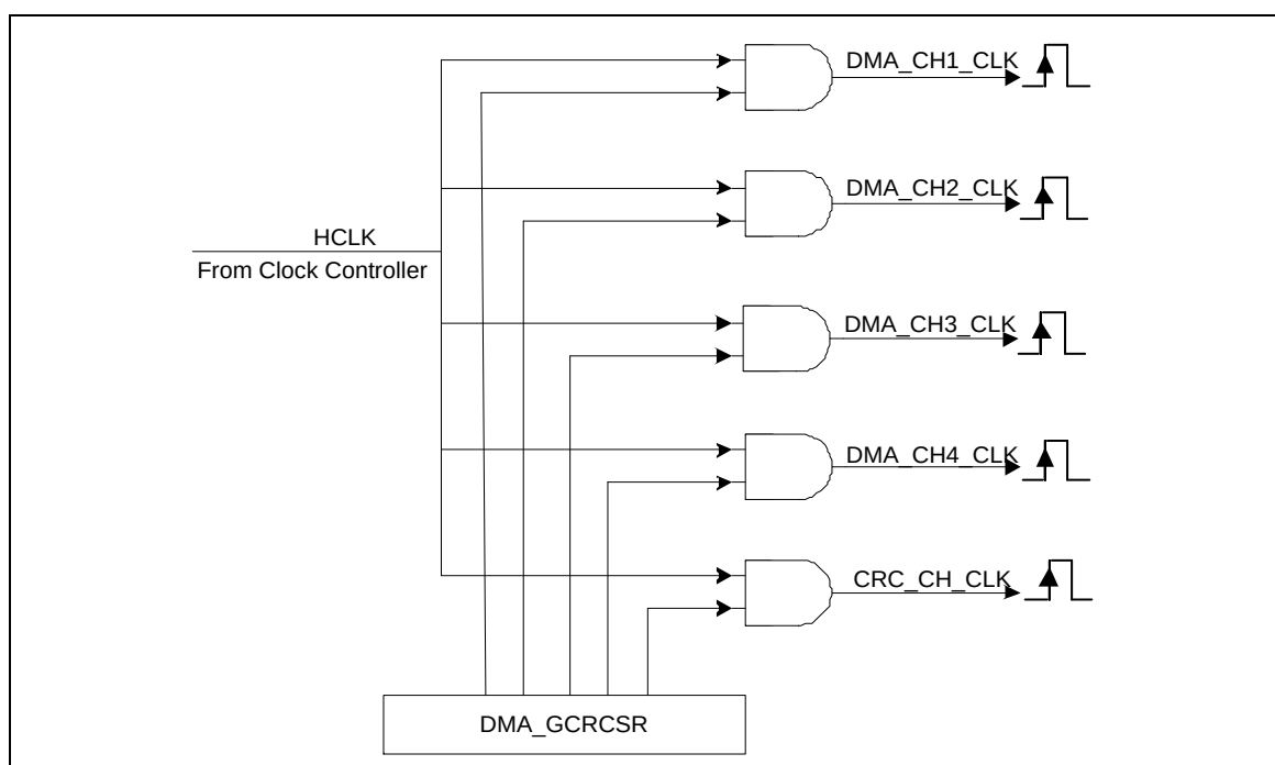
Figure 6-26 DMA Clock Control Diagram
