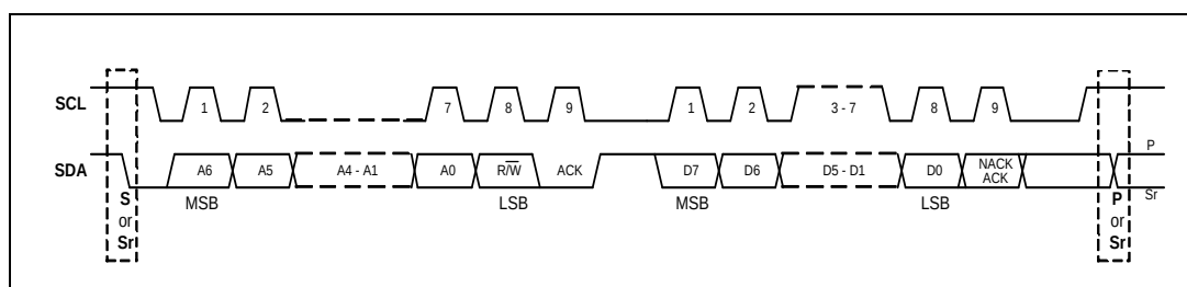
Figure 6-75 I 2 C Protocol
