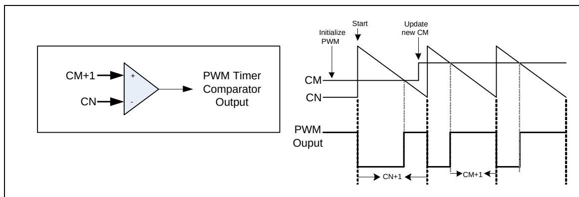
Figure 6-37 Legend of Internal Comparator Output of PWM-Timer
