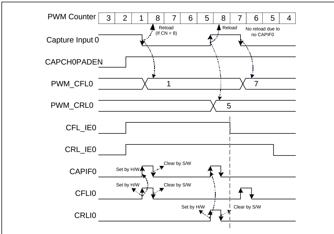
Figure 6-43 PWM Capture Operation Timing
