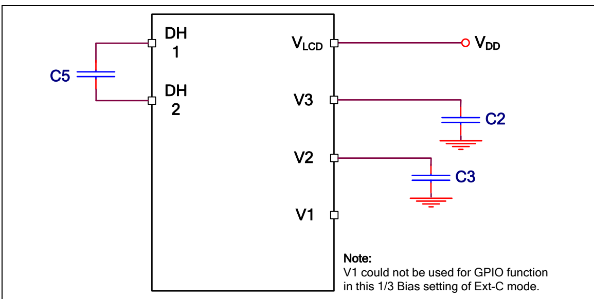
Figure 6-64 1/3 Bias (External Capacitor Ladder)
