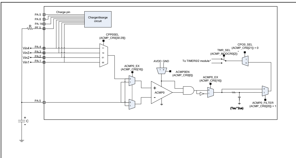
Figure 6-136 ACMP Sigma-Delta ADC Mode Reference Circuit
