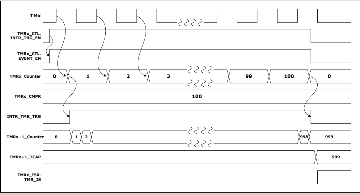
Figure 6-32 Inter-Timer Trigger Mode
