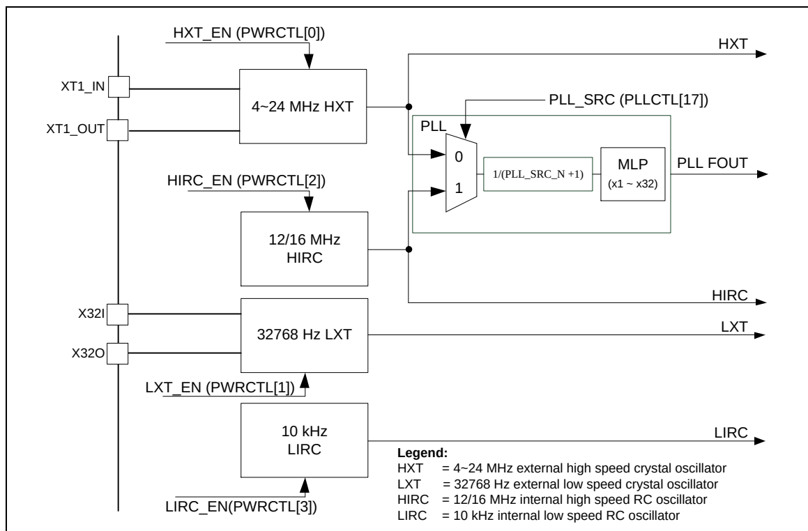
Figure 6-6 Clock Controller Block Diagram (1/3)
