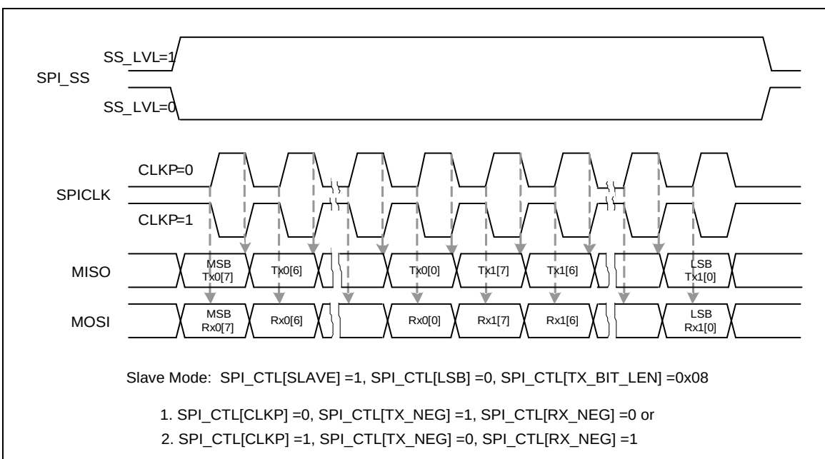
Figure 6-102 SPI Timing in Slave Mode
