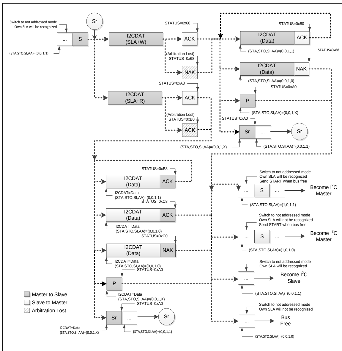
Figure 6-84 Slave Mode Control Flow
