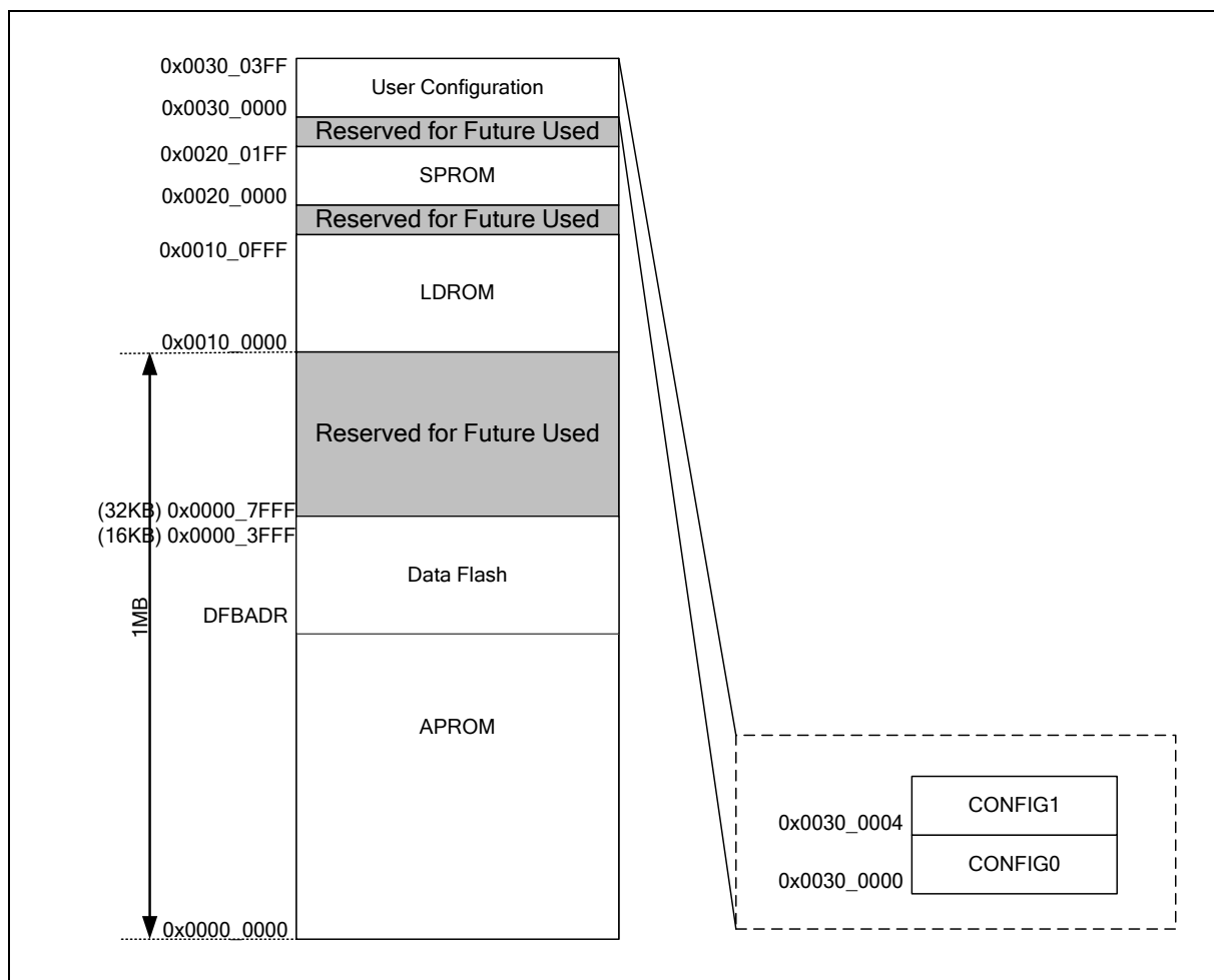
Figure 6-16 Flash Memory Organization
