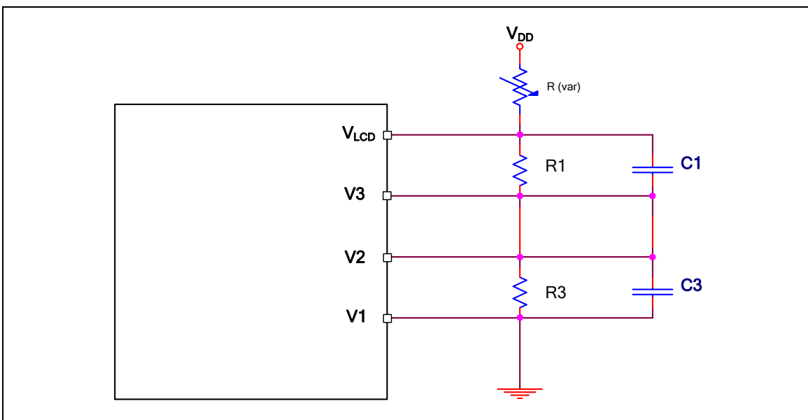
Figure 6-112 1/2 Bias (Resistor Ladder with Capacitor)
