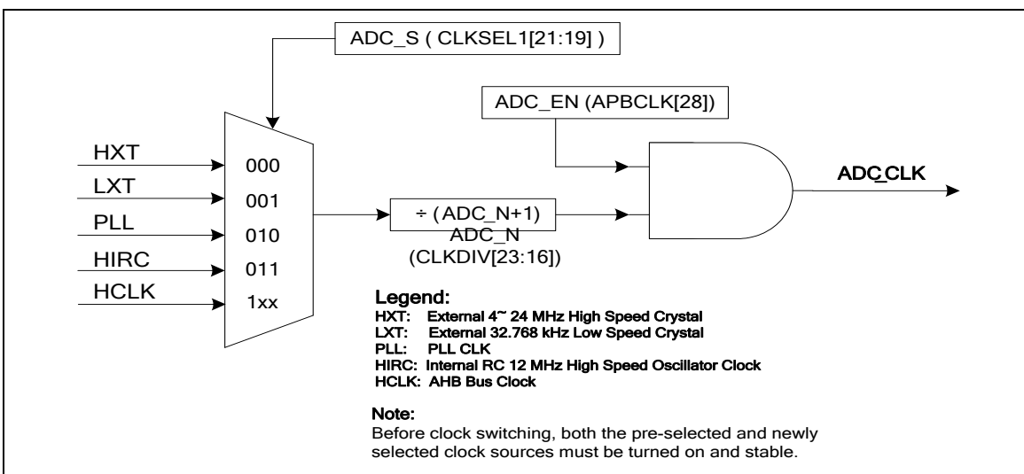
Figure 6-118 ADC Clock Control
