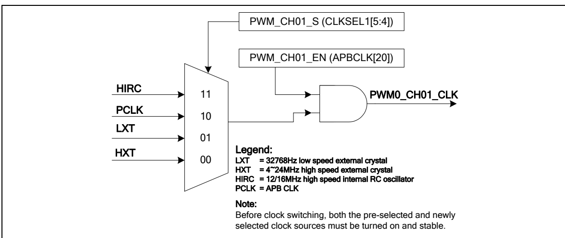
Figure 6-33 PWM Clock for Channel 0, 1
