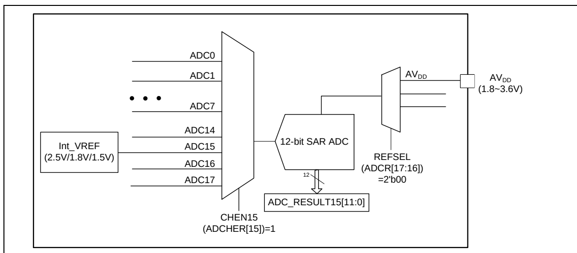
Figure 6-130 Int_VREF for Measuring AVDD Application Block Diagram
