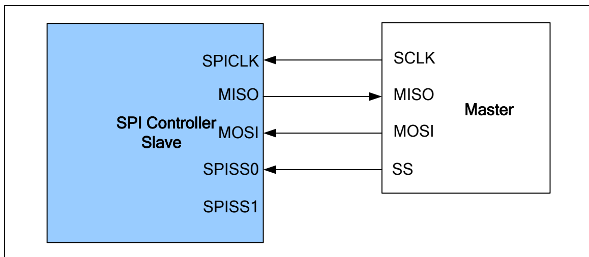
Figure 6-90 SPI Slave Mode Application Block Diagram
