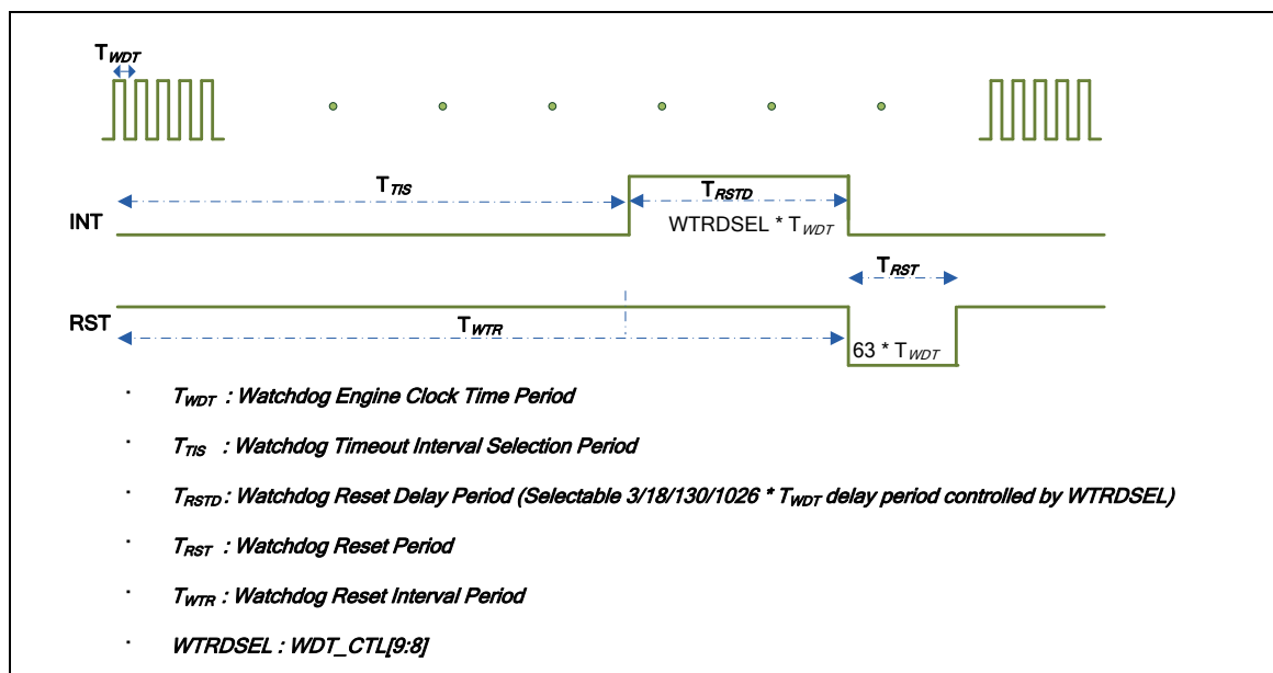
Figure 6-48 Watchdog Timing of Interrupt and Reset Signal
