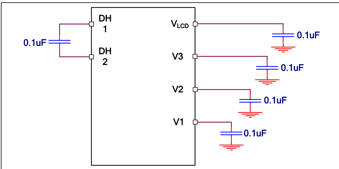
Figure 6-115 1/2 Bias (Charge Pump)
