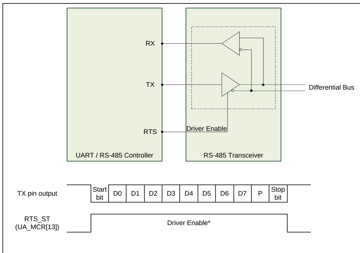
Figure 6-63 Structure of RS-485 Frame
