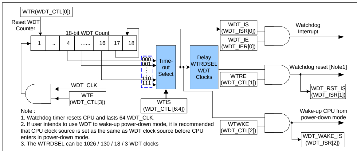
Figure 6-46 Watchdog Controller Block Diagram
