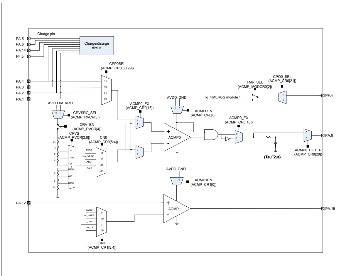
Figure 6-131 Analog Comparator Block Diagram
