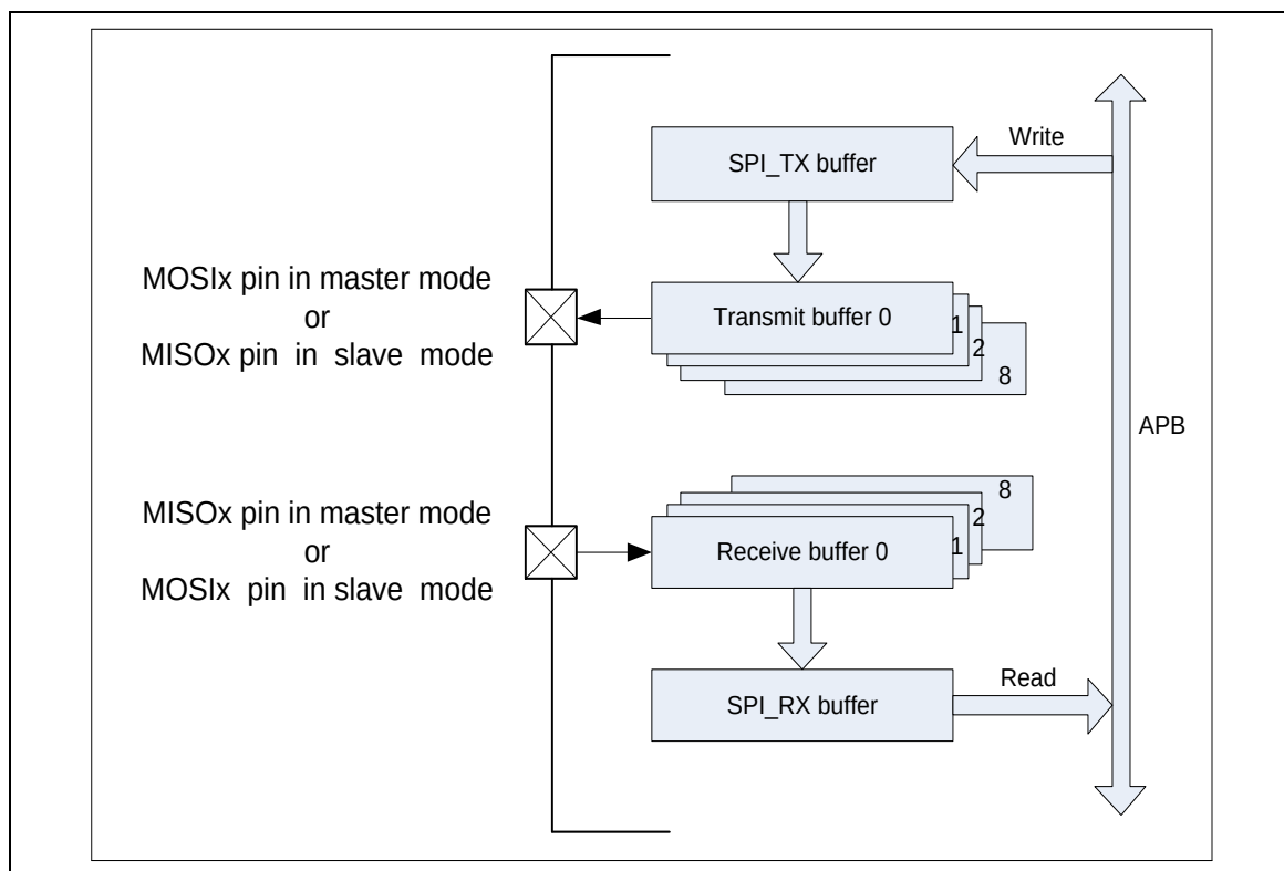
Figure 6-98 SPI FIFO Mode Control
