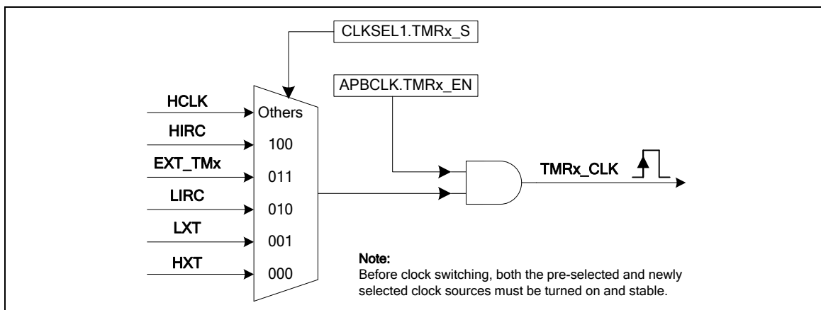
Figure 6-30 Timer Clock Controller Diagram
