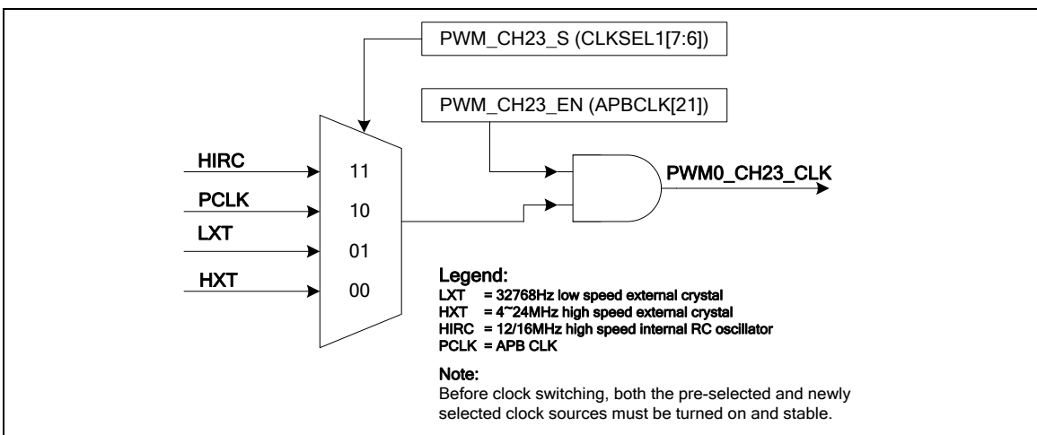
Figure 6-35 PWM Clock for Channel 2, 3
