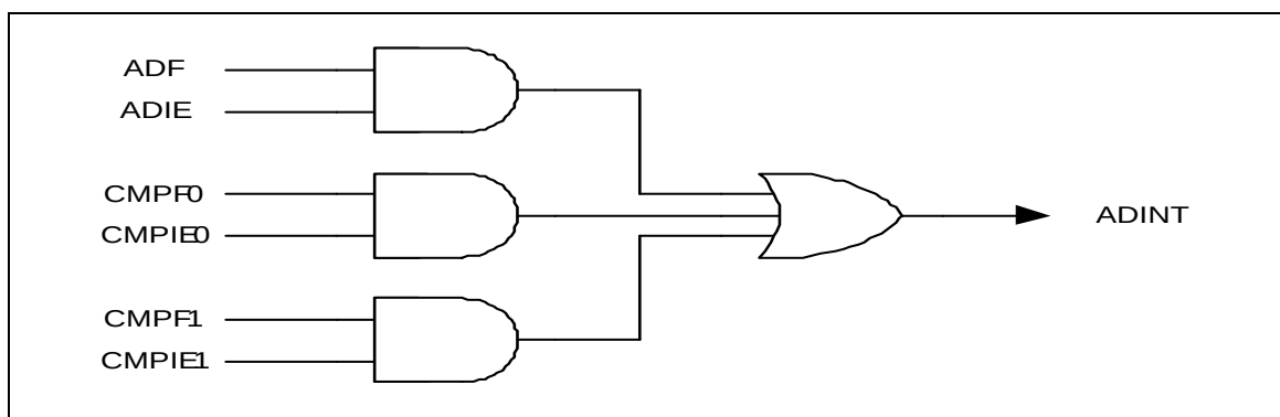
Figure 6-123 ADC Controller Interrupt
