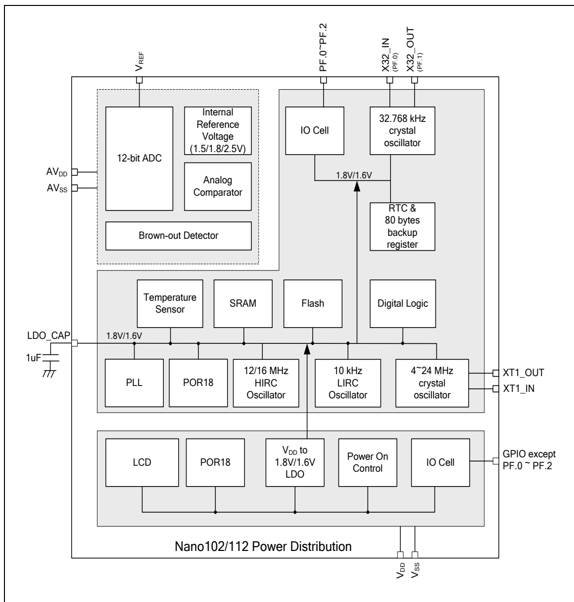
Figure 6-3 Power Architecture
