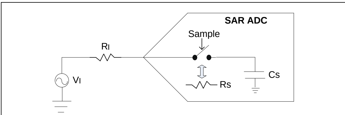
Figure 6-125 Model of Sampling Network
