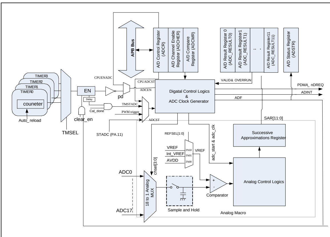
Figure 6-117 ADC Controller Block Diagram
