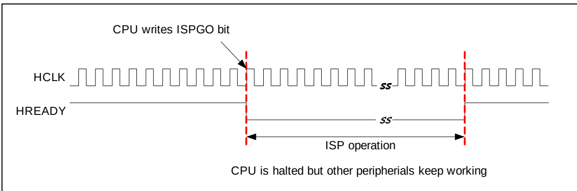
Figure 6-20 CPU Halt during ISP Operation
