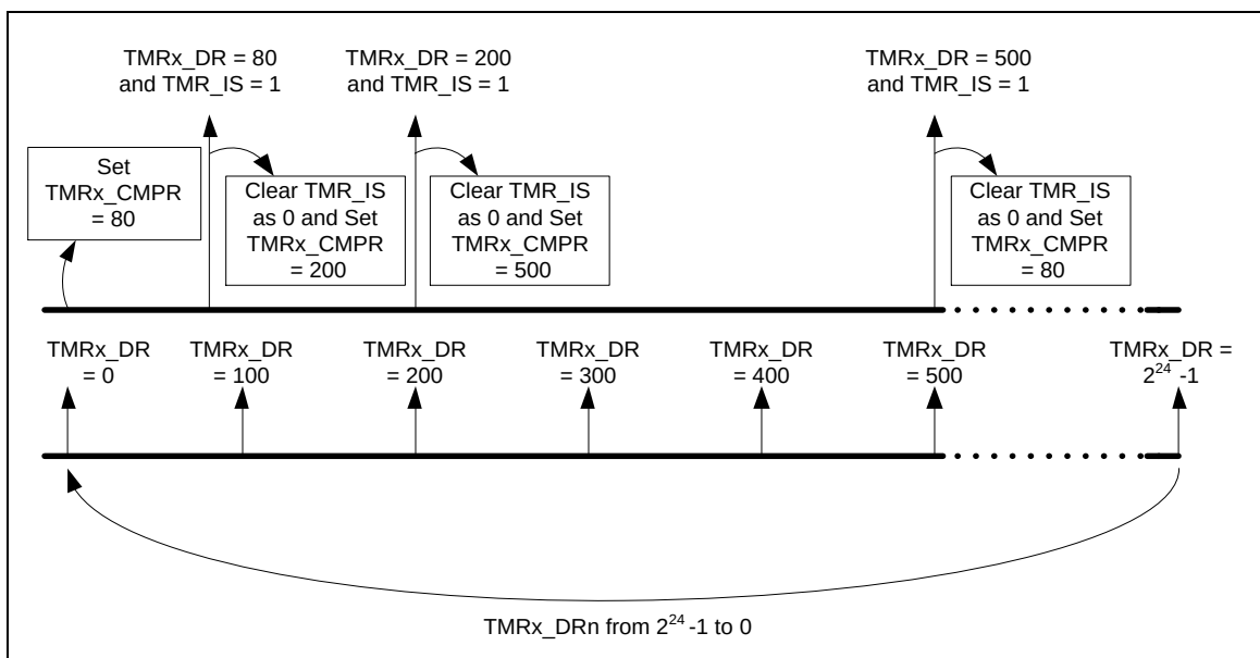
Figure 6-31 Continuous Counting Mode
