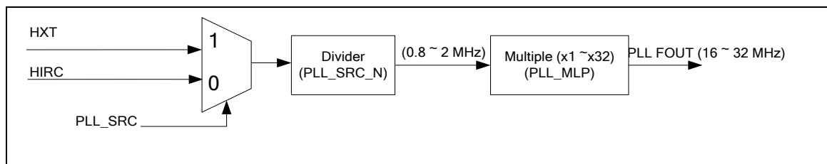
Figure 6-13 PLL Block Diagram
