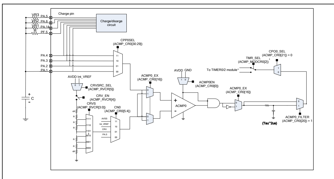
Figure 6-134 ACMP Single Slope ADC Mode Reference Circuit
