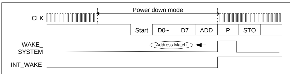
Figure 6-60 UART RS-485 AAD Mode Address Match Wake-Up
