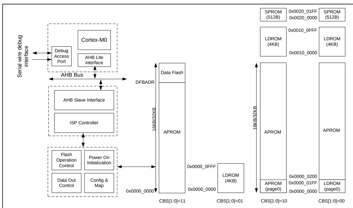
Figure 6-15 Flash Memory Controller
