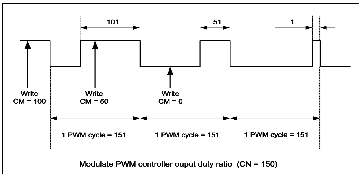
Figure 6-41 PWM Controller Output Duty Ratio
