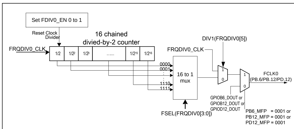
Figure 6-11 Frequency Divider0 Block Diagram
