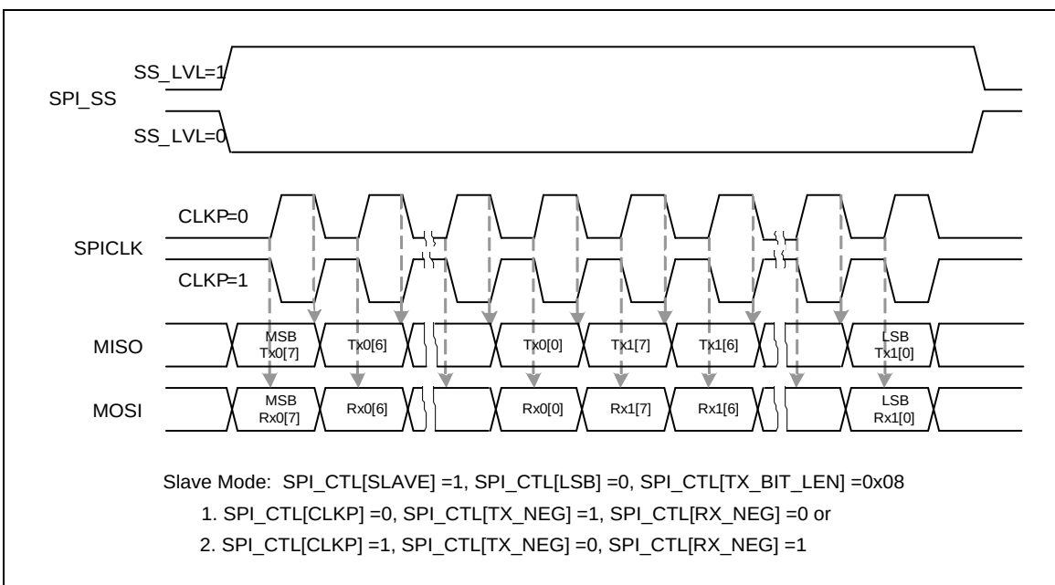
Figure 6-101 SPI Timing in Slave Mode (Alternate Phase of SPICLK & LSB = 0)
