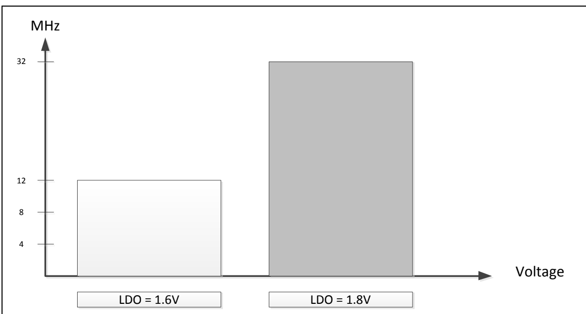
Figure 6-5 Scalable LDO and Performance
