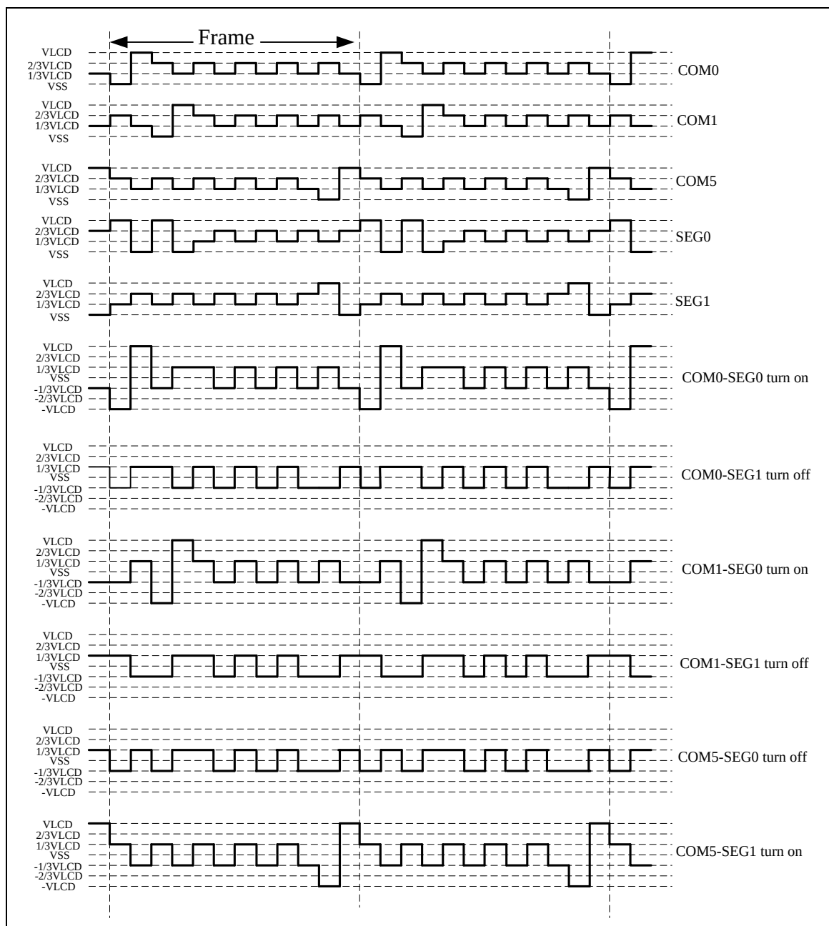
Figure 6-108 COM-SEG Signal Waveform by 1/6 Duty with 1/3 Bias
