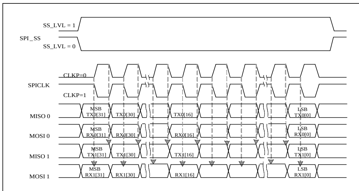
Figure 6-96 SPI 2-bit Transfer Mode Timing Diagram
