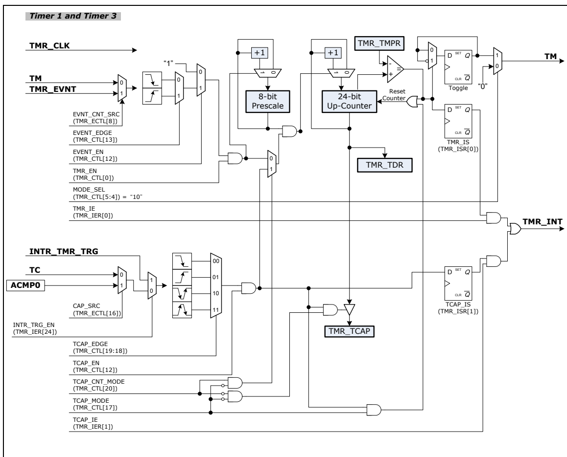
Figure 6-29 Timer 1 and Timer 3 Controller Block Diagram
