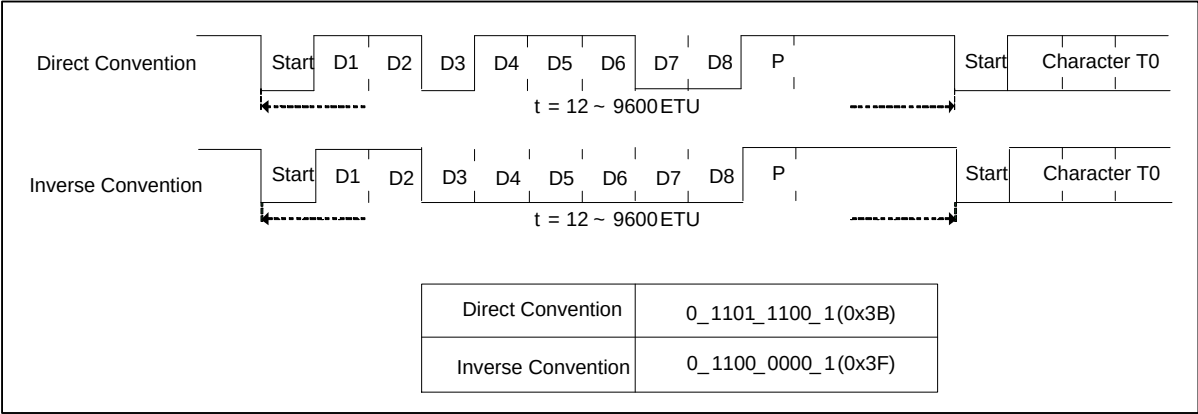
Figure 6-72 Initial Character TS
