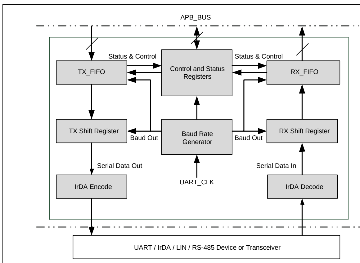
Figure 6-53 UART Block Diagram
