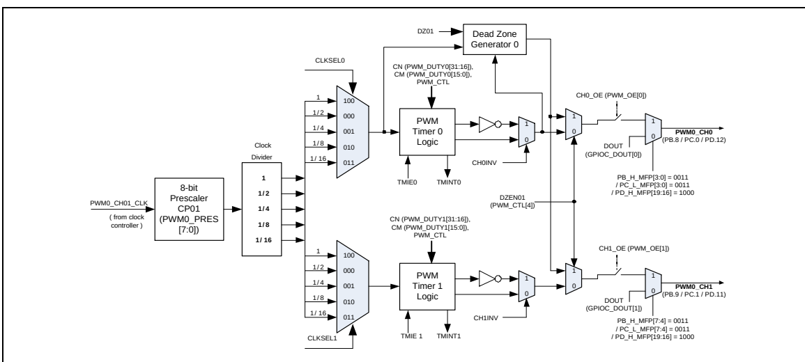
Figure 6-34 PWM Generator for Channel 0, 1
