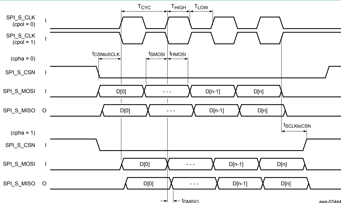
Figure 3. SPI slave timing
