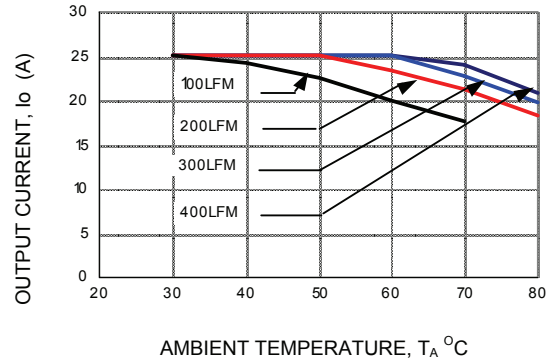
Figure 18. Derating Output Current versus Local Ambient Temperature and Airflow ( V_{in} = 12Vdc , V_o = 5.0 Vdc ).
