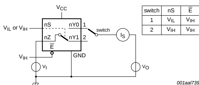
Fig 5. Test circuit for measuring OFF-state leakage current
