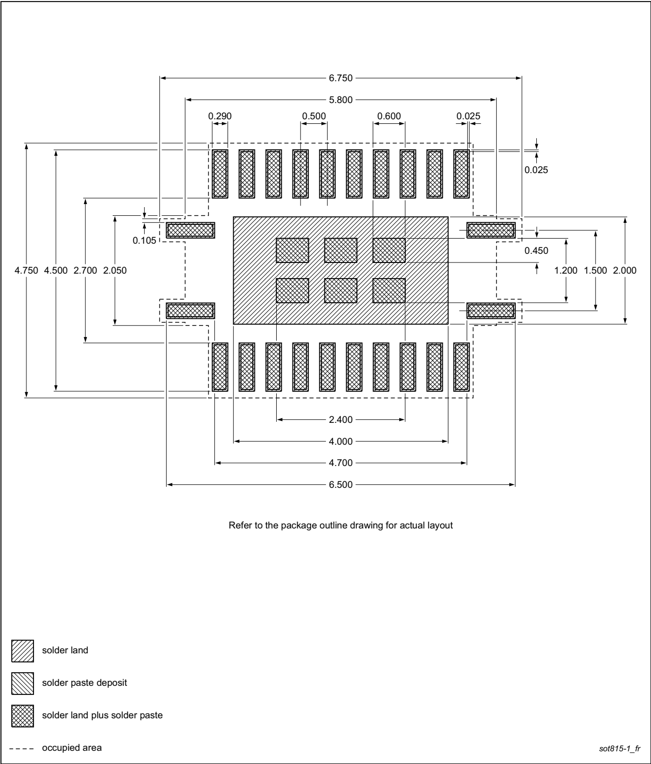
Footprint information for reflow soldering of DHVQFN24 package
