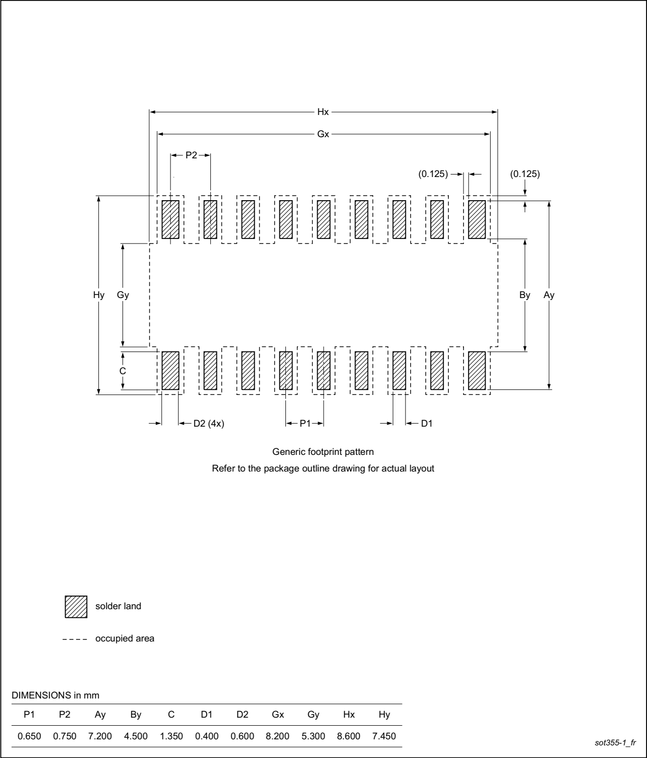
Fig 27. PCB footprint for SOT355-1 (TSSOP24); reflow soldering
