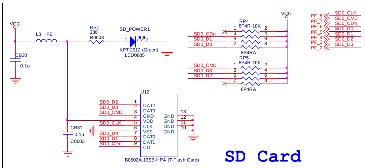
Figure 4-13 MicroSD Card Circuit
