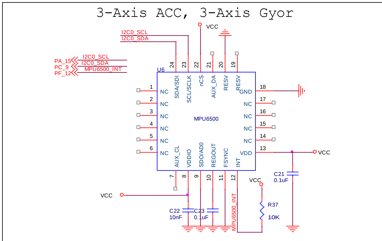
Figure 4-20 MPU6500 Circuit
