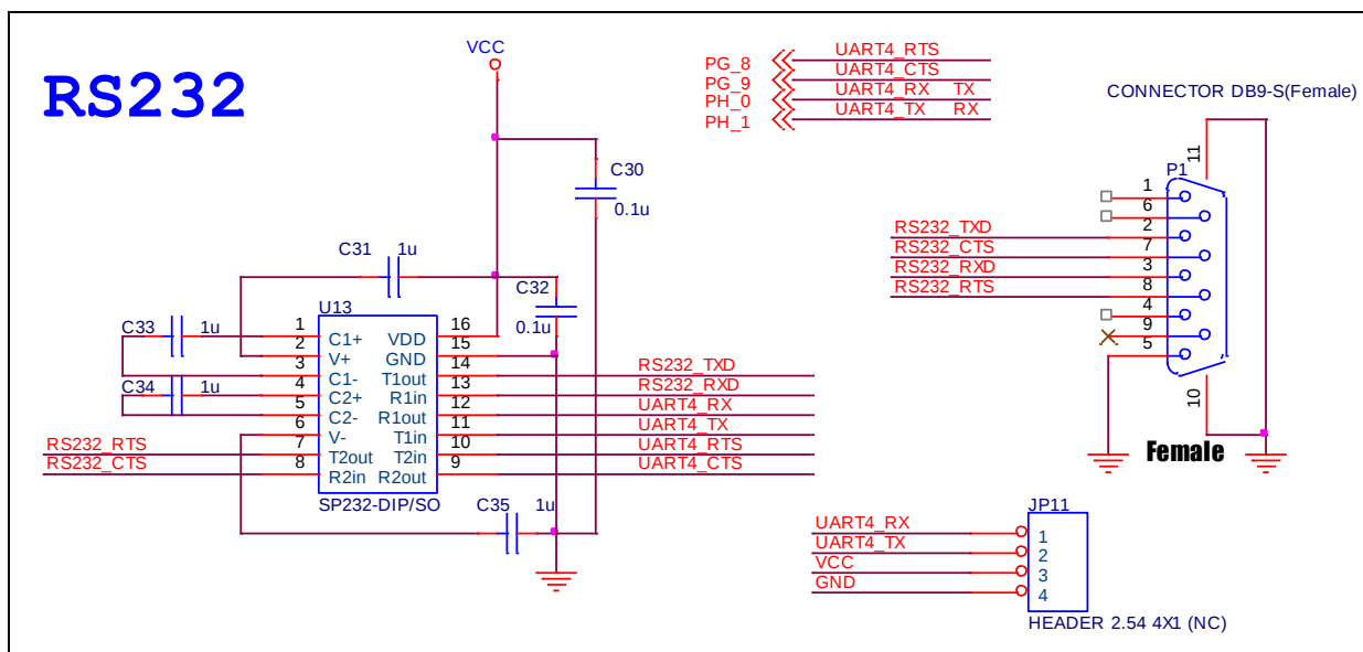
Figure 4-12 RS232 Circuit
