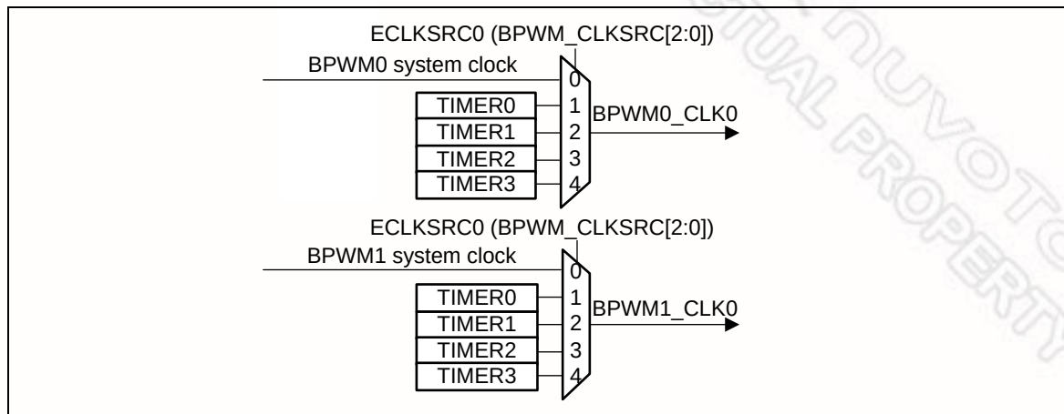
Figure 6-59 BPWM Clock Source Control
