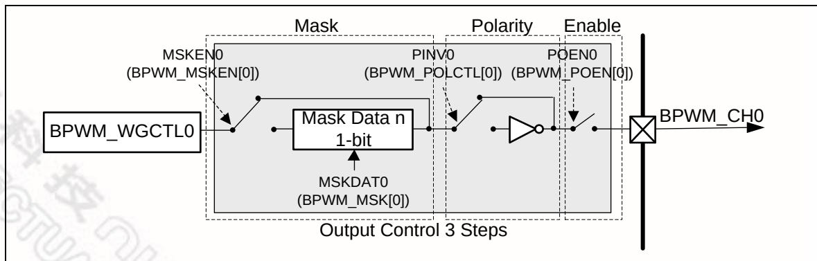
Figure 6-72 BPWM_CH0 Output Control 3 Steps
