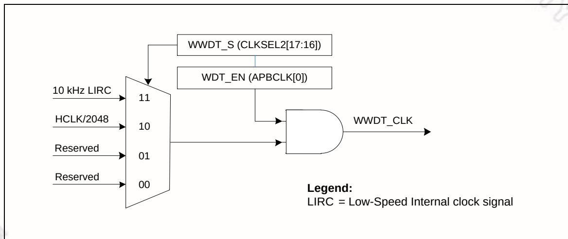
Figure 6-83 Window Watchdog Timer Clock Control
