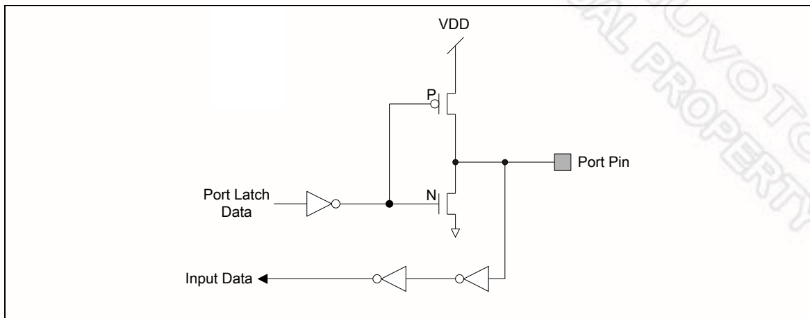
Figure 6-17 Push-Pull Output
