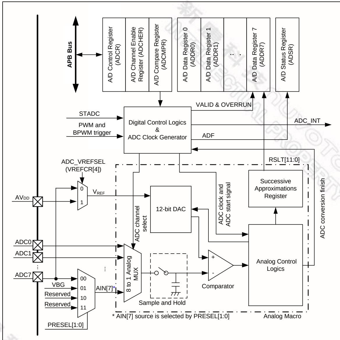
Figure 6-149 ADC Controller Block Diagram
