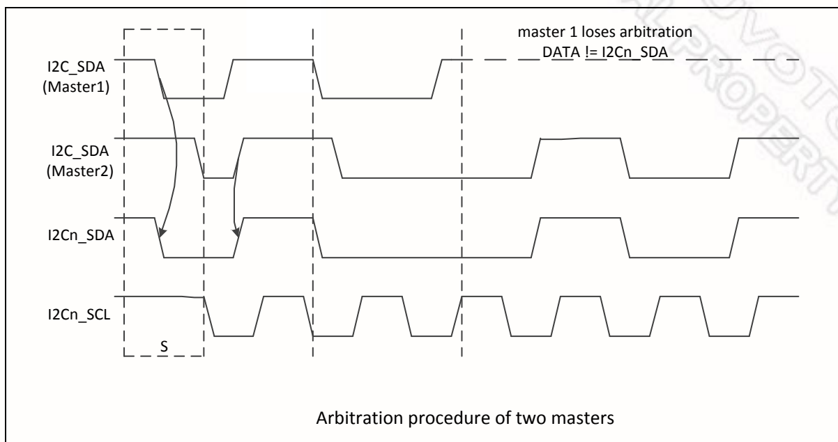
Figure 6-119 Arbitration Lost
