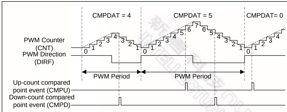
Figure 6-32 PWM CMPDAT Events in Up-Down Counter Type
