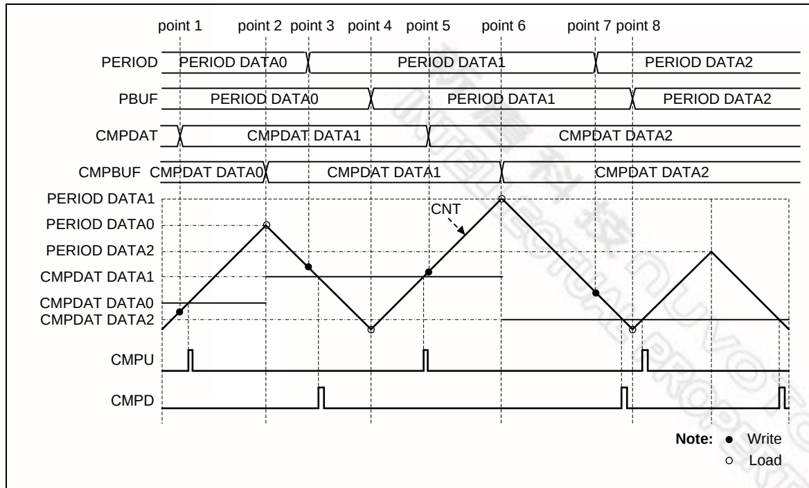
Figure 6-69 Center Loading Mode with Up-Down-Counter Type
