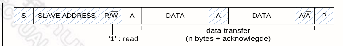
Figure 6-113 Master Reads Data from Slave
