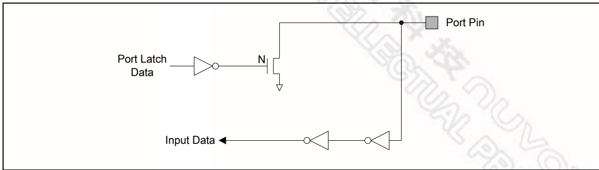
Figure 6-18 Open-Drain Output
