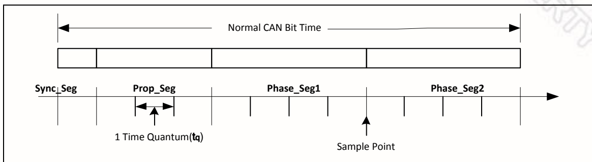
Figure 6-144 Bit Timing
