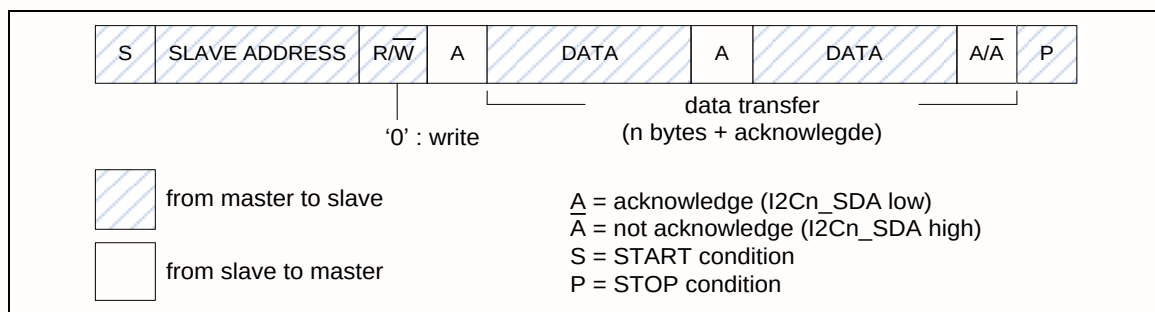
Figure 6-112 Master Transmits Data to Slave
