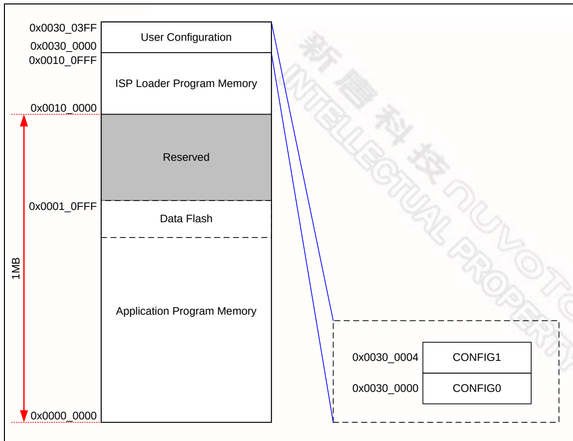
Figure 6-12 Flash Memory Organization (DFVSEN = 0)
