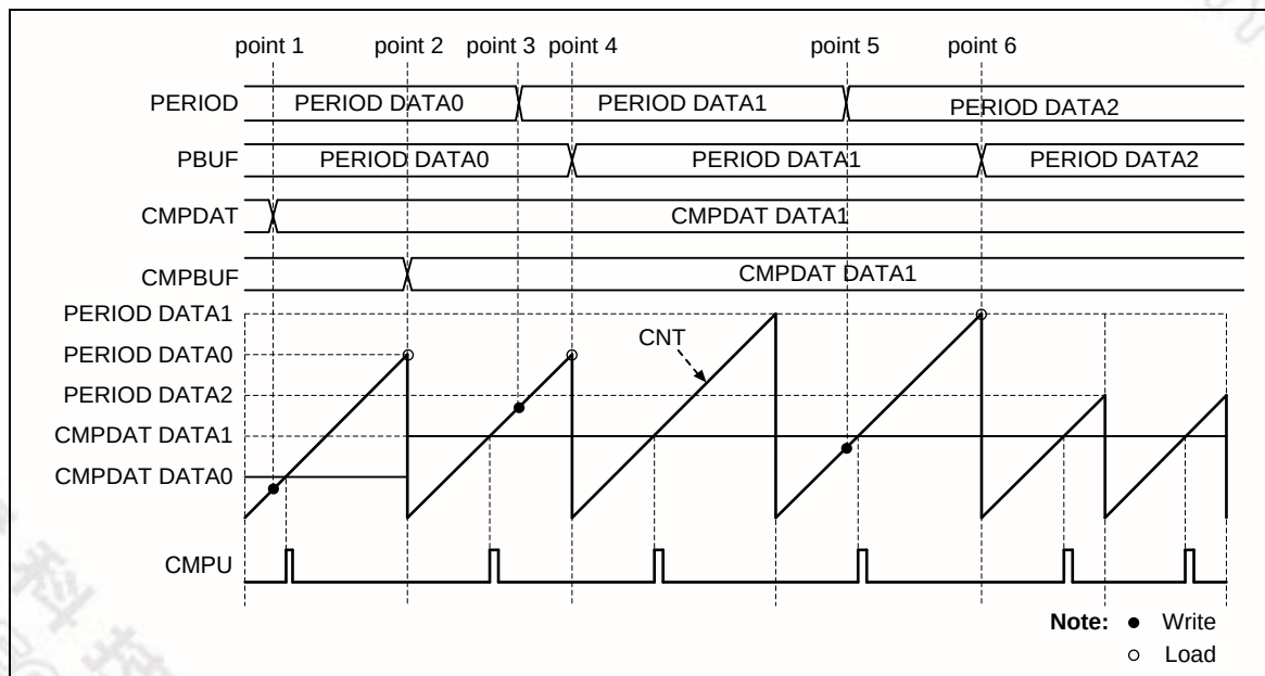
Figure 6-34 Period Loading Mode with Up-Counter Type
