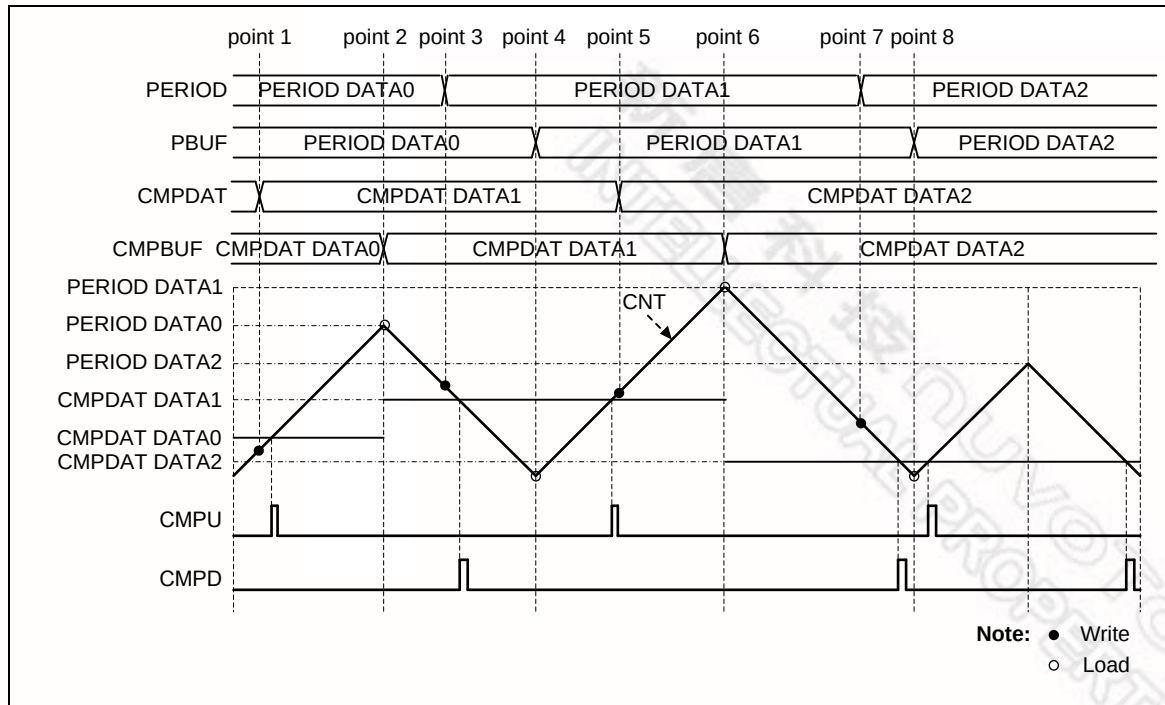
Figure 6-36 Center Loading Mode with Up-Down-Counter Type
