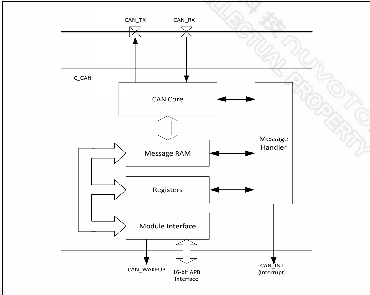
Figure 6-138 CAN Peripheral Block Diagram
