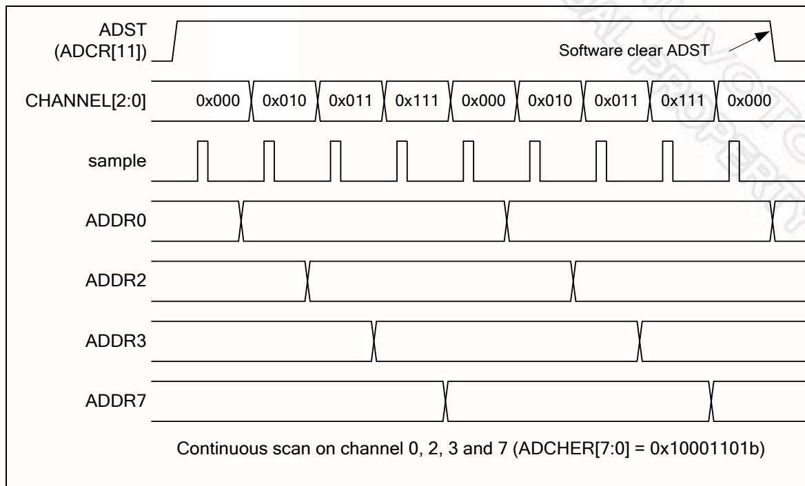
Figure 6-153 Continuous Scan on Enabled Channels Timing Diagram
