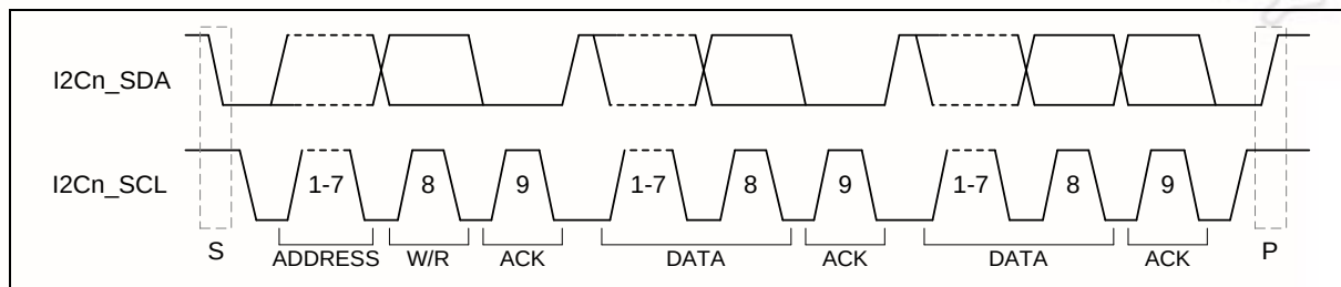
Figure 6-108 I 2 C Protocol
