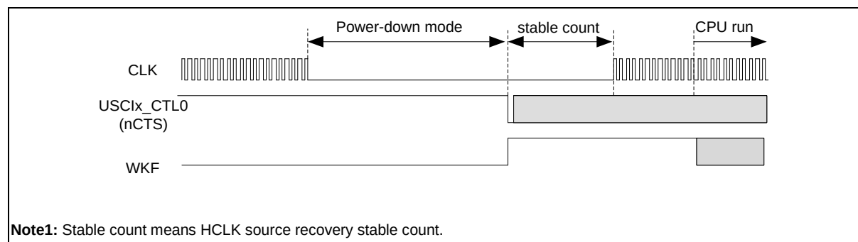
Figure 6.20-8 nCTS Wake-Up Case 2
