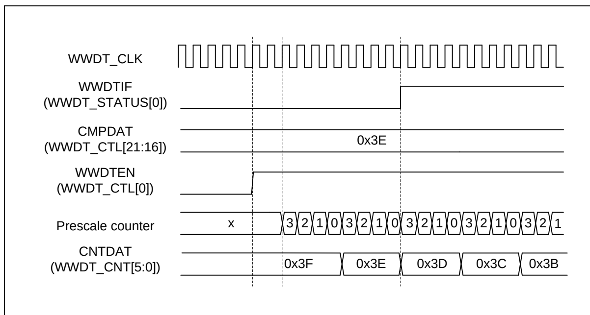
Figure 6.25-3 WWDT Compare Match Interrupt when CMPDAT is 0x3E
