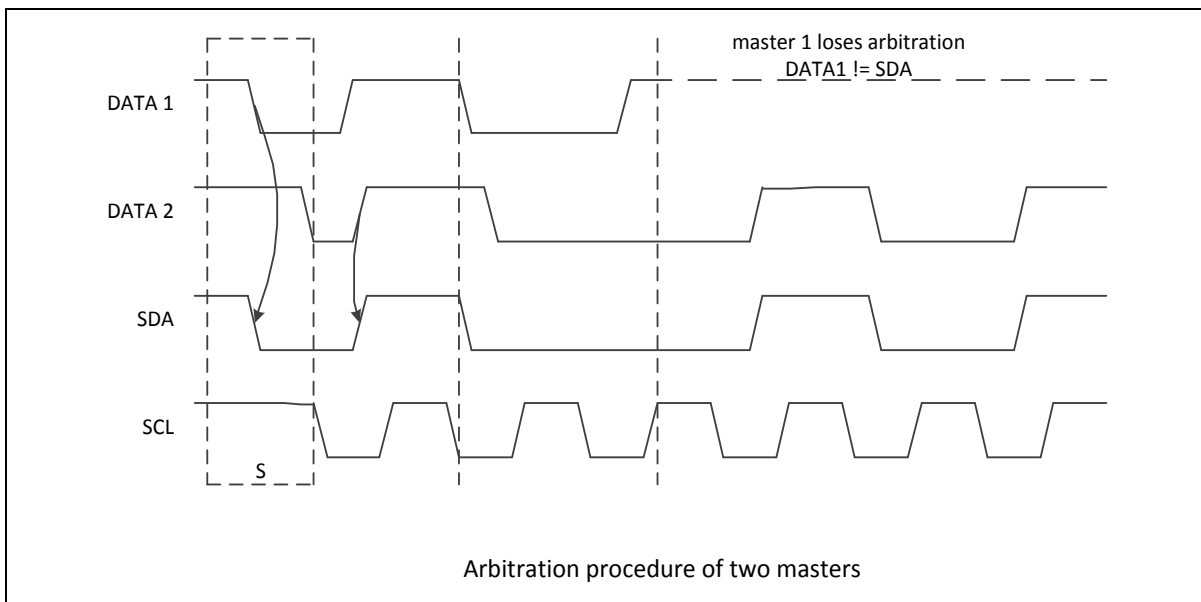
Figure 6.11-14 Arbitration Lost
