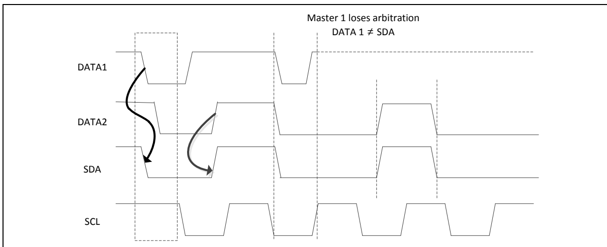
Figure 6.22-7 Arbitration Lost
