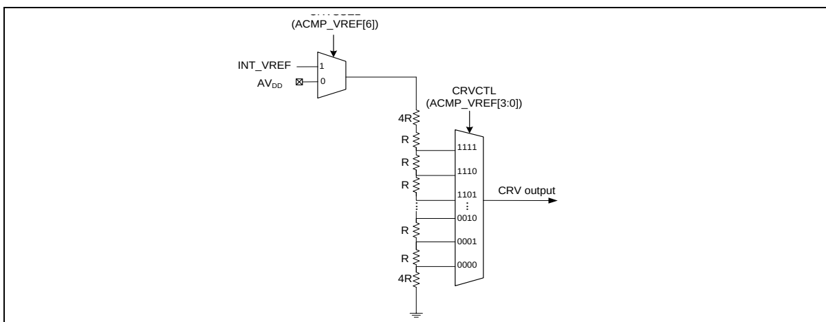
Figure 6.5-6 Comparator Reference Voltage Block Diagram
