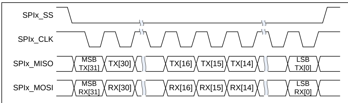
Figure 6.16-532-Bit in One Transaction
