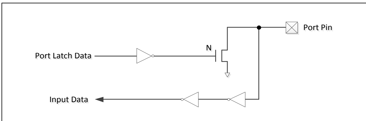
Figure 6.9-3 Open-Drain Output
