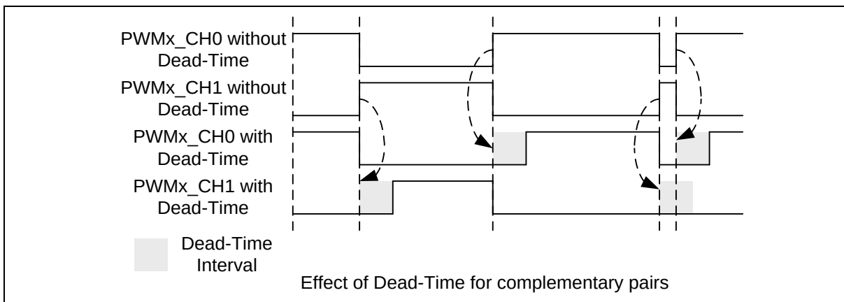
Figure 6.13-27 Dead-Time Insertion
