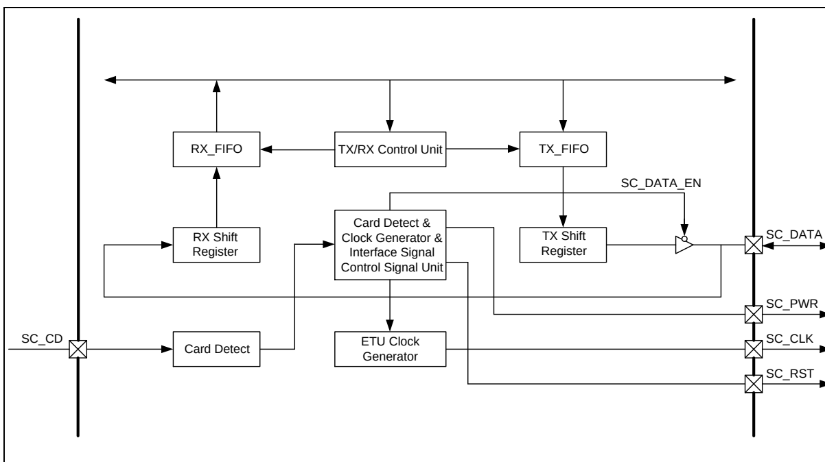
Figure 6.15-2 SC Controller Block Diagram
