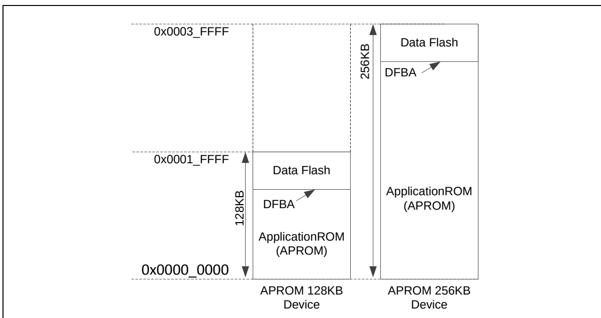
Figure 6.4-2 Data Flash
