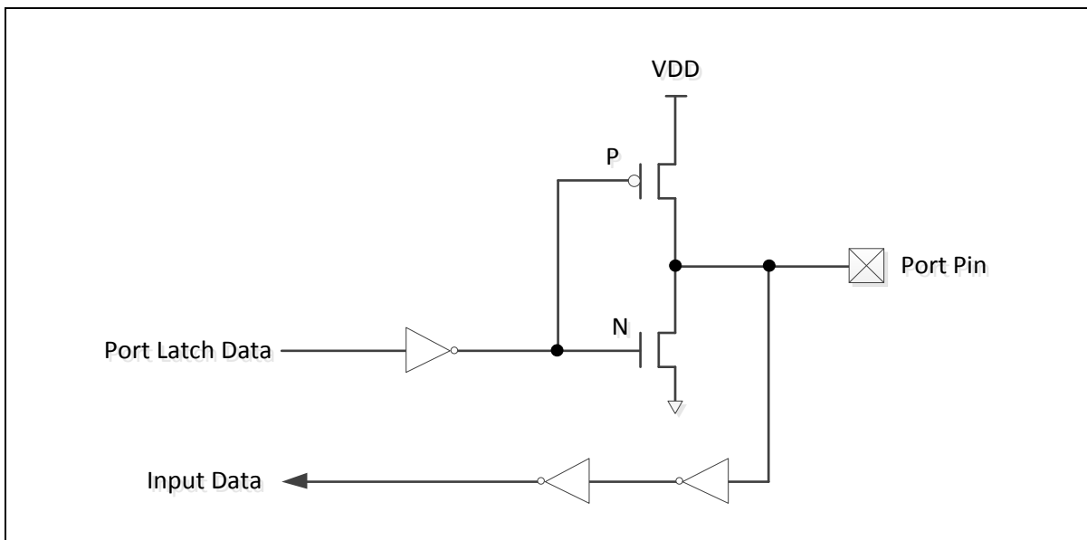
Figure 6.9-2 Push-Pull Output
