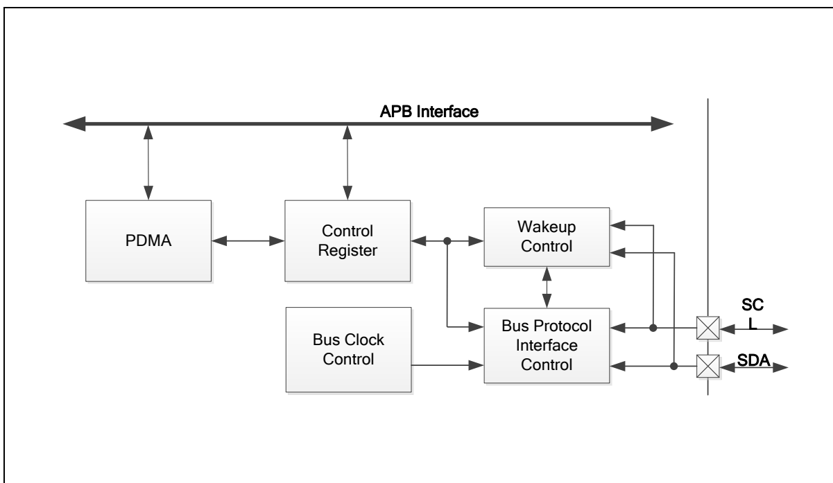
Figure 6.11-1 I²C Controller Block Diagram
