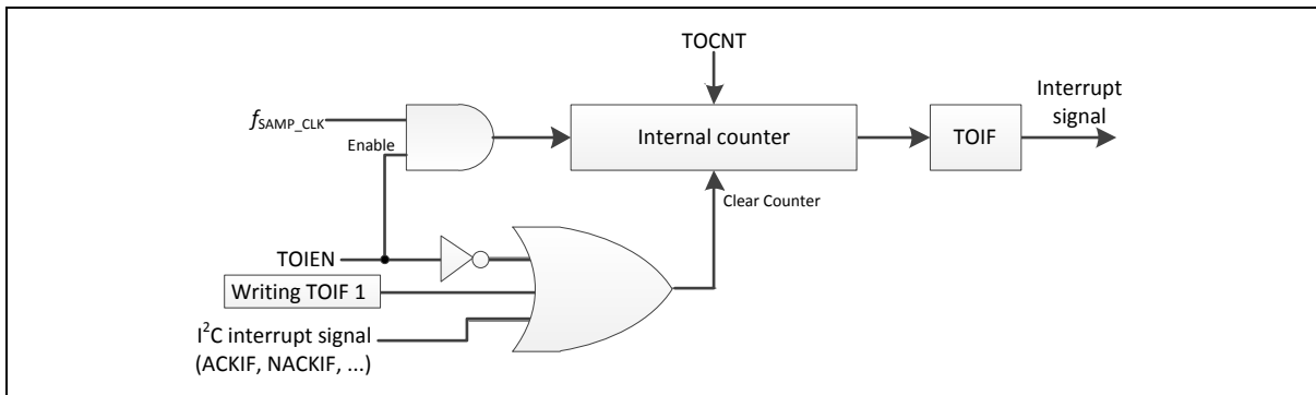
Figure 6.22-19 I²C Time-out Count Block Diagram
