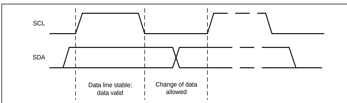
Figure 6.11-5 Bit Transfer on the I 2 C Bus
