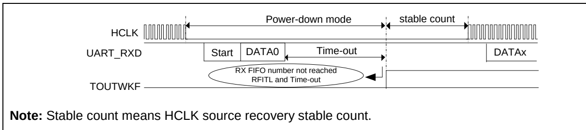
Figure 6.23-10 UART Received Data FIFO Threshold Time-out Wake-up
