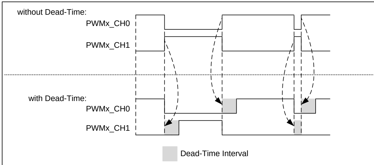
Figure 6.17-26 Dead-Time Insertion
