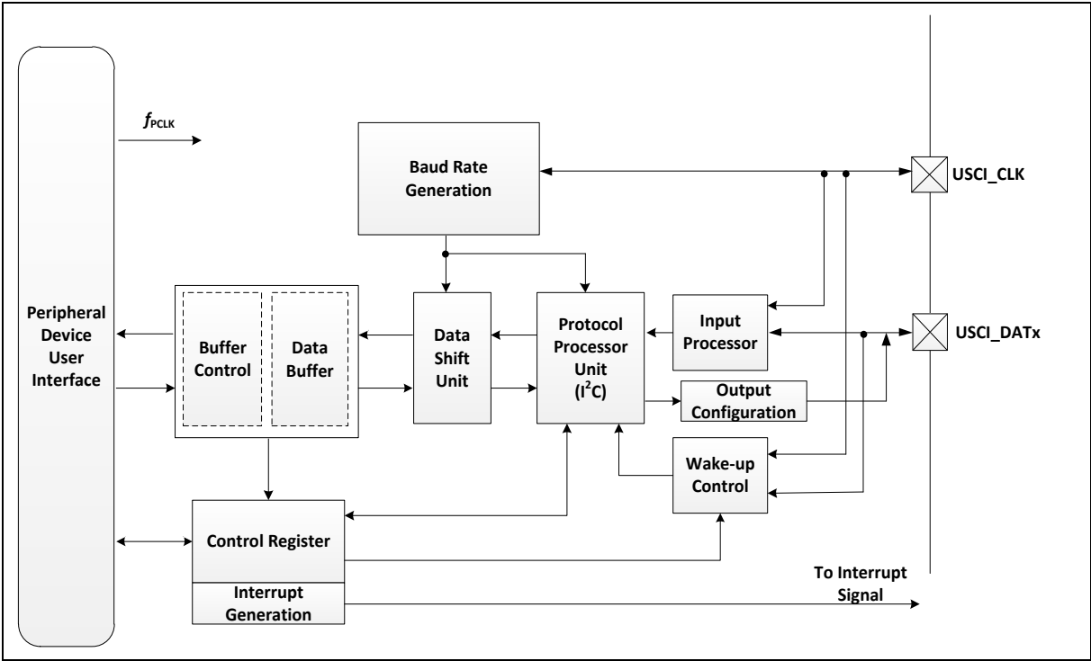
Figure 6.22-2 USCI I²C Mode Block Diagram
