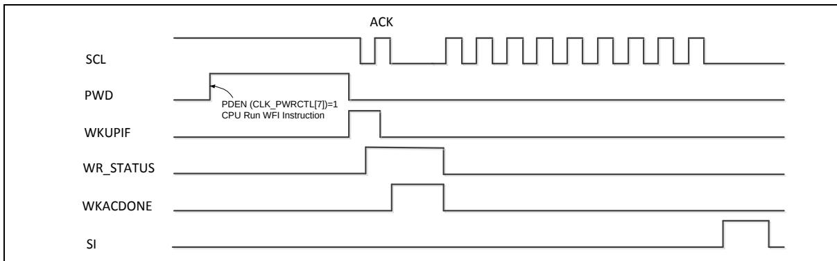
Figure 6.11-21 I²C Wake-Up Related Signals Waveform
