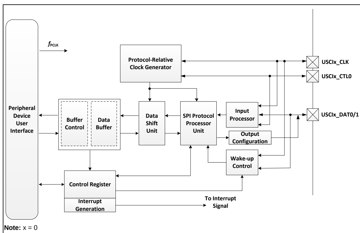
Figure 6.14-3 Block Diagram
