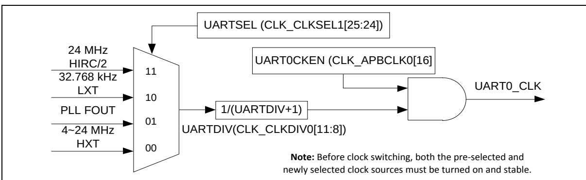
Figure 6.16-1 UART Clock Control Diagram
