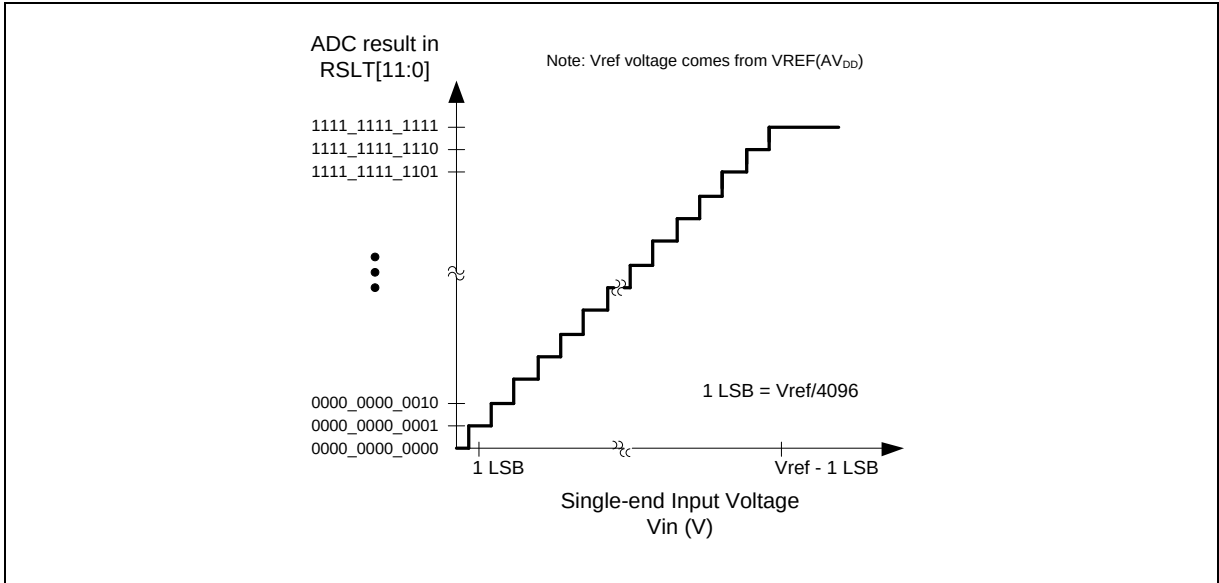
Figure 6.20-9 Conversion Result Mapping Diagram of ADC Single-end Input
