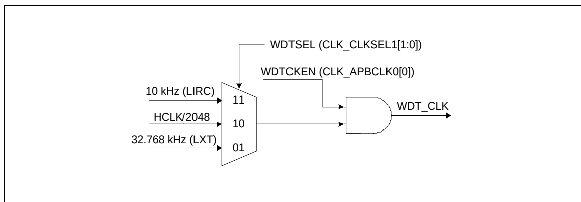
Figure 6.10-2 Watchdog Timer Clock Control
