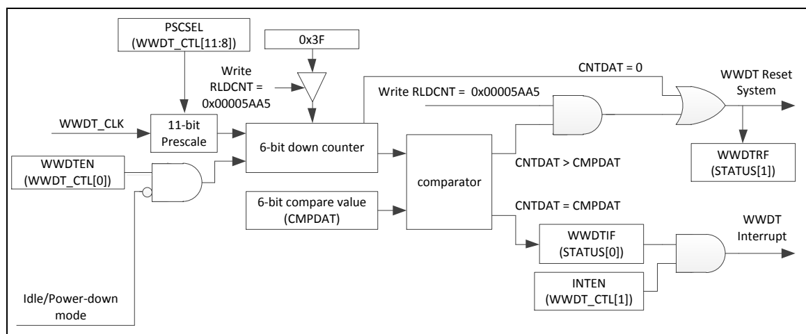
Figure 6.11-1 WWDT Block Diagram
