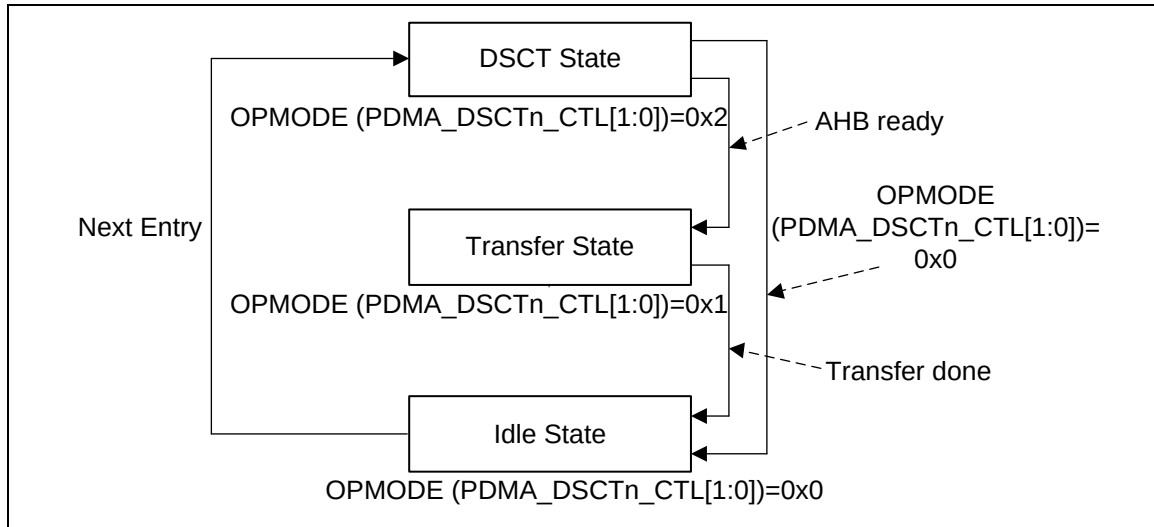
Figure 6.6-6 Scatter-Gather Mode Finite State Machine
