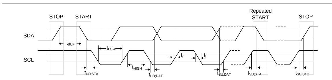
Figure 6.17-2 I²C Bus Timing
