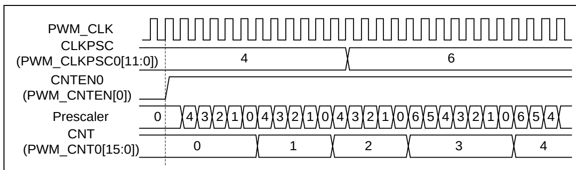
Figure 6.9-6 PWM_CH0 CLKPSC waveform
