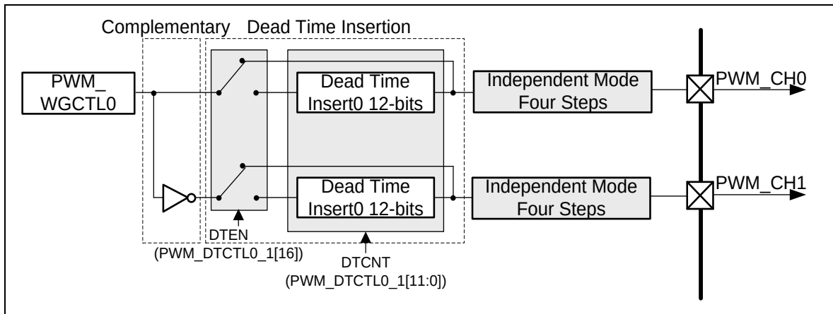
Figure 6.9-20 PWM_CH0 and PWM_CH1 Output Control in Complementary Mode
