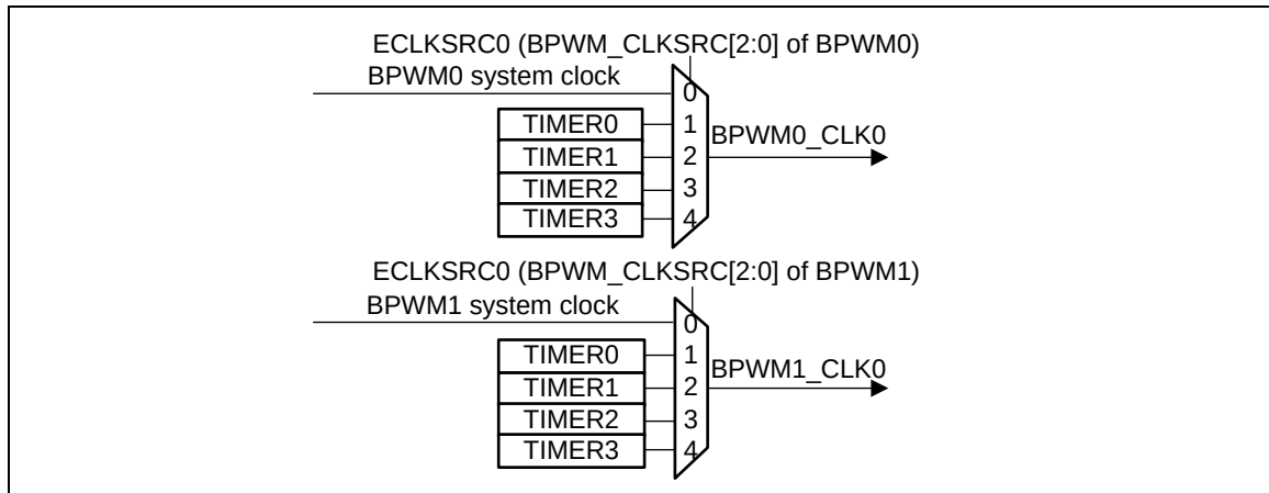
Figure 6.8-3 BPWM Clock Source Control
