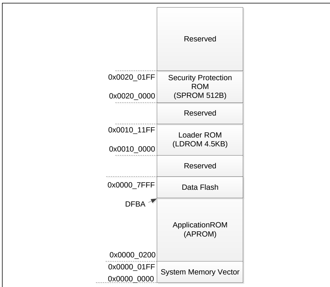
Figure 6.4-5 System Memory Map with IAP Mode
