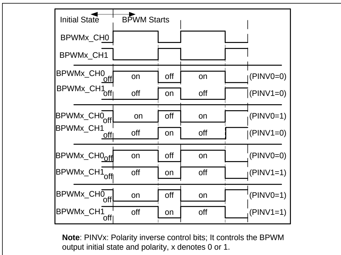
Figure 6.8-18 Initial State and Polarity Control
