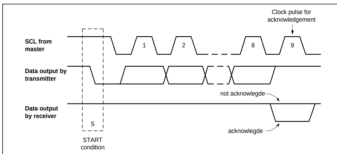
Figure 6.17-6 Acknowledge on the I 2 C Bus
