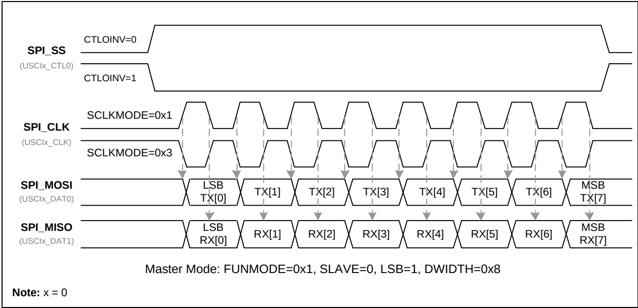
Figure 6.14-17 SPI Timing in Master Mode (Alternate Phase of Serial Bus Clock)
