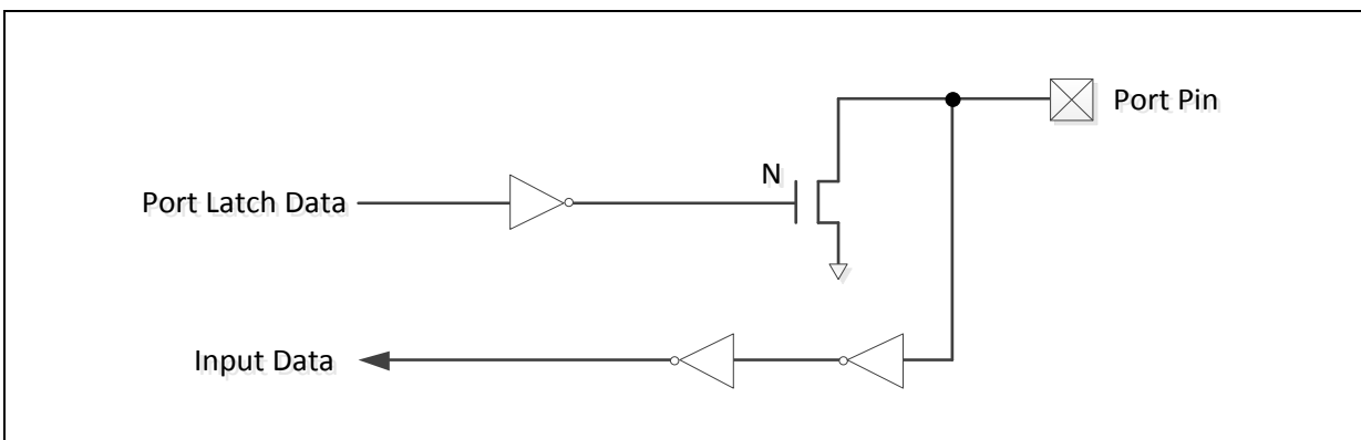
Figure 6.5-3 Open-Drain Output
