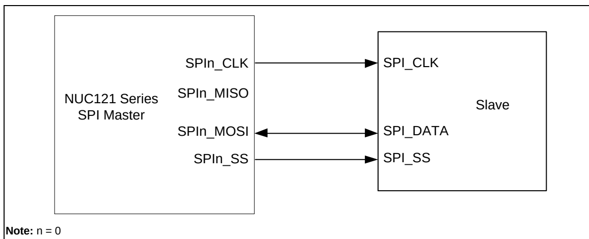
Figure 6.18-10 SPI Half-Duplex Master Mode Application Block Diagram
