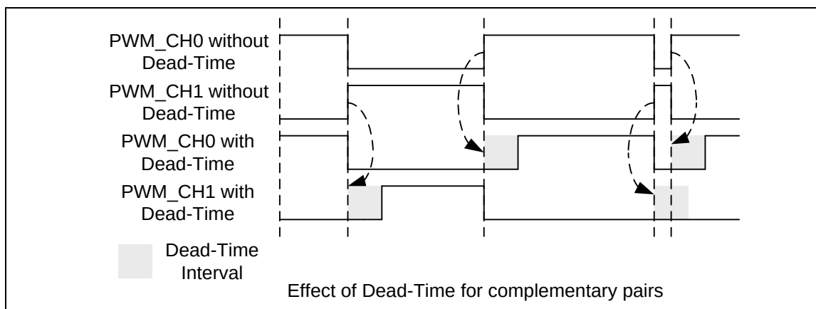
Figure 6.9-21 Dead-Time Insertion
