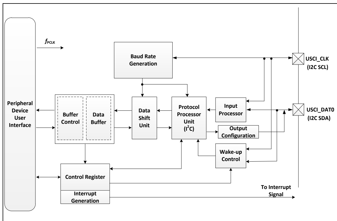
Figure 6.15-2 Block Diagram
