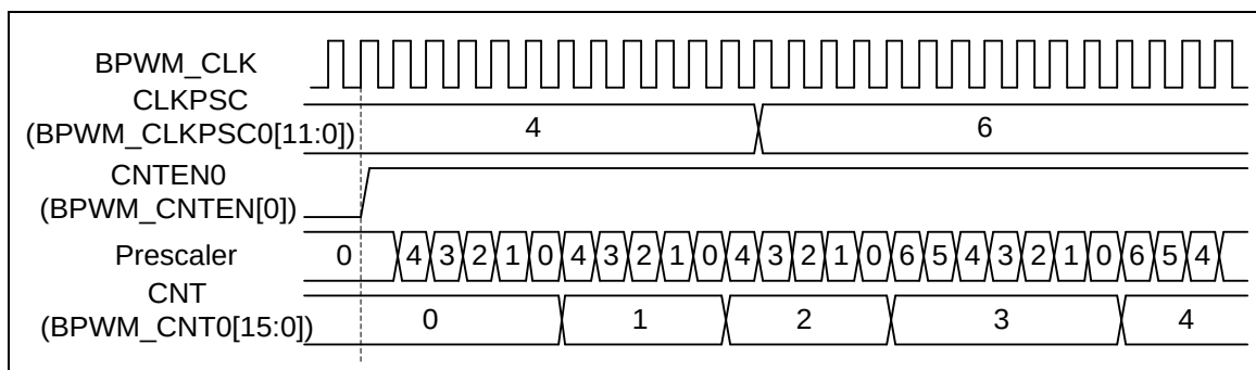
Figure 6.8-5 BPWM_CH0 CLKPSC waveform
