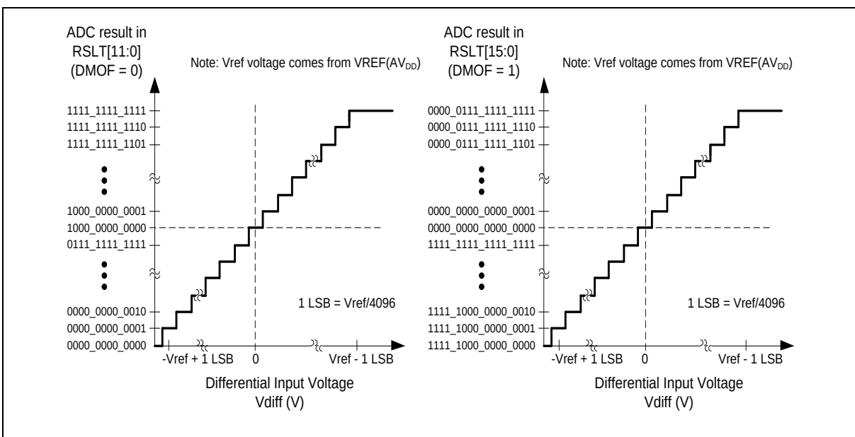
Figure 6.20-10 Conversion Result Mapping Diagram of ADC Differential Input
