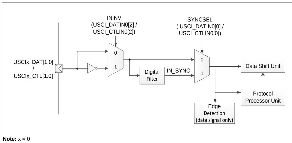
Figure 6.12-2 Input Conditioning for USC1x_DAT[1:0] and USC1x_CTL[1:0]
