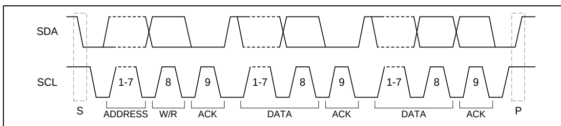
Figure 6.17-3 I²C Protocol
