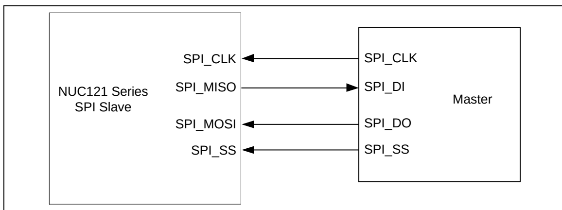
Figure 6.18-4 SPI Full-Duplex Slave Mode Application Block Diagram
