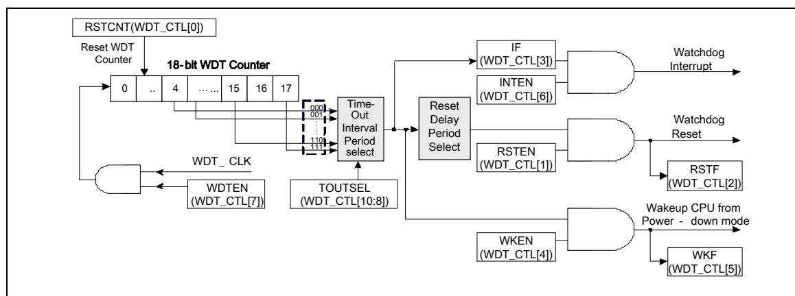
Figure 6.10-1 Watchdog Timer Block Diagram
