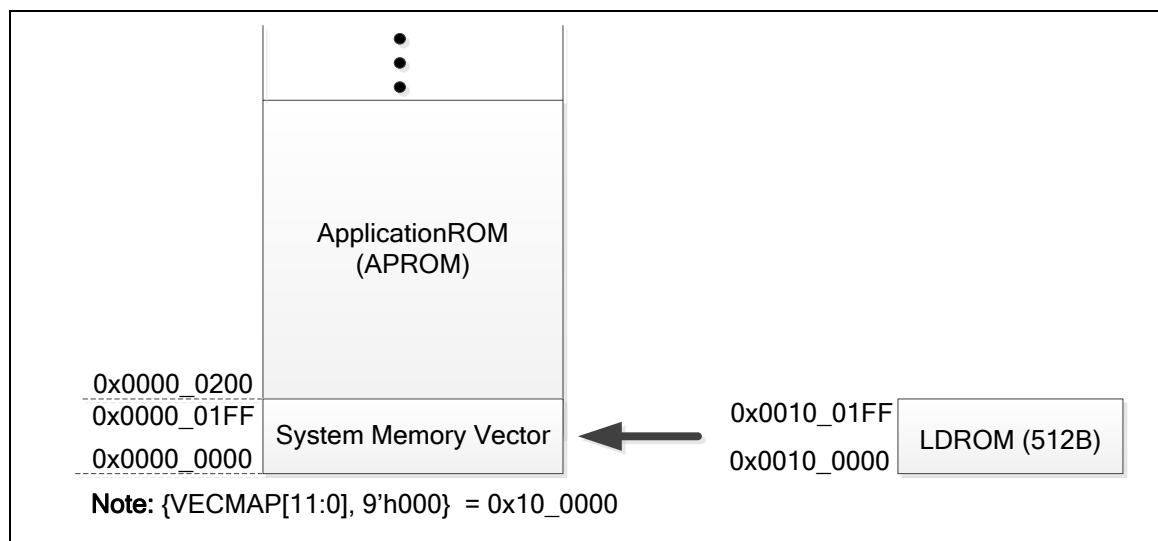
Figure 6.4-6 LDROM with IAP Mode
