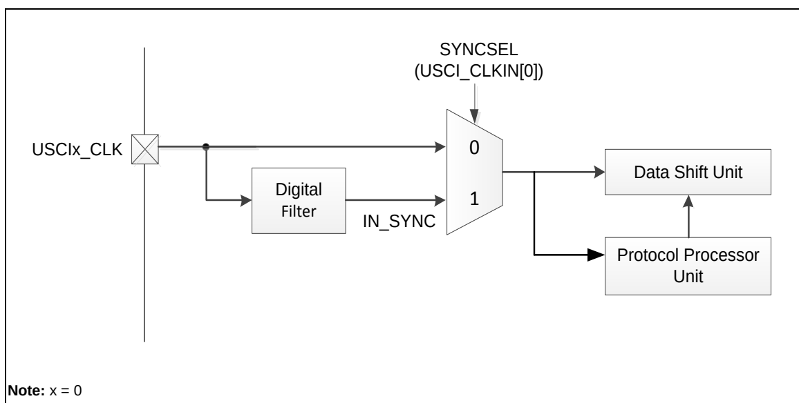
Figure 6.12-3 Input Conditioning for USC1x_CLK
