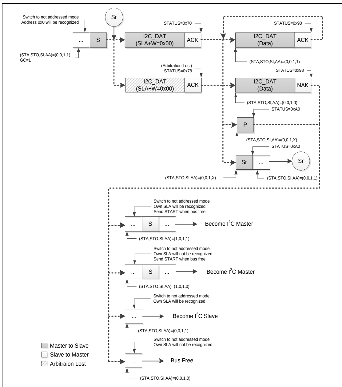
Figure 6.17-13 GC Mode
