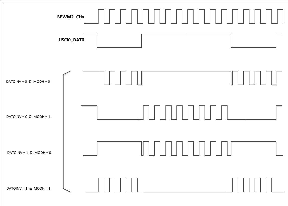
Figure 6.2-11 USCIO_DAT0 Modulated with PWM Channel
