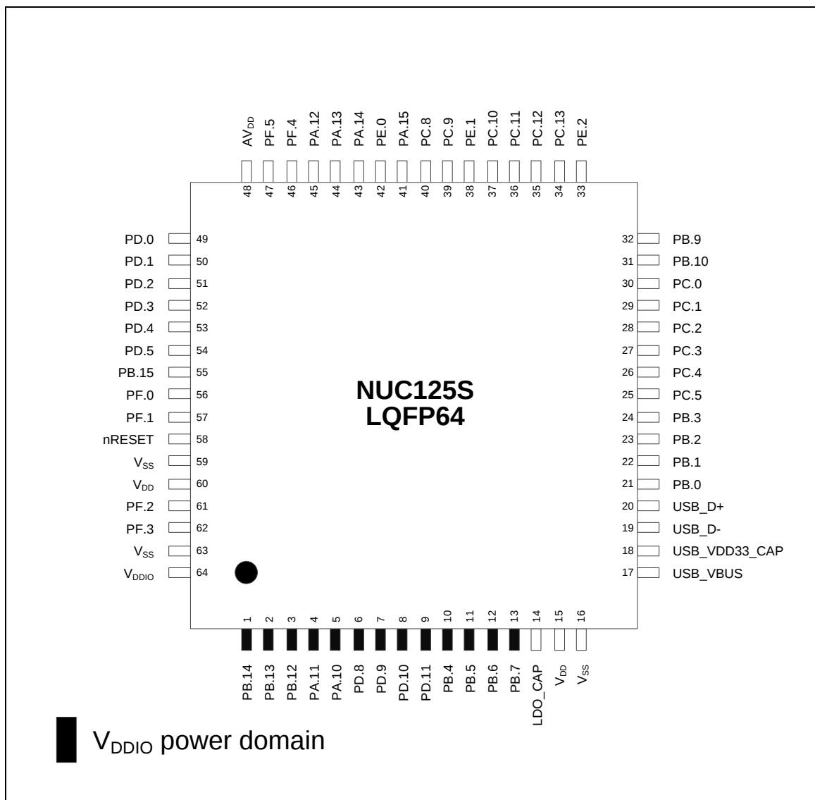
Figure 4.2-11 NuMicro® NUC125 LQFP 64-Pin Diagram
