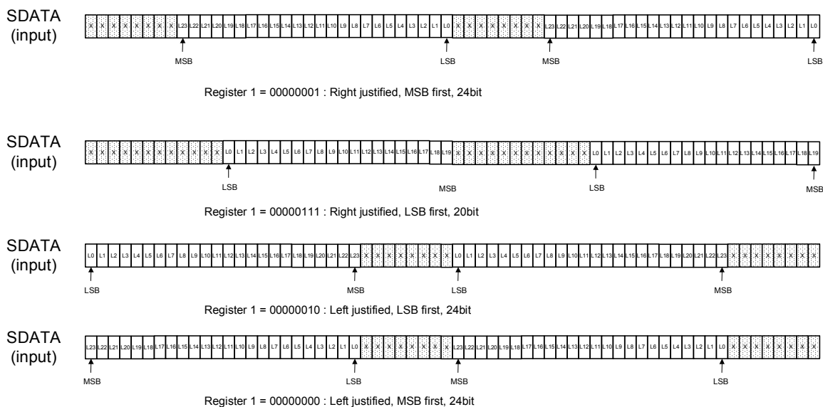
Figure 11 General serial audio data formats
