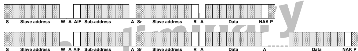
Figure 6 Read Mode Sequence
