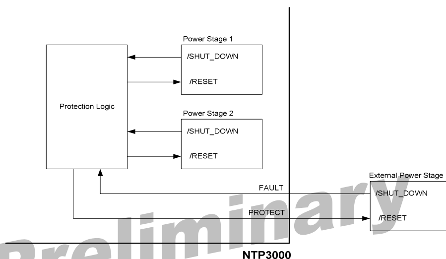
Figure 8 Protection Logic connection Diagram
