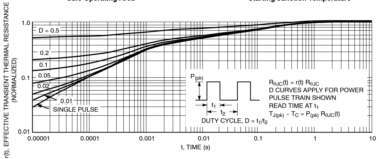
Figure 13. Thermal Response
