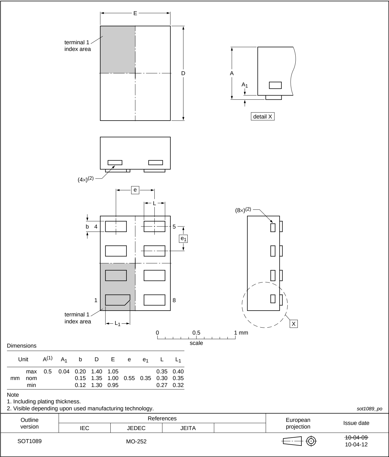
Fig 15. Package outline SOT1089 (XSON8) NTB0102 All information provided in this document is subject to legal disclaimers. © NXP B.V. 2013. All rights reserved. Product data sheet Rev. 4 — 23 January 2013 21 of 26
