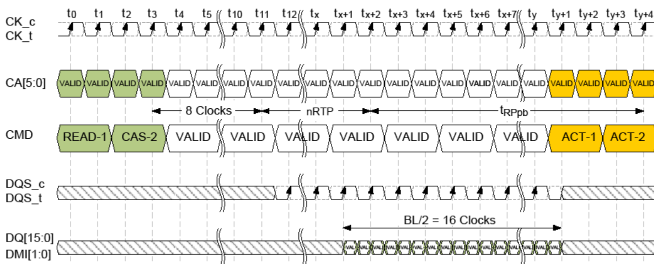
Burst READ with Auto-PRECHARGE (Shown with BL32, 2tCK pre-amble)
