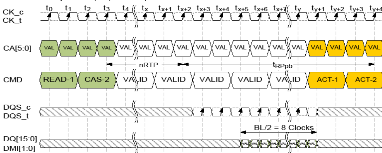
Burst READ with Auto-PRECHARGE (Shown with BL16, 2tCK pre-amble)
