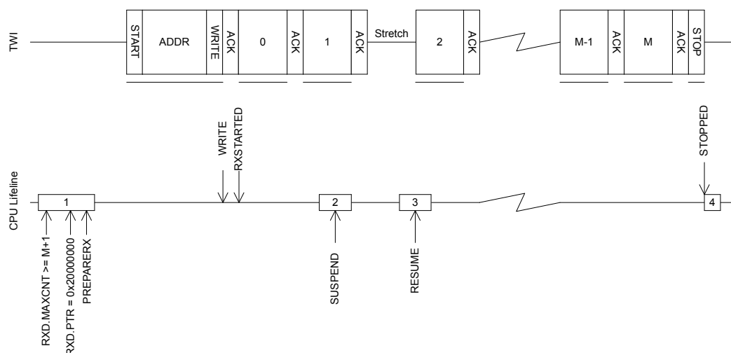
Figure 100: The TWI slave responding to a write command
