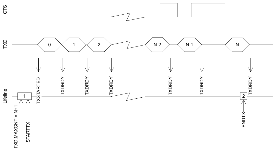
Figure 104: UARTE transmission
