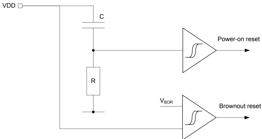
Figure 9: Power supply supervisor
