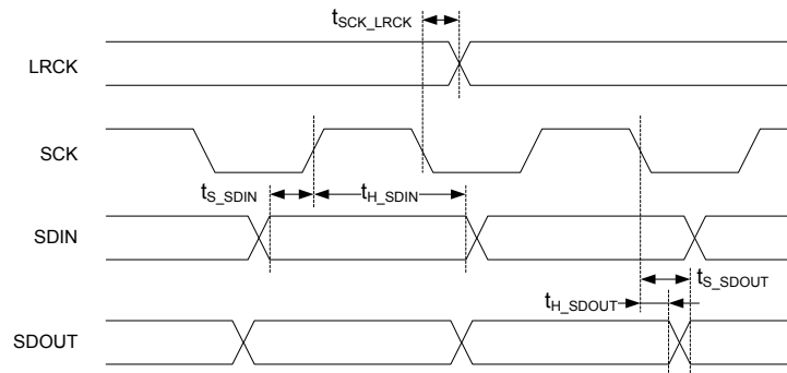
Figure 32: I2S timing diagram
