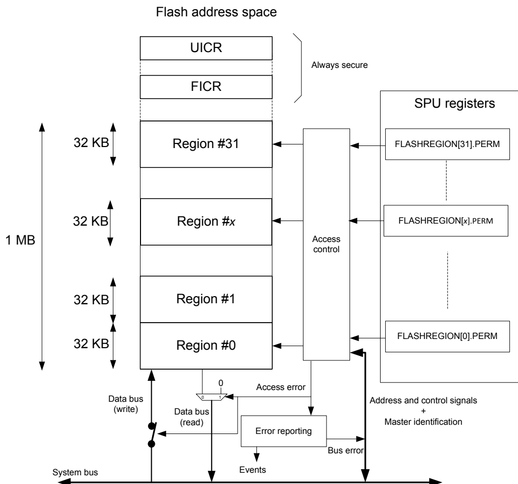
Figure 79: Region definition in the flash memory space
