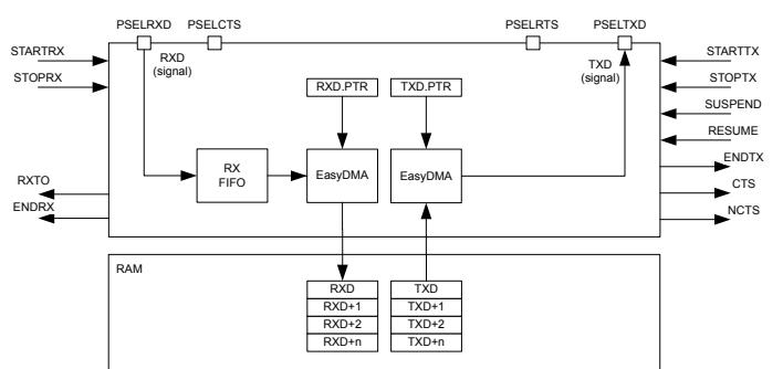
Figure 103: UARTE configuration
