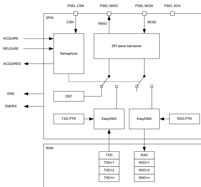
Figure 73: SPI slave
