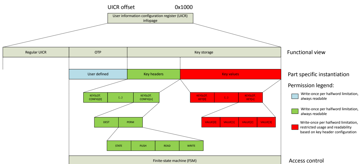
Figure 33: Memory map overview
