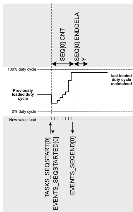
Figure 46: Single shot ( LOOP.CNT=0 )
