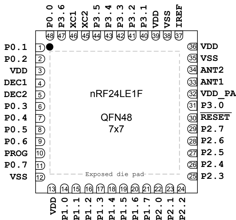
Figure 4. nRF24LE1F pin assignment (top view) for a QFN48 7×7 mm package
