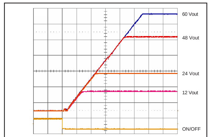
Figure 8: Turn-on transient at full load (20 ms/div). Ch 1: ON/OFF input (5 V/div) Ch 2-4: Vout (10 V/div)(100mV/div).
