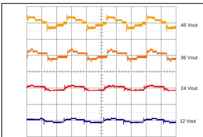
Figure 11: Output voltage response for 12 V, 24 V, 36 V, and 48 Vout to step-change in load current (50-75-50% of I_{out} max; di/dt=0.1A/\mu s ). Load cap: 100 \mu F, 100m \Omega ESR tant, Vout (2 V/div).
