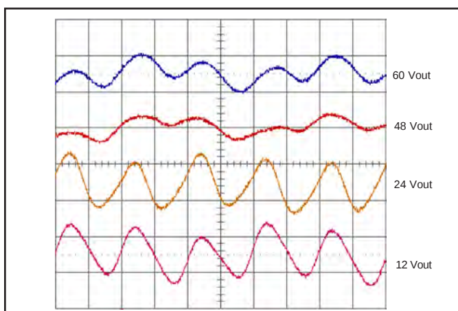
Figure 5: Input Terminal Ripple Voltage at 24 V input voltage and rated load current (500 mA/div). Bandwidth: 20 MHz. See Figure 4.
