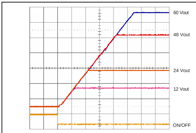
Figure 7: Turn-on transient at zero load (20 ms/div). Ch 1: ON/OFF input (5 V/div) Ch 2-4: Vout (10 V/div)
