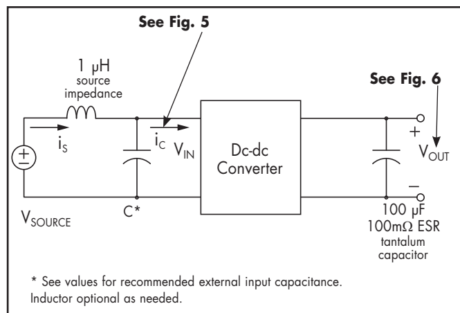
Figure 4: Test set-up diagram showing measurement points for Input Terminal Ripple Voltage (Figure 5), and Output Voltage Ripple (Figure 6).
