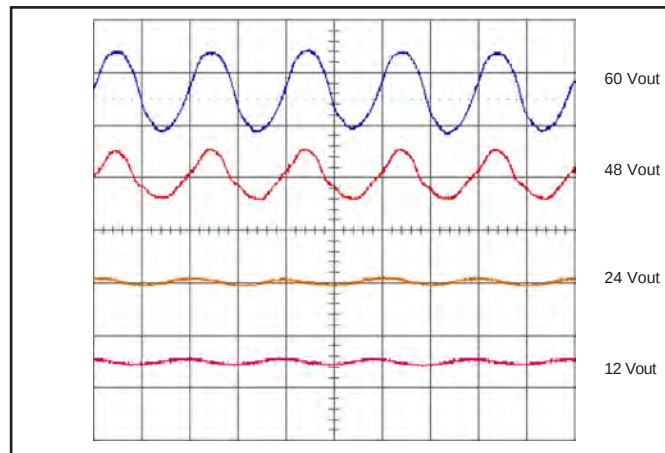
Figure 6: Output Voltage Ripple at 36 V input voltage and rated load current (100 mV/div). Zero load capacitance. Bandwidth: 20 MHz. See Figure 4.
