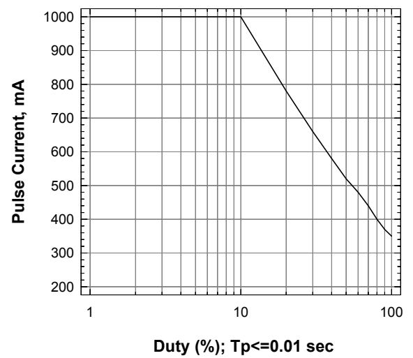
Maximum Permissible Pulse Current, T_a=25^\circ\text{C}
