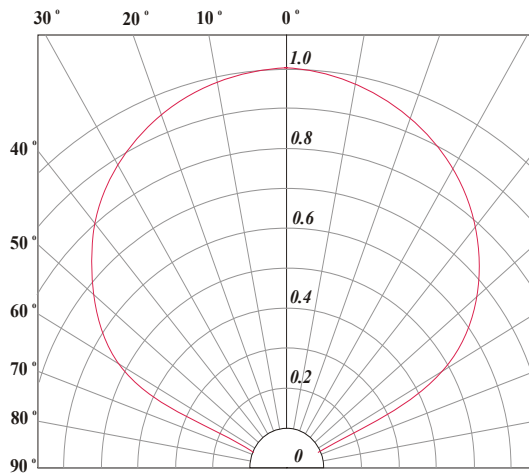
Radiation Pattern
