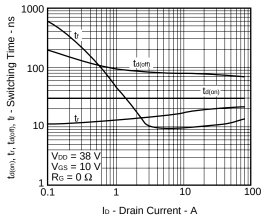
Figure15. SWITCHING CHARACTERISTICS
