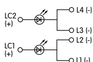
Amber LED
