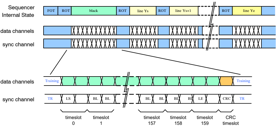
Figure 33. P1&P3–SN/SE/FN: Time Line for Black Line Readout
