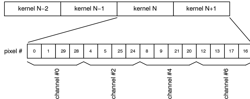
Figure 46. P1,P3–SE: Data Output Order for 4 LVDS Output Channels in Subsampling Mode on a Color Sensor
