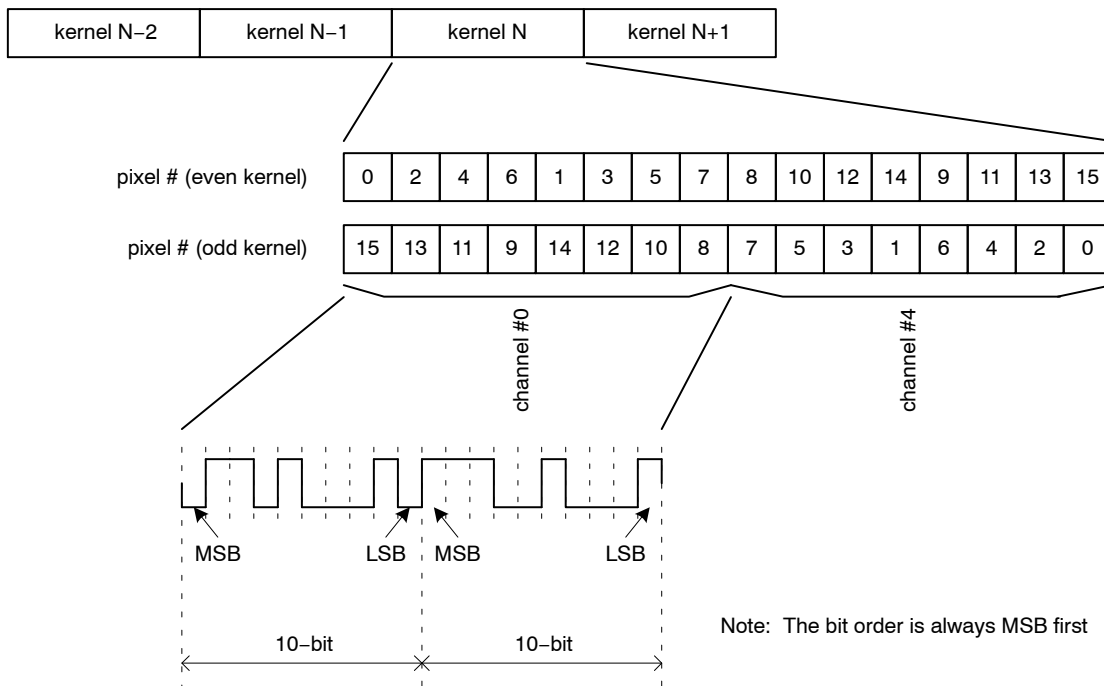
Figure 39. P1,P3-SN/SE/FN: 2 LVDS Data Output Order when Subsampling is Disabled
