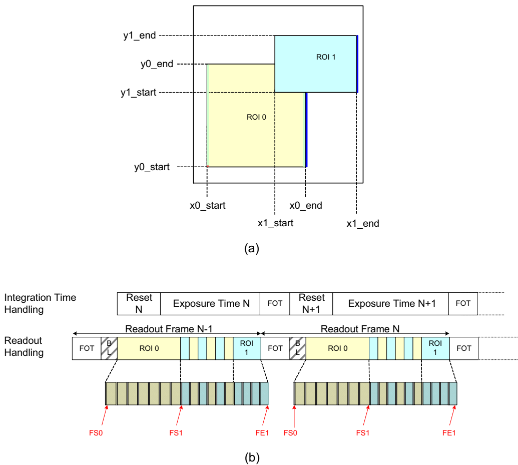
Figure 32. P1&P3–SN/SE/FN: Frame Sync Codes
