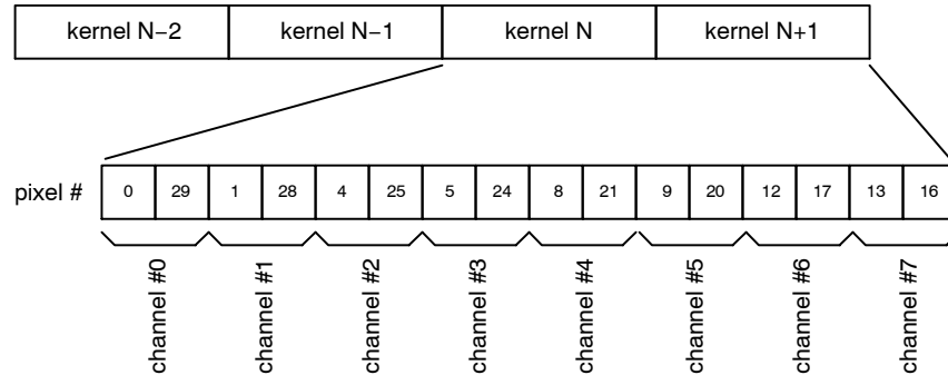
Figure 45. P1–SE: Data Output Order for 8 LVDS Output Channels in Subsampling Mode on a Color Sensor
