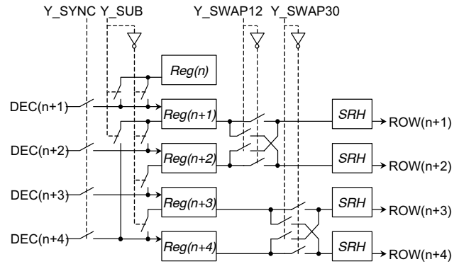
Figure 10. Row Structure
