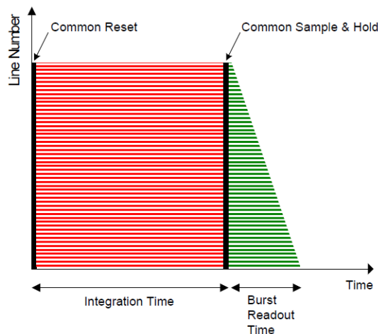
Figure 17. Global Shutter Operation
