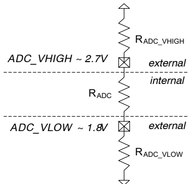
Figure 14. Internal and External ADC Connections
