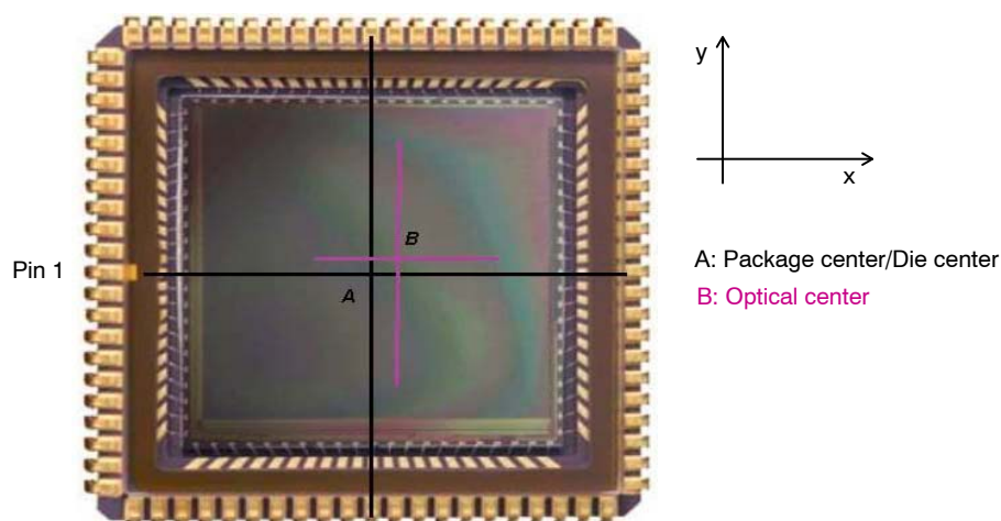
Figure 3. Die Placement
