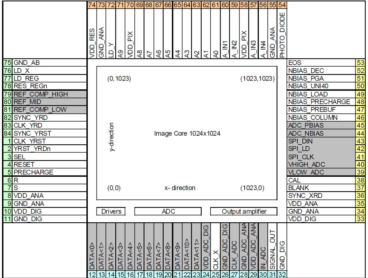
Figure 25. Pin Configuration
