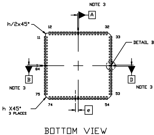
Figure 4. 84-Pin JLCC Package Diagram
