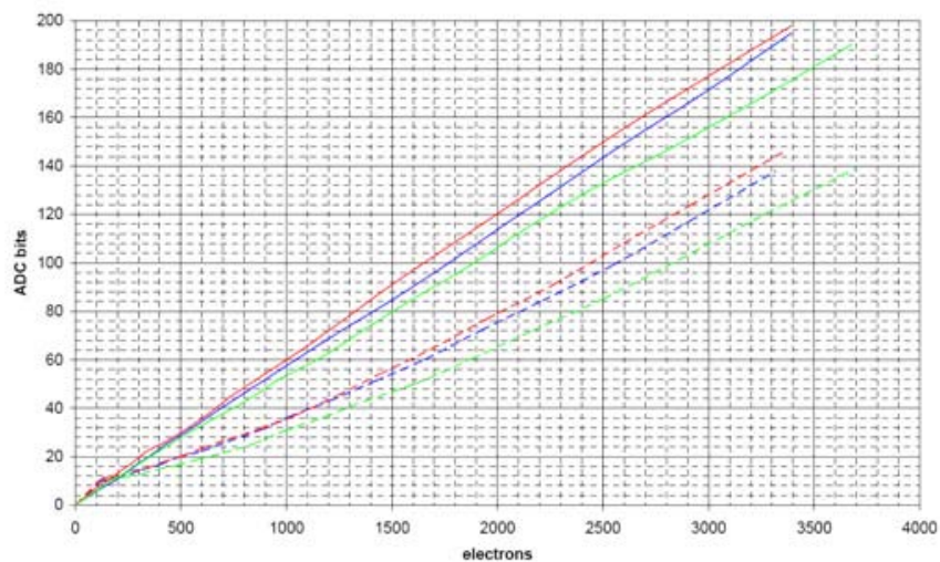
Figure 10. Pixel Response Curve < 4000\text{ e}^-
