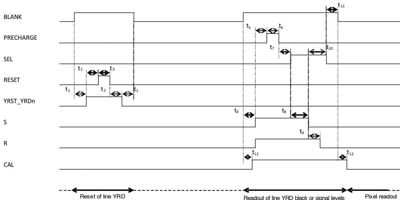
Figure 37. Non-destructive Readout Timing Diagram
