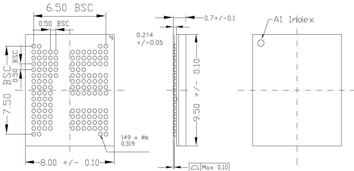
BOTTOM VIEW
