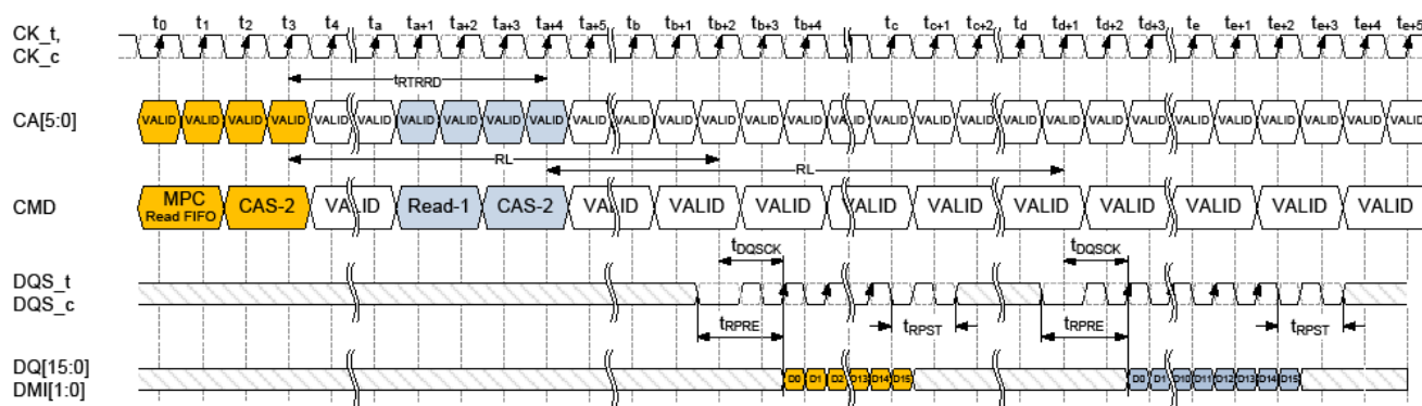
MPC [RD FIFO] Operation : tRPST=toggling, tRPST=1.5nCK
