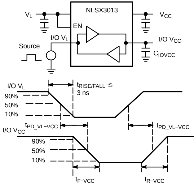
Figure 4. Driving I/O V_L Test Circuit and Timing
