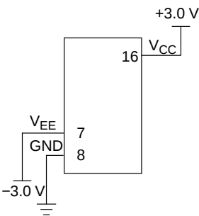
Figure 25. Dual Supply V_{CC} = 3.0\text{ V} , V_{EE} = -3.0\text{ V}
