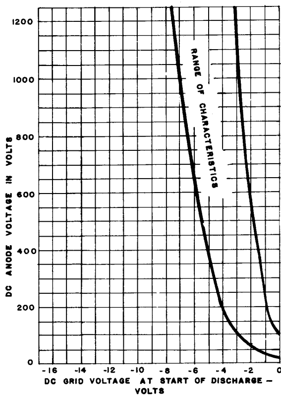
GRID CHARACTERISTIC
