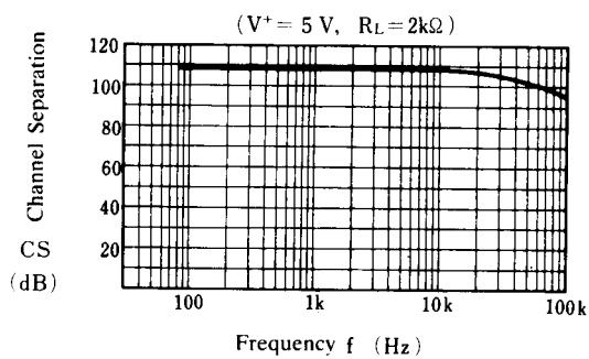
Channel Separation vs. Frequency
