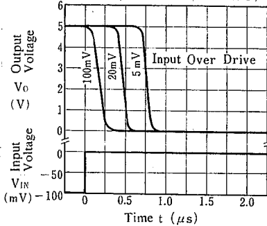
Response Time for Various Input Over Drives ( V^+ = 5\text{ V} , R_L = 5.1\text{ k}\Omega , T_a = 25^\circ\text{C} )
