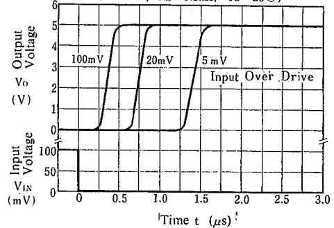
Response Time for Various Input Over Drives ( V^+ = 5\text{ V} , R_L = 5.1\text{ k}\Omega , T_a = 25^\circ\text{C} )
