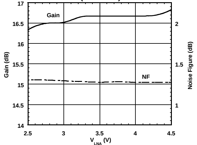
Gain, Noise Figure vs. V_{LNA} ( f=820\text{MHz} )
