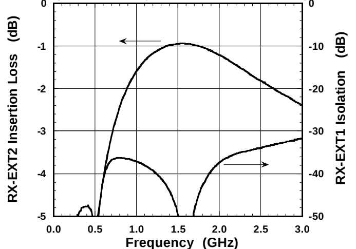
RX-EXT1 Isolation
