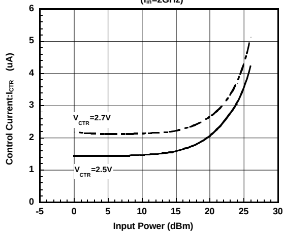
(PC-P1) Control Current vs. Input Power
