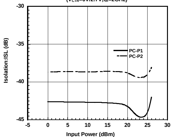
Isolation vs. Input Power
