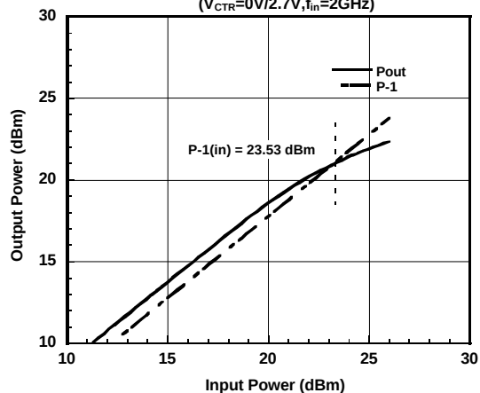
(PC-P1) Output Power vs. Input Power
