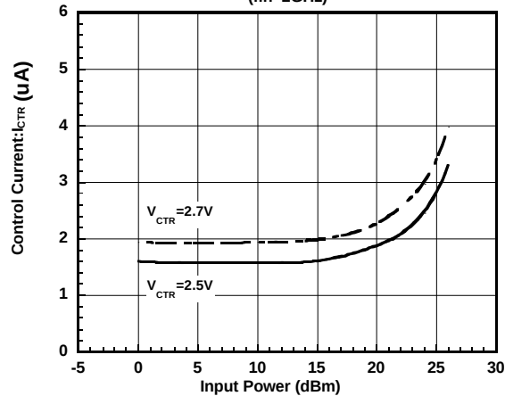
(PC-P2) Control Current vs. Input Power
