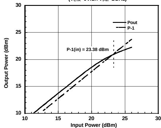
(PC-P2) Output Power vs. Input Power
