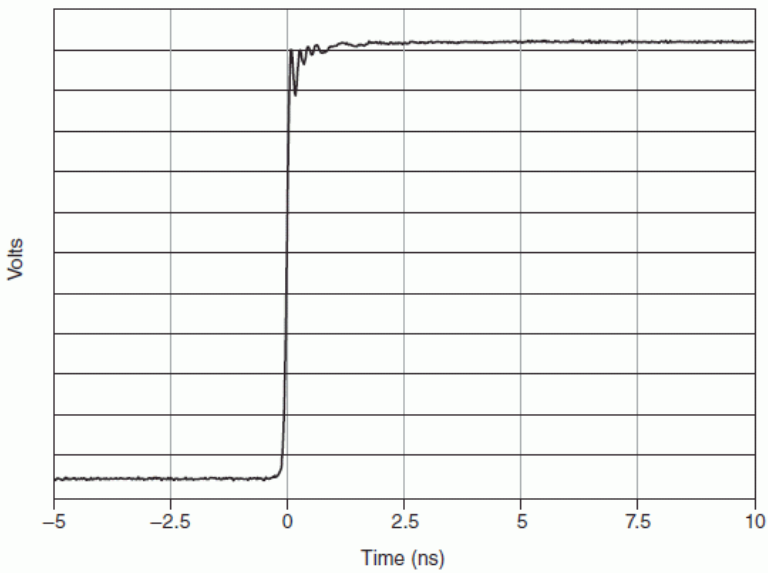
NI 5185 Frequency Response (Characteristic)
