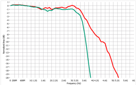
Figure 8. Typical Frequency Response Performance From Using the NI PXIe-5185 or PXIe-5186 with the Tektronix P6330 Probe in a Solder-In Configuration
