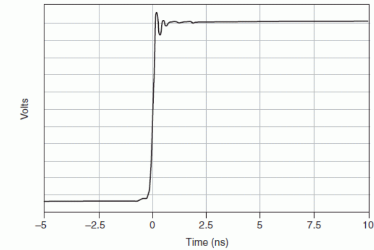
NI 5186 Step Response, 50 Ω, -0.25 V Programmable Offset (Characteristic)
