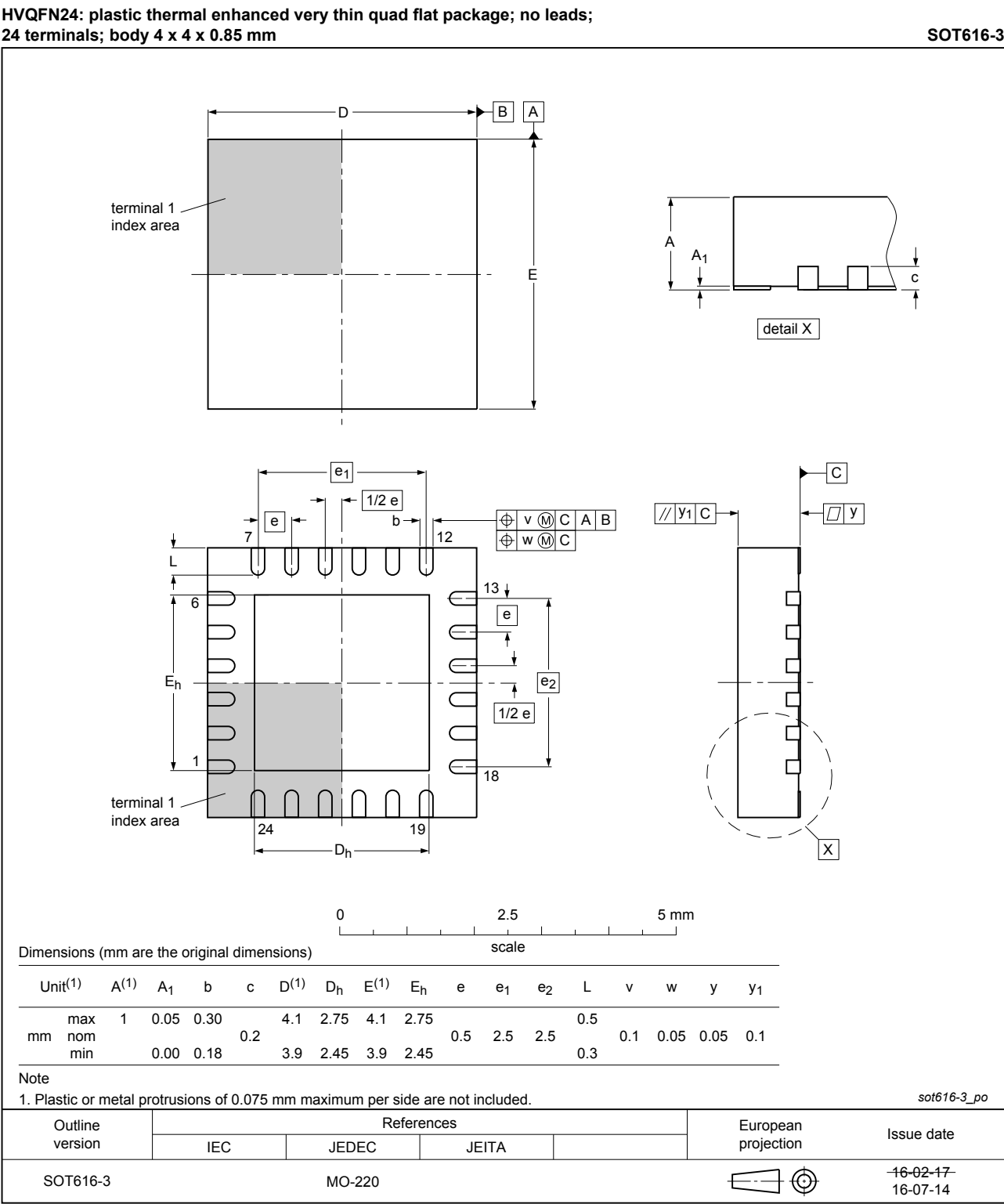
Figure 19. HVQFN24 package outline
