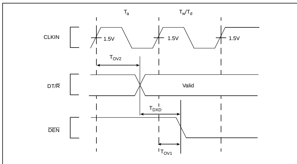
Figure 27. \overline{DT/R} and \overline{DEN} Timings Waveform
