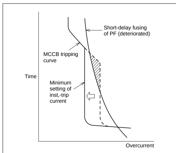
Fig. 6.23 Coordinated PF and MCCB Characteristics
