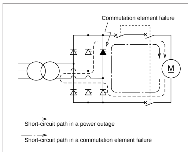
Fig. 7.18 Ward-Leonard Thyristor Protection
