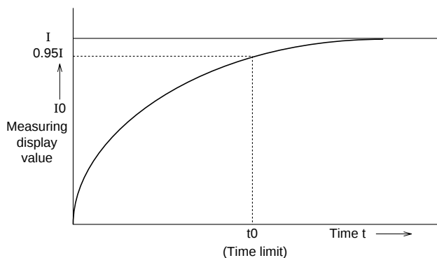
Fig.7.26 Demand Characteristics
