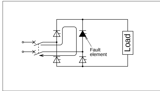
Fig. 7.14 Fault-Current Flow
