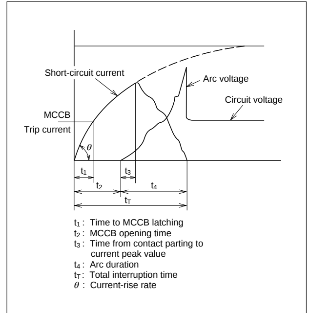
Fig. 7.16 Thyristor Short-Circuit Interruption
