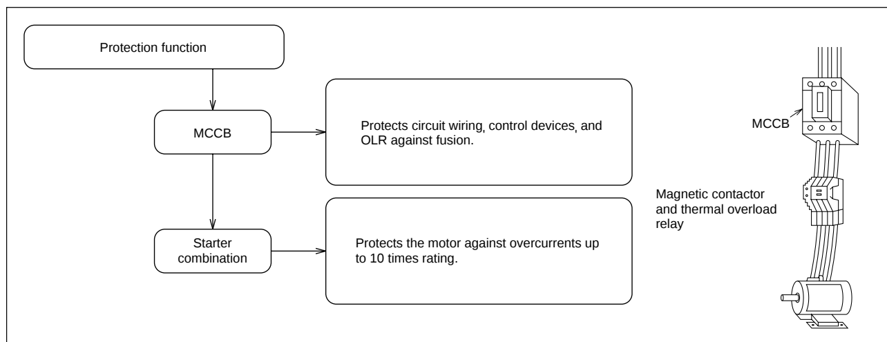
Fig. 6.18 Protective Coordination; MCCBs and Motor Starters
