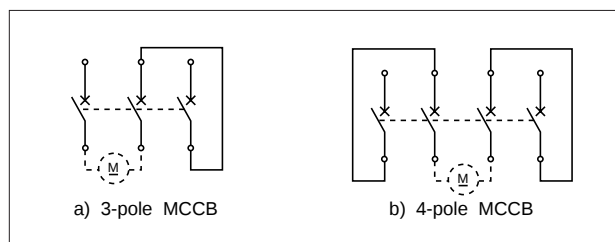
Fig. 7.20 Series Connection of MCCB Poles
