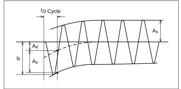
Fig. 9.3 Short-Circuit Current
