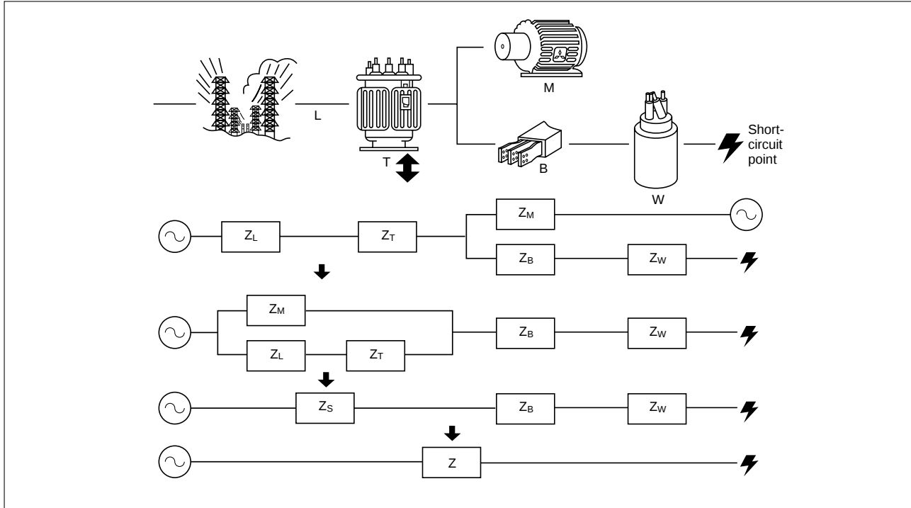
Fig. 9.2 3-Phase Equivalent Circuits
