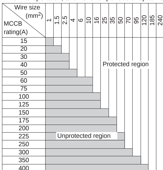
Fig. 6.15 MCCBs and Wiring Sizes
