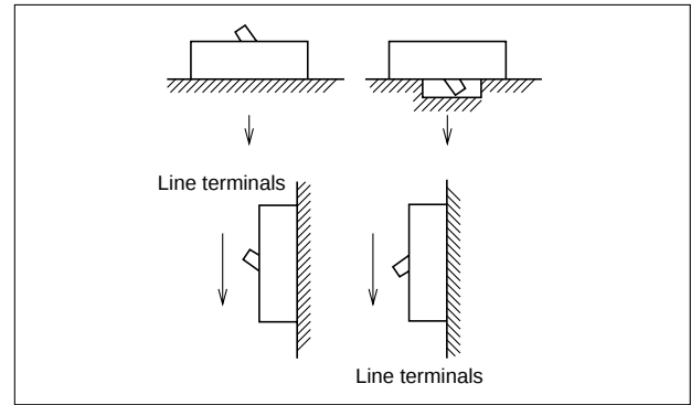
Fig. 8.2 Drop-Test Attitudes
