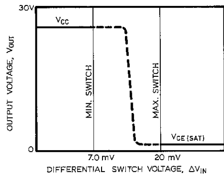
TYPICAL SWITCH CHARACTERISTICS
