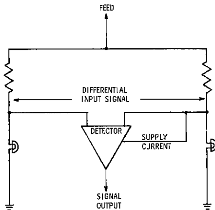
BASIC BRIDGE MONITORING SYSTEM
