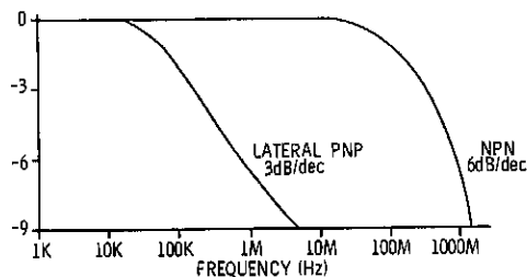
Figure 5 FREQUENCY RESPONSE
