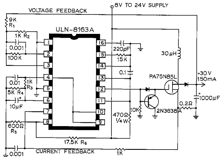
FIGURE 1 BOOST CONVERTER
