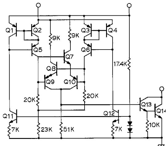
SIMPLIFIED SCHEMATIC (One of 4 differential sense amplifiers)
