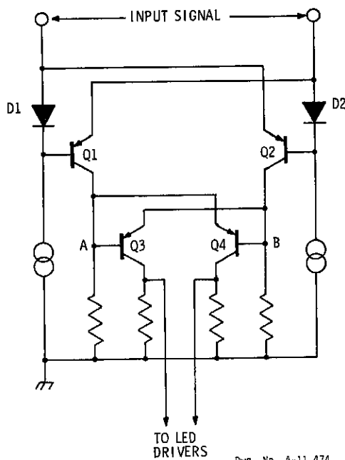
Figure 4 SIMPLIFIED DETECTOR
