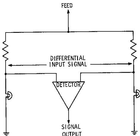
Figure 3 BRIDGE MONITORING SYSTEM
