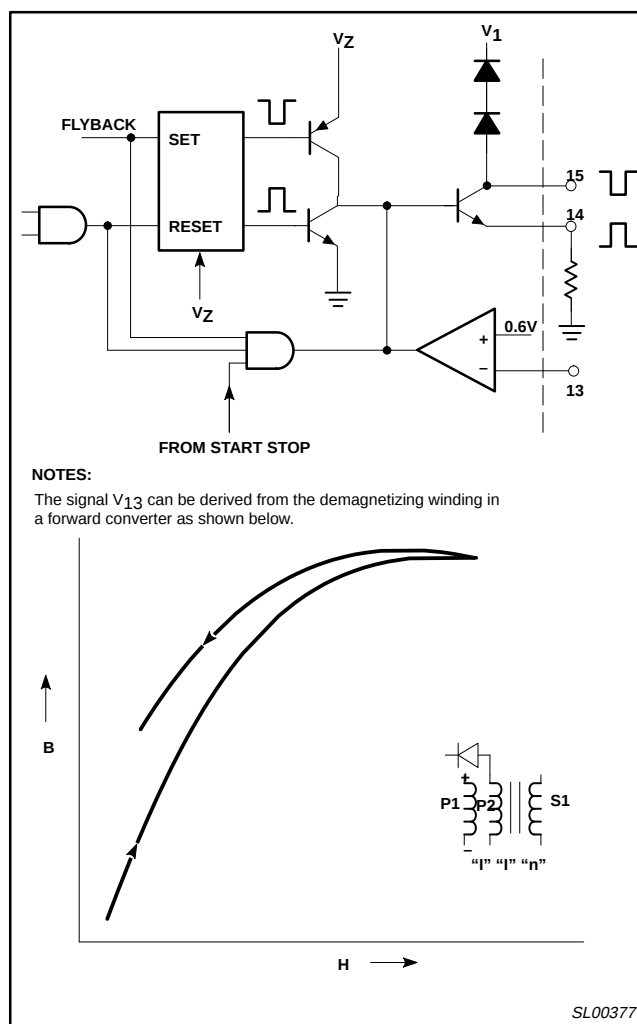
Figure 18. Output Stage
