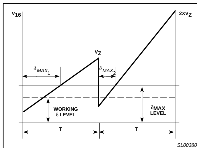
Figure 21. Feed-Forward Circuitry
