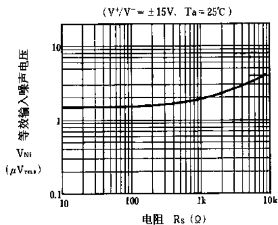
等效输入噪声电压与电阻 R_s
