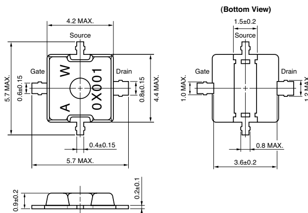
PACKAGE OUTLINE 79A
