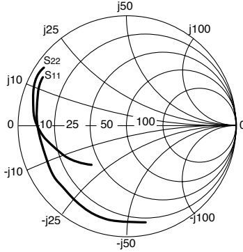
Coordinates in Ohms Frequency in GHz V_D = 3.5\text{ V} , I_D = 200\text{ mA}
