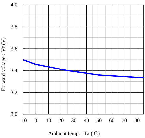
Ambient temp. vs. Forward voltage
