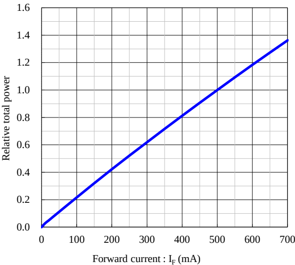
Forward current vs. Relative total power
