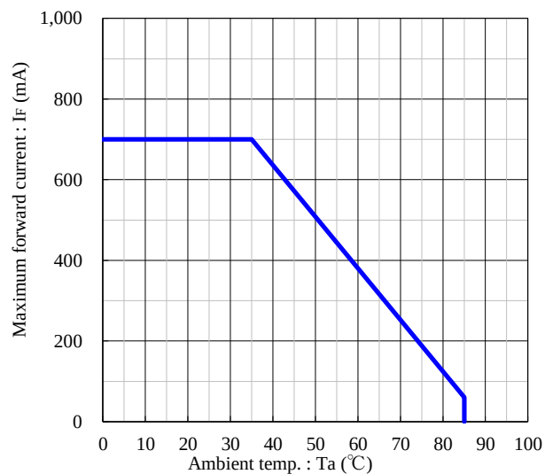
Ambient temp. vs. Maximum forward current
