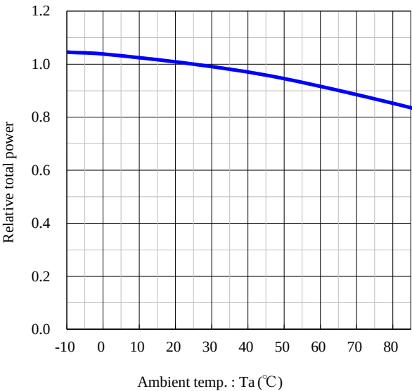
Ambient temp. vs. Relative total power
