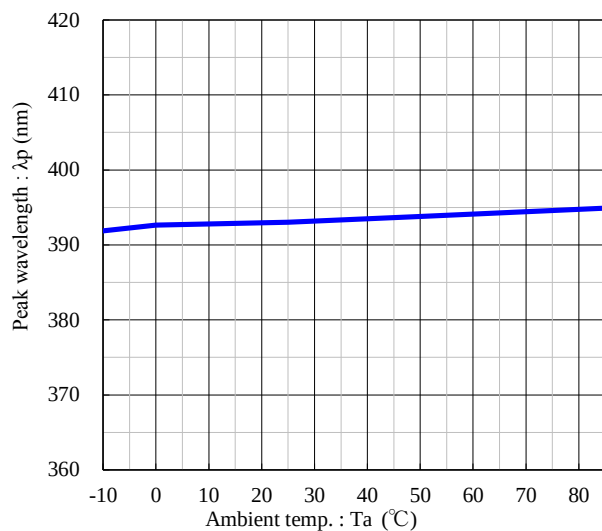
Ambient temp. vs. Peak wavelength
